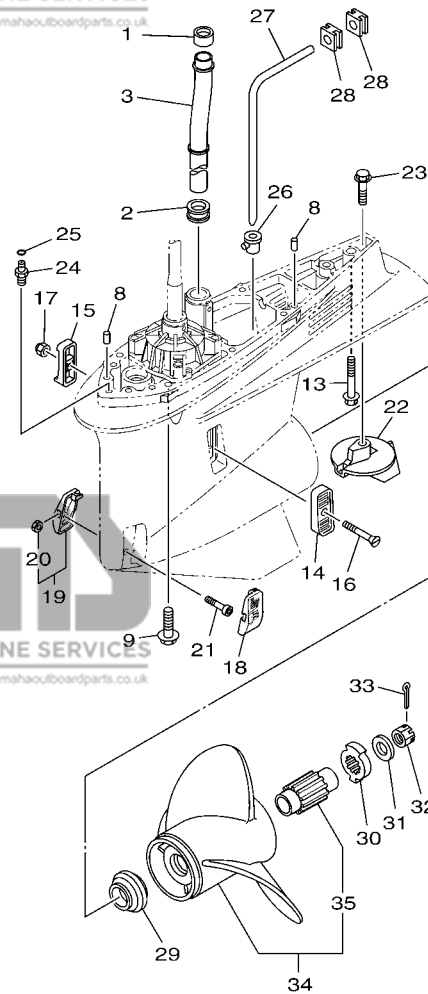
NORMAL PROPELLER
