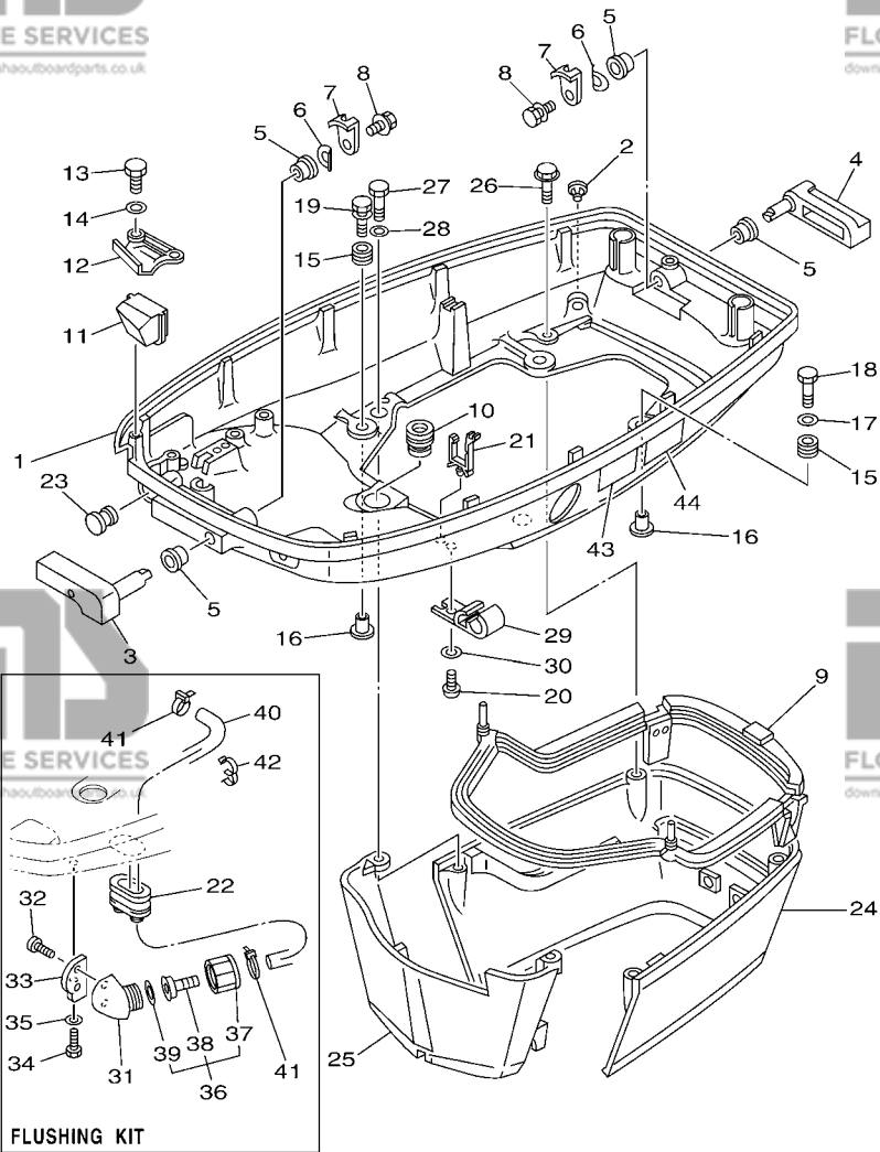
FLUSHING KIT 6H1G300-M120
