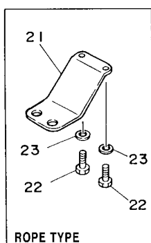
ROPE TYPE
