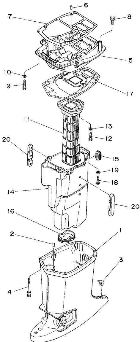
6H36100-F190
