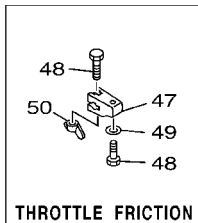
THROTTLE FRICTION
