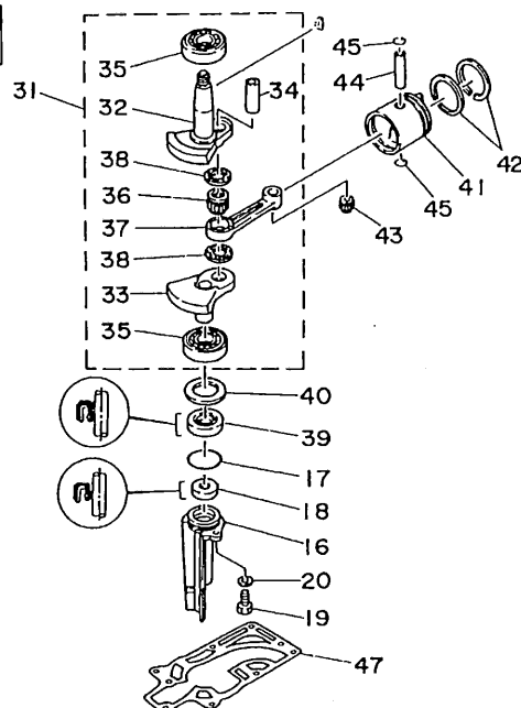
CRANK CYLINDER ASSY
