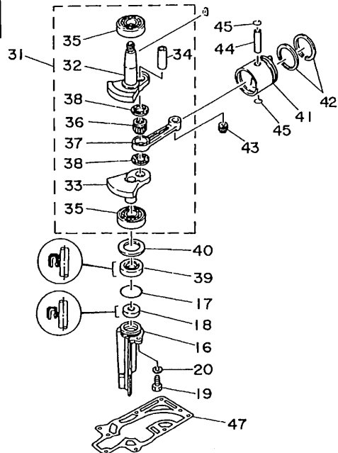
CRANK CYLINDER ASSY
