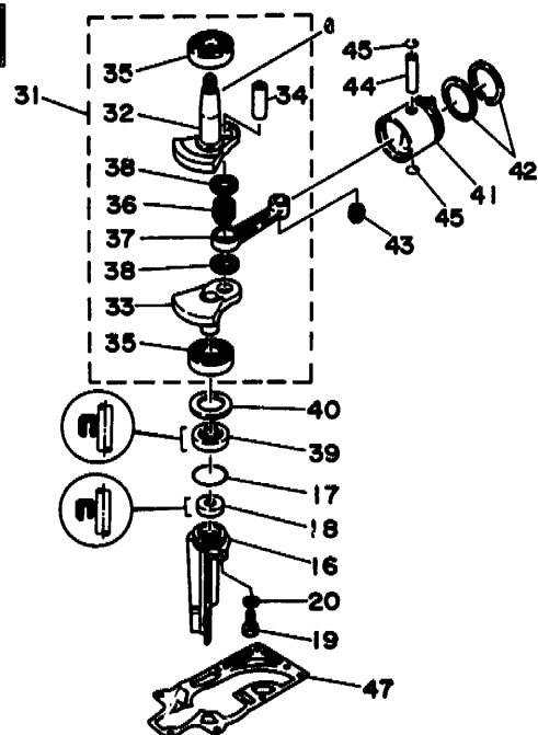
CYLINDER BLOCK ASSY
