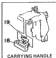
CARRYING HANDLE
