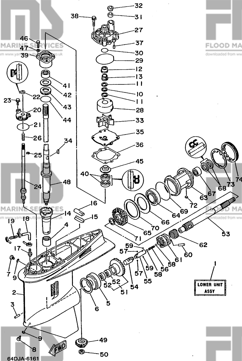
FIG. 17 LOWER CASING. DRIVE 1
