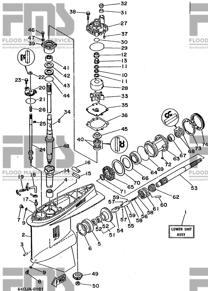
FIG. 17 LOWER CASING. DRIVE 1
