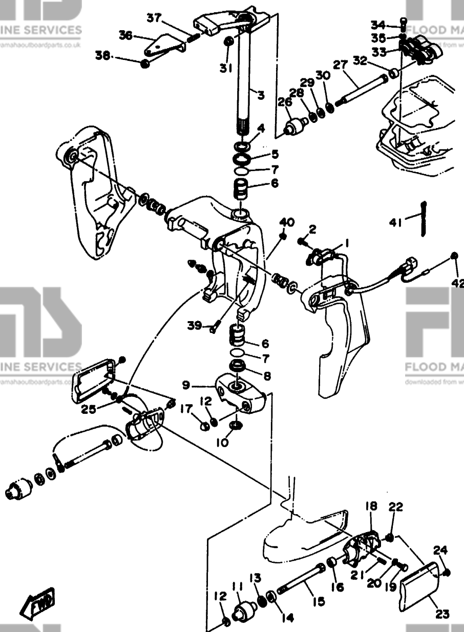
FIG. 11 BRACKET 2
