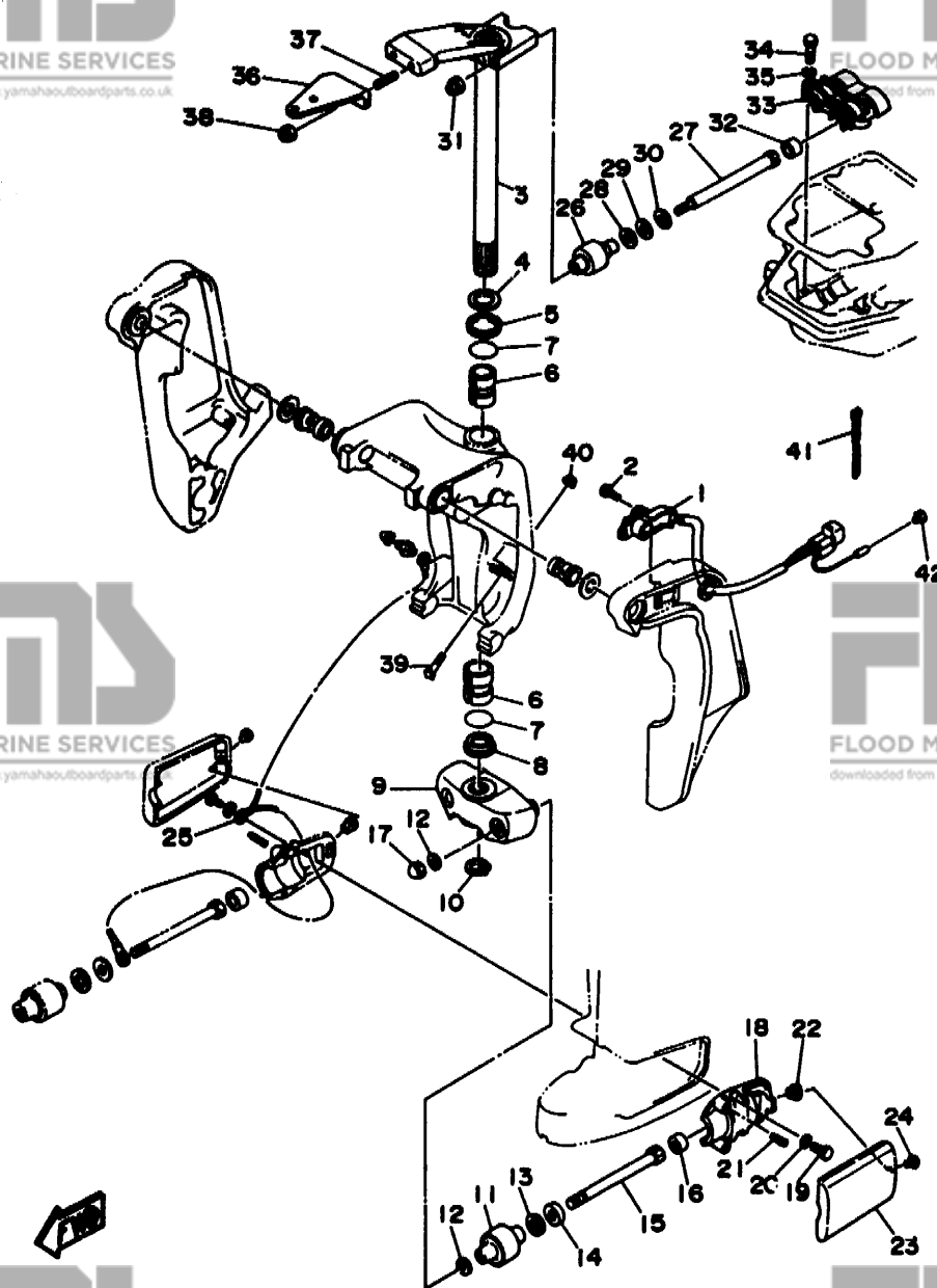
FIG. 11 BRACKET 2
