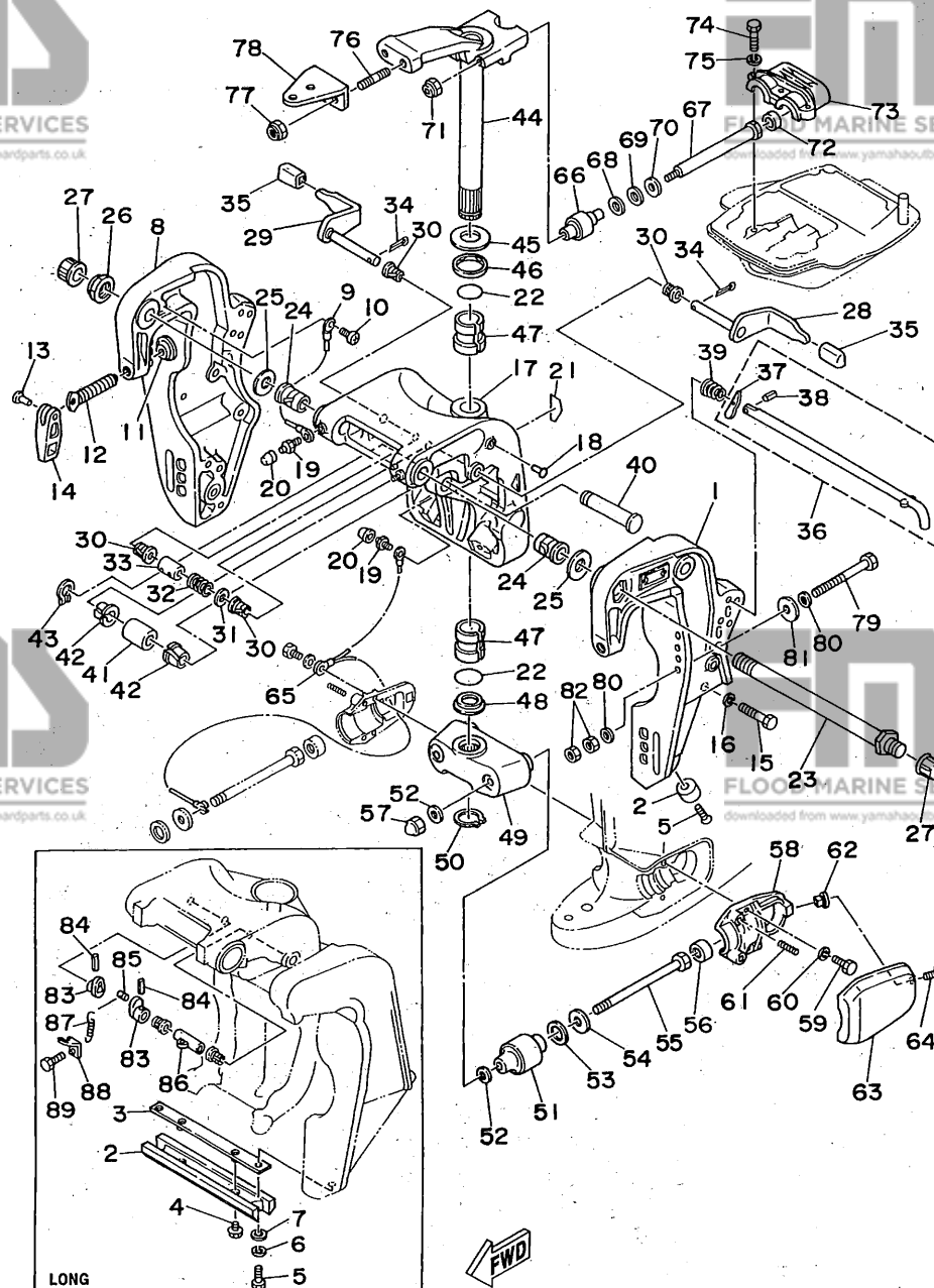
FIG. 6 BRACKET 1 (55BE/55BEM)
