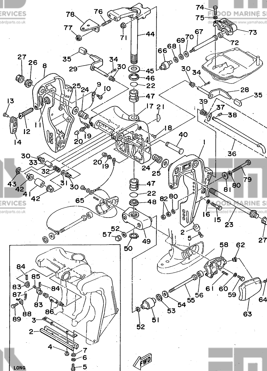
FIG. 6 BRACKET 1 (55BE/55BEM)
