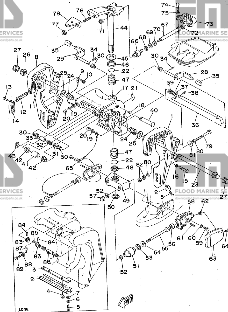
FIG. 6 BRACKET 1 (55BE/55BEM)
