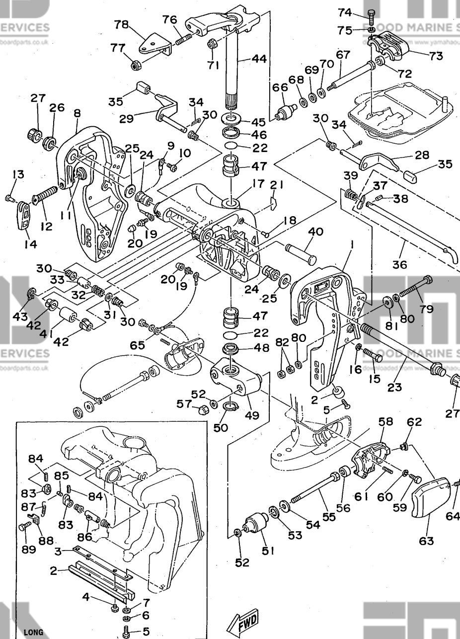
FIG. 6 BRACKET 1 (55BE/55BEM)
