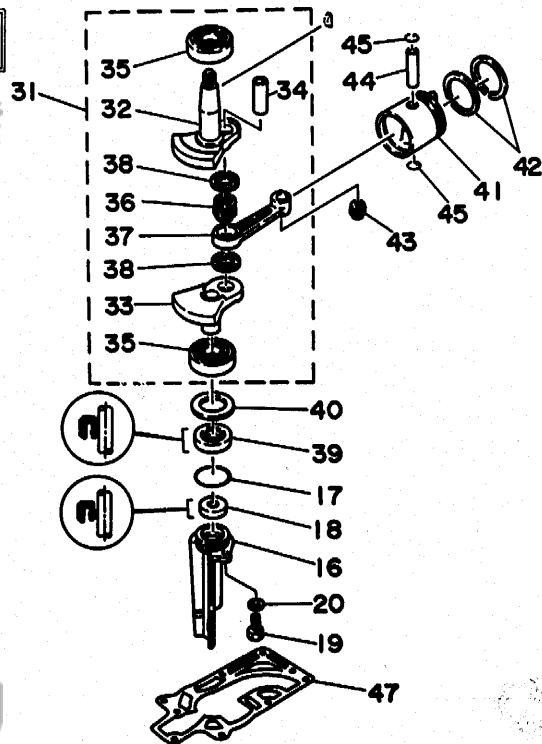
CRANK CYLINDER ASSY
