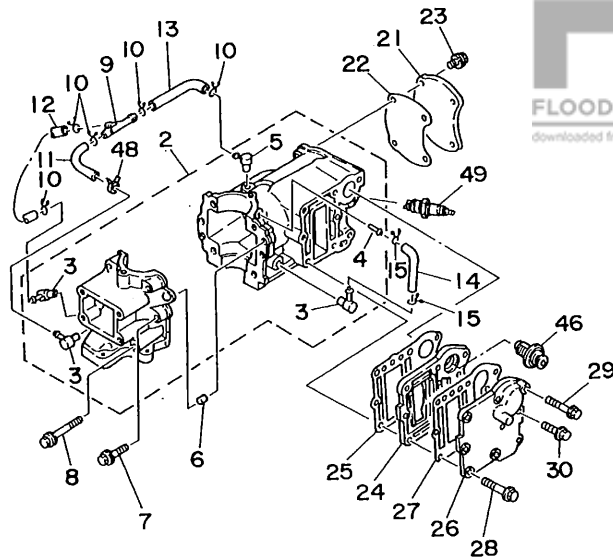
CRANK CYLINDER ASSY
