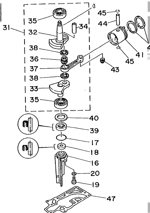
CRANK CYLINDER ASSY
