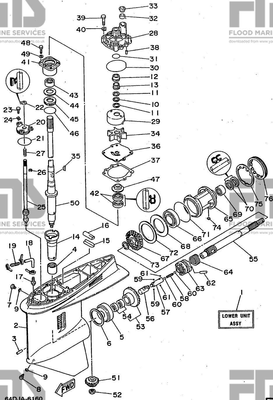
FIG. 20 LOWER CASING. DRIVE 1 (150/175/200)
