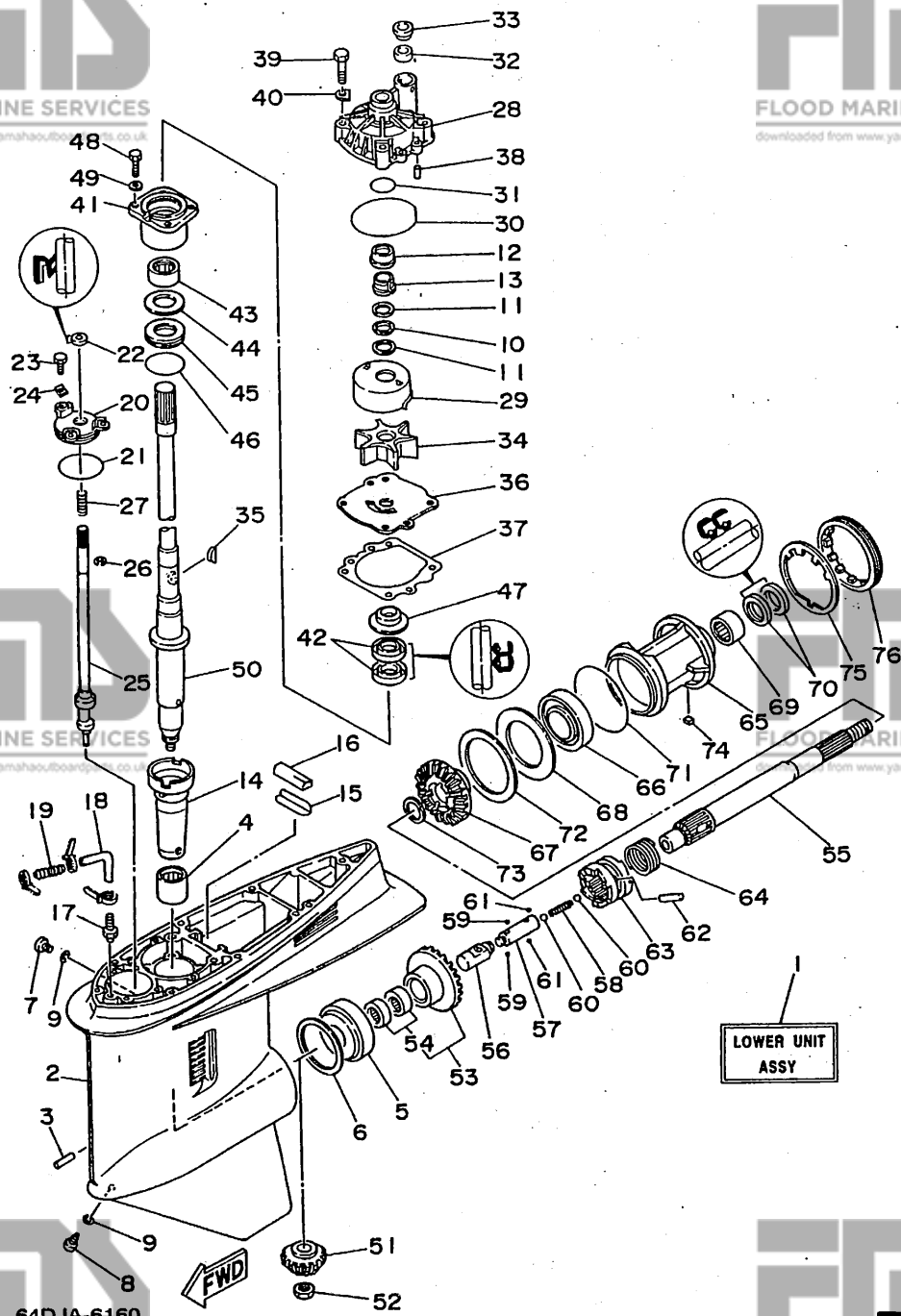
FIG. 20 LOWER CASING. DRIVE 1 (150/175/200)
