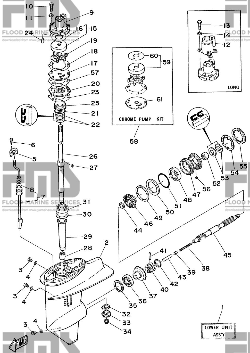
Fig. 12 LOWER & DRIVE 1
