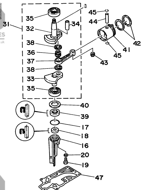
CRANK CYLINDER ASSY
