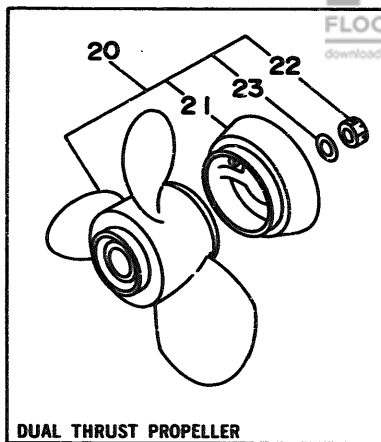
DUAL THRUST PROPELLER
