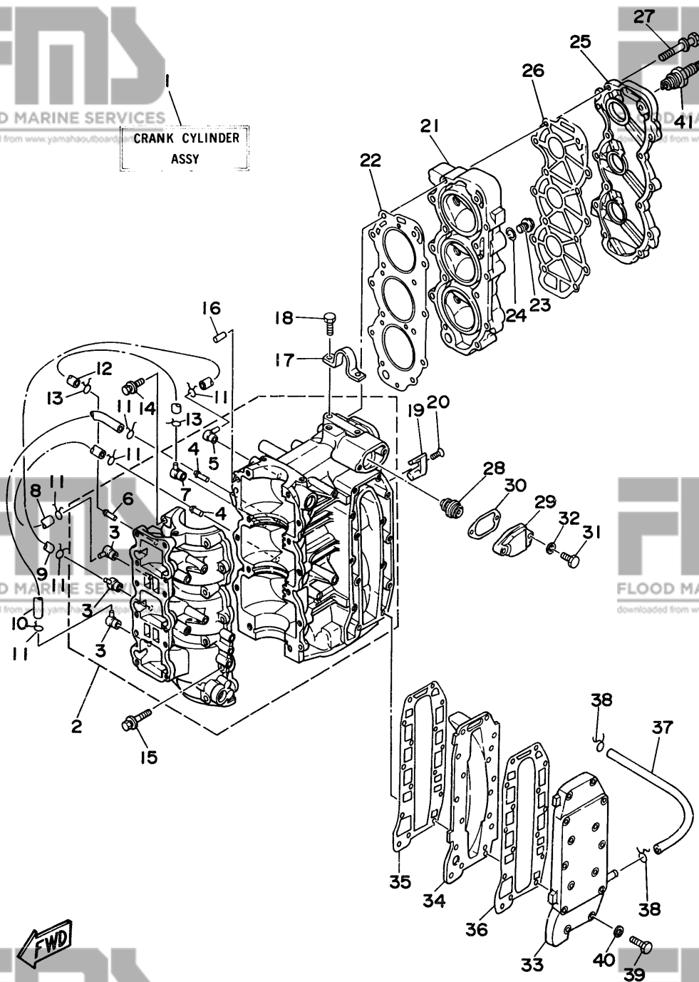
FIG. 1 CYLINDER. CRANKCASE
