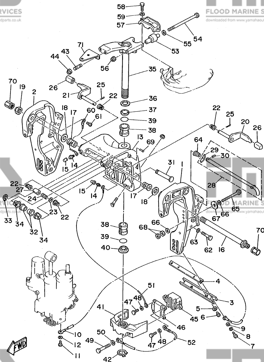
FIG. 15 BRACKET 4 (40HET0)
