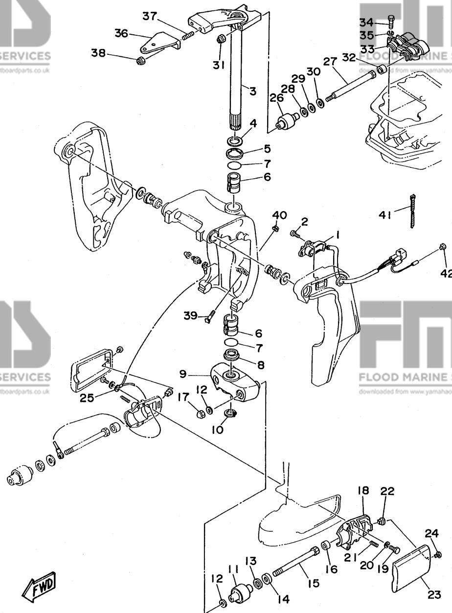
FIG. 11 BRACKET 2
