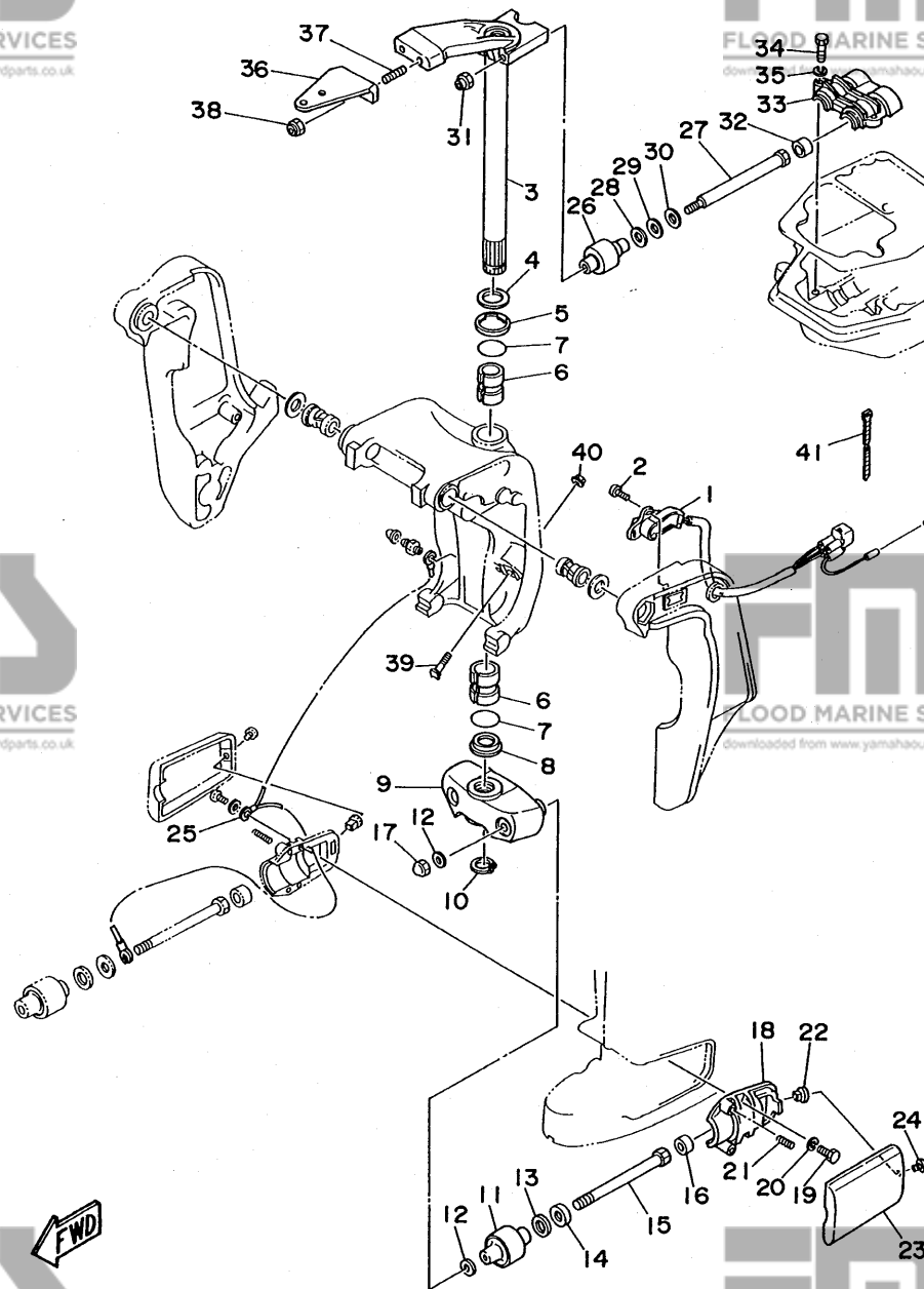
FIG. 11 BRACKET 2
