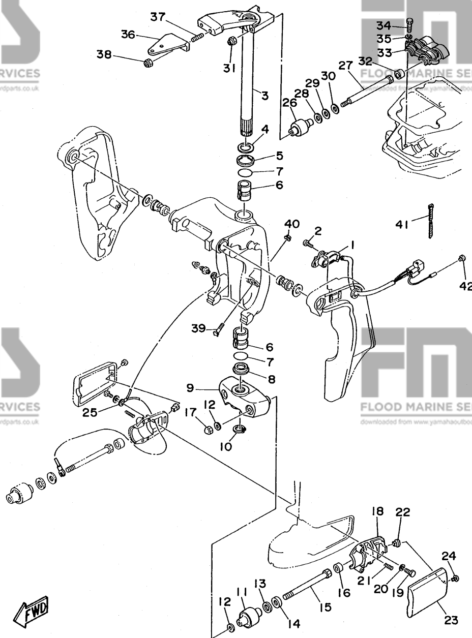
FIG. 11 BRACKET 2
