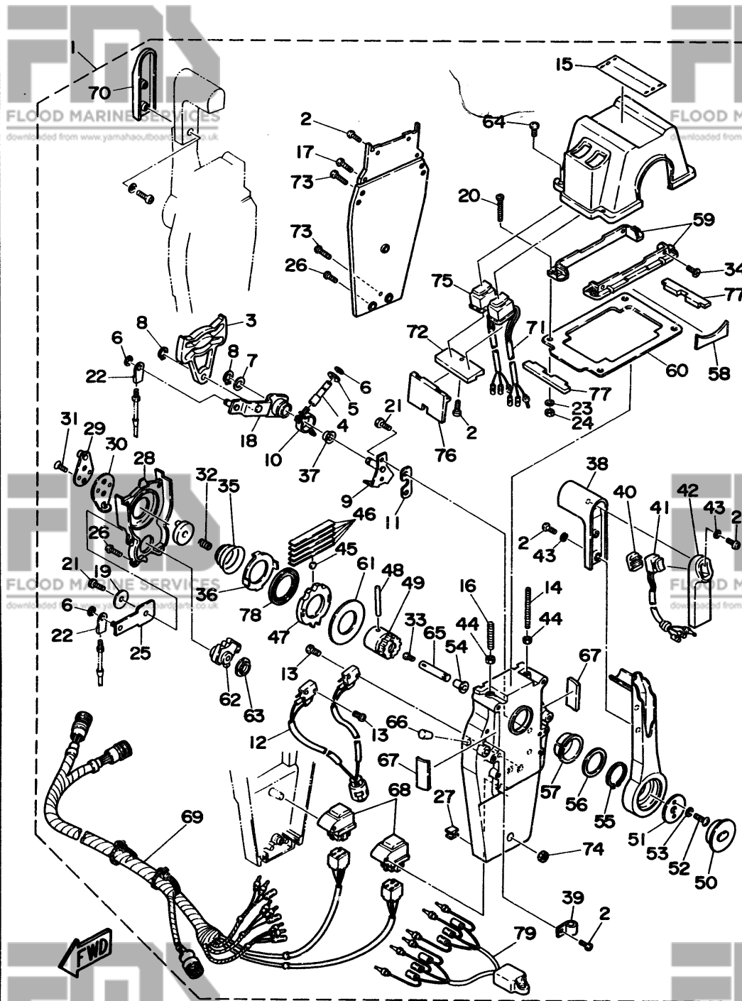
Fig. 26 REMOTE CONTROL ASSY 3
