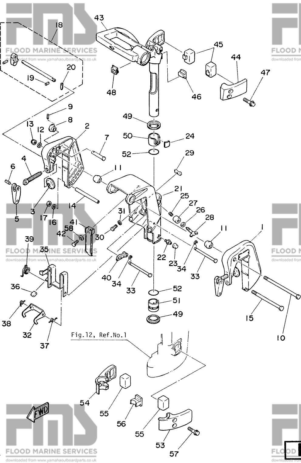
Fig. 9 BRACKET
