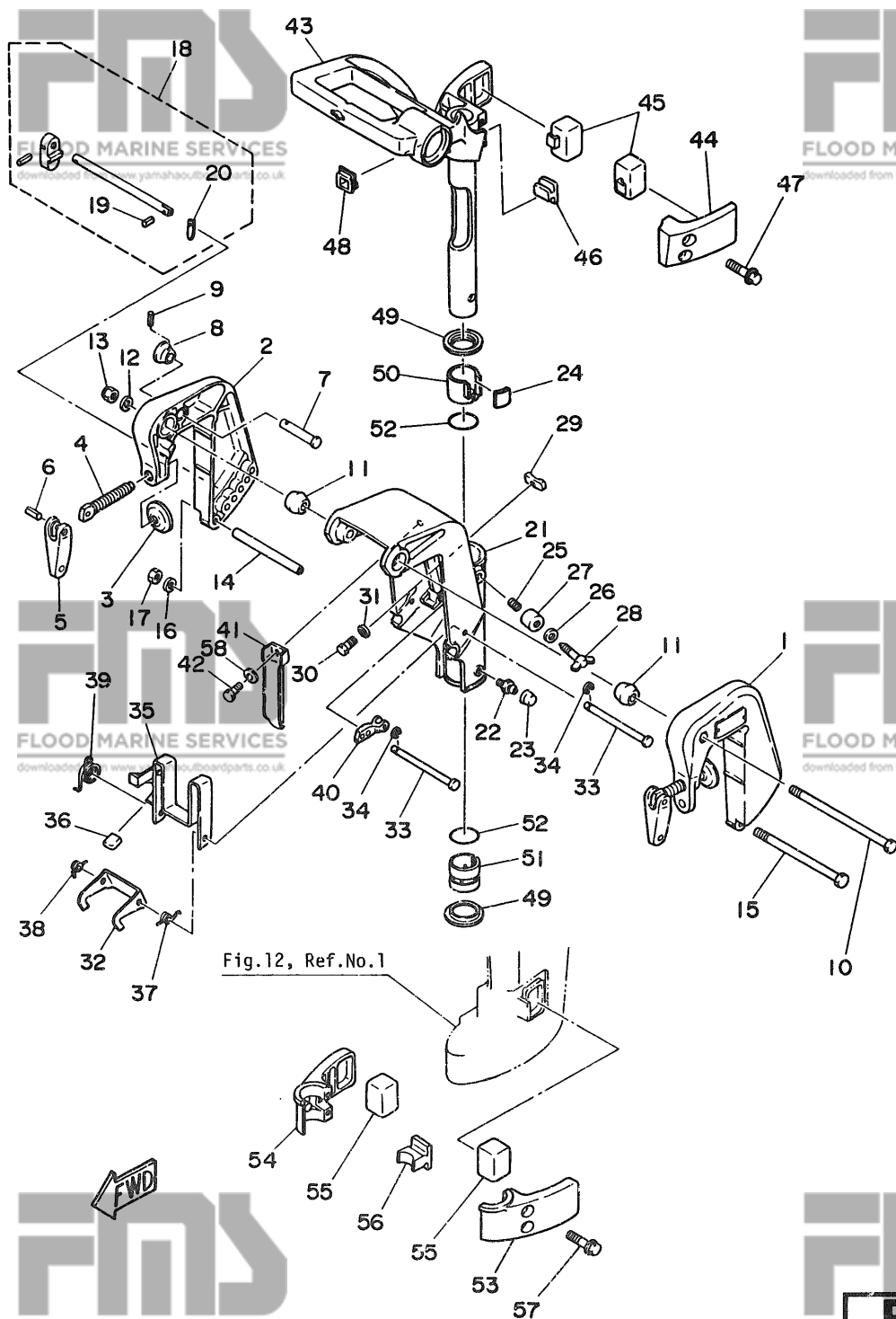
Fig. 9 BRACKET
