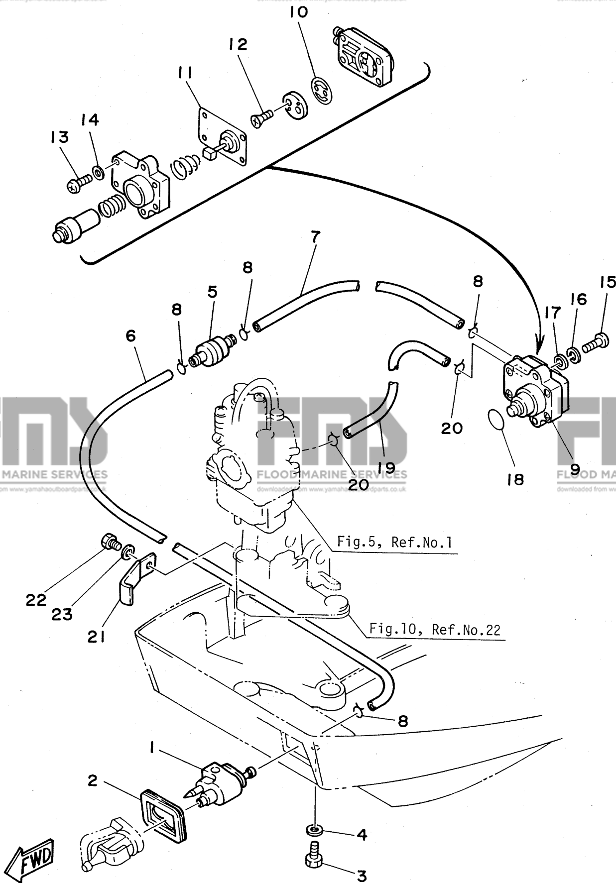
Fig. 8 FUEL
