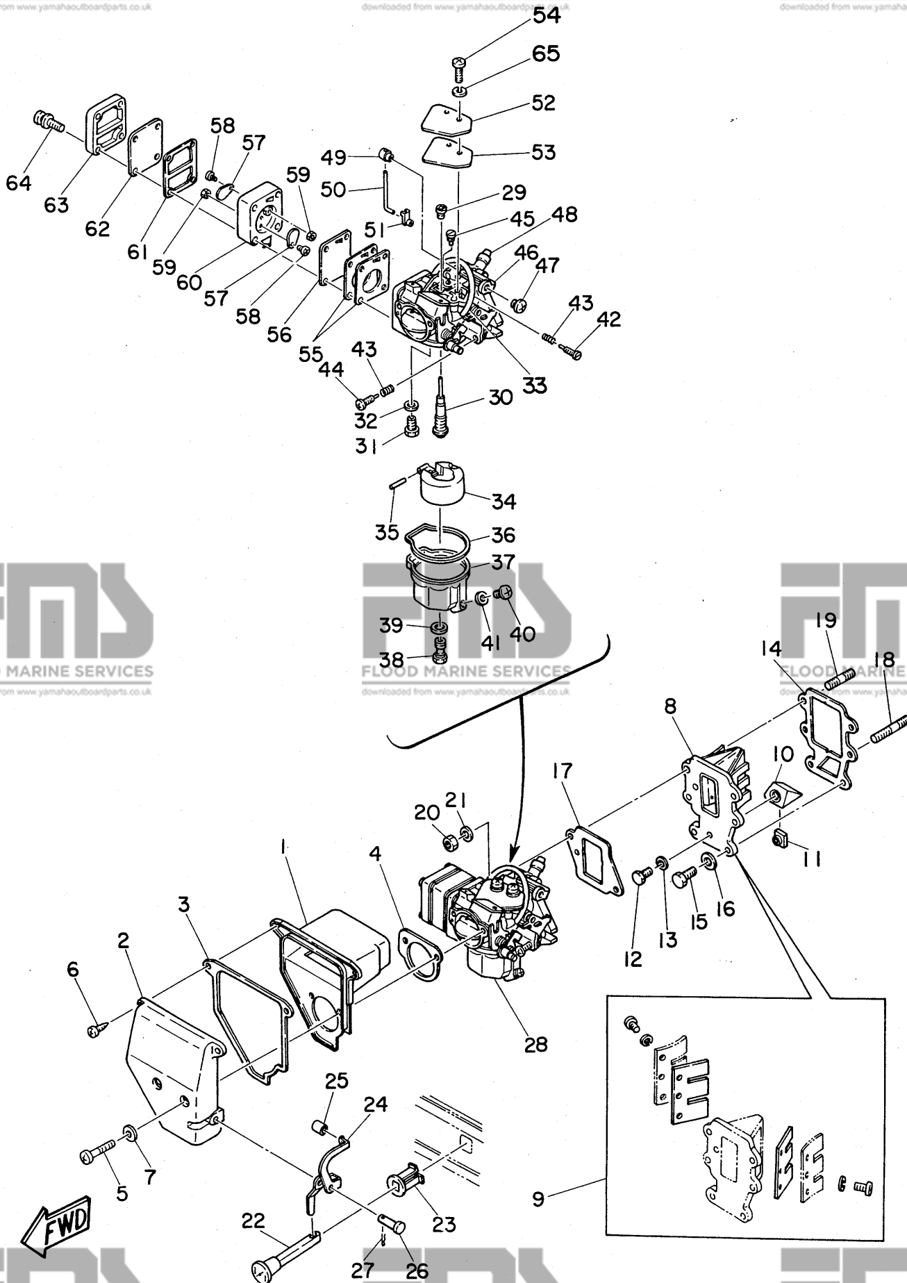
Fig. 3 INTAKE
