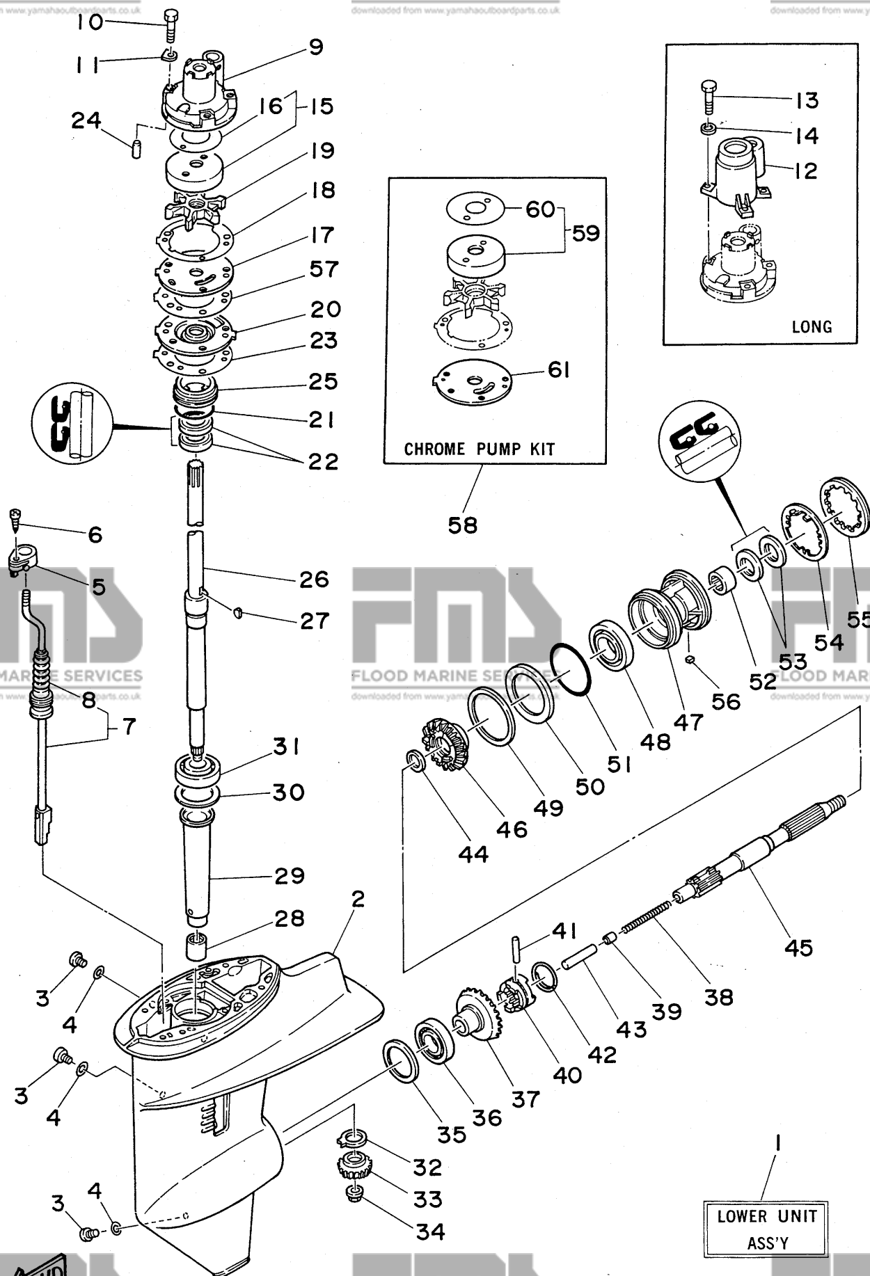
Fig. 12 LOWER & DRIVE I
