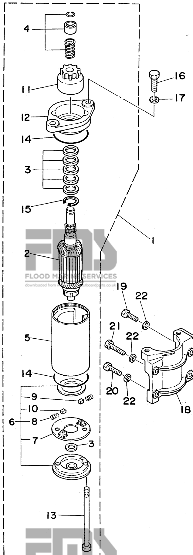
Fig. 18 ELECTRIC MOTOR (6CEM/6DEM/8CEM MODEL)
