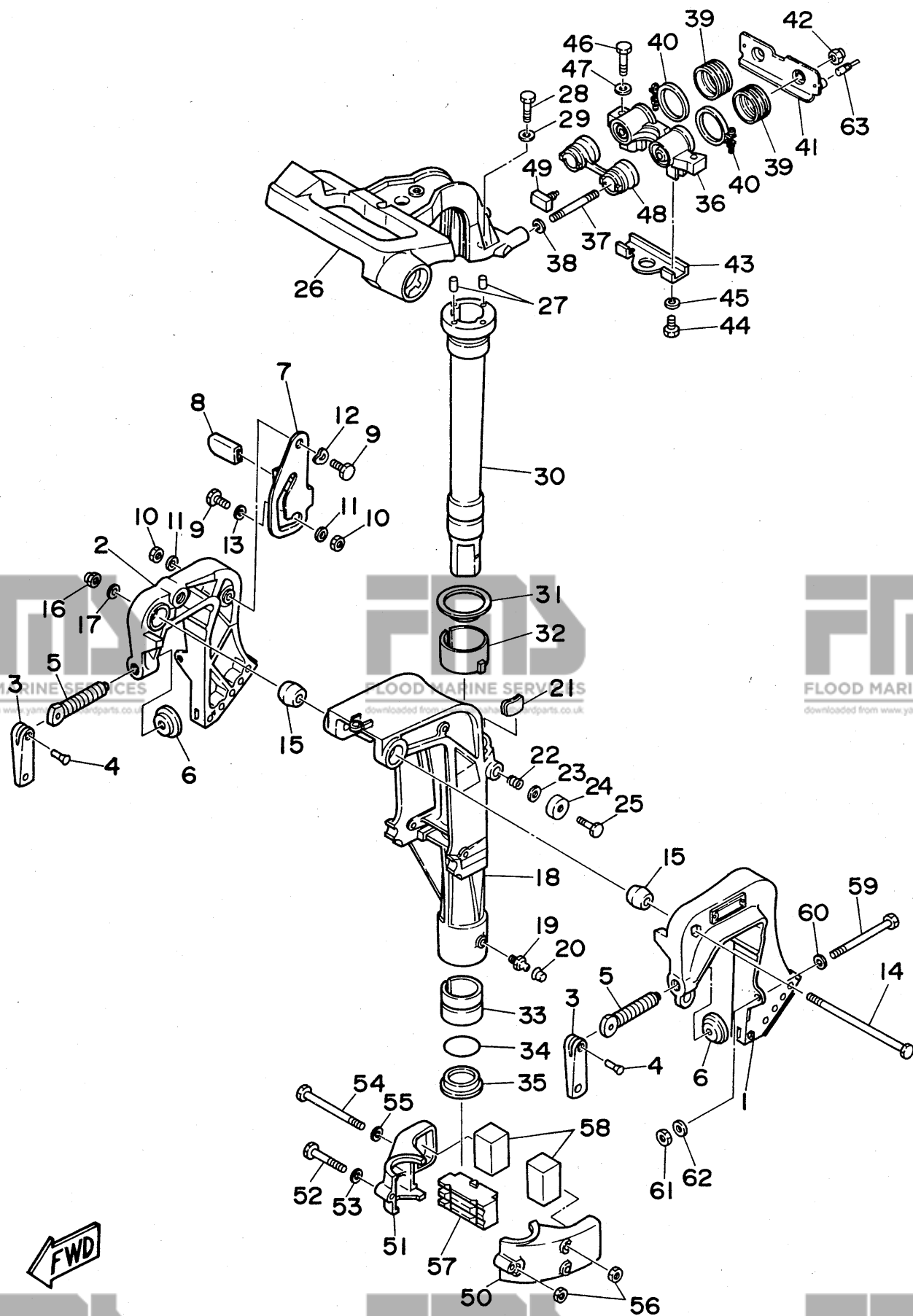
Fig. 11 BRACKET 1
