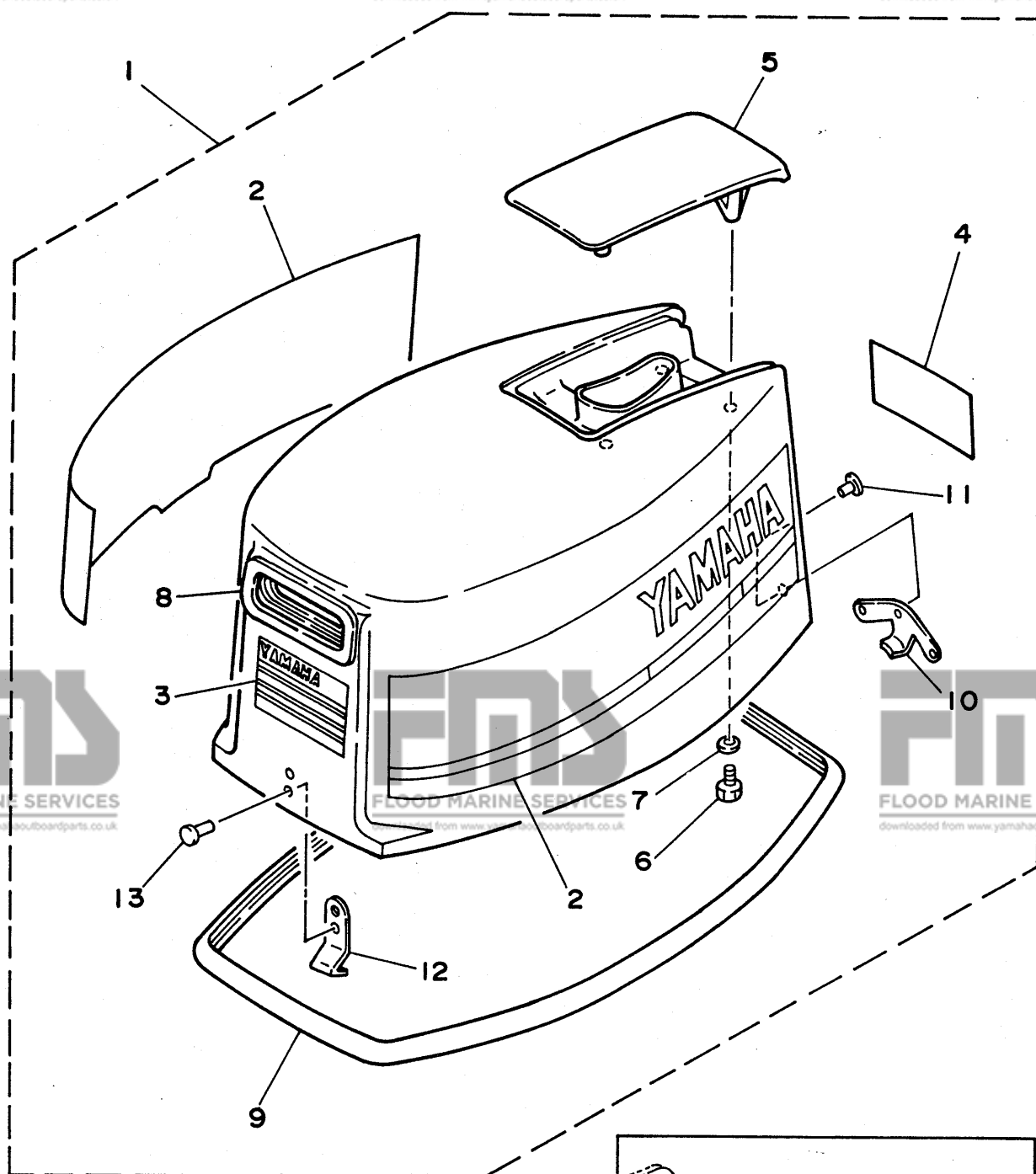
Fig. 6 TOP COWLING
