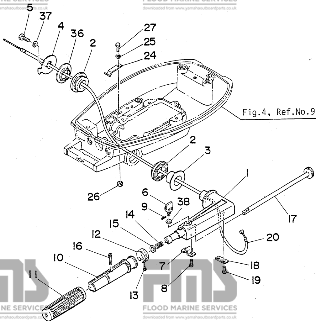
Fig. 6 CONTROL
