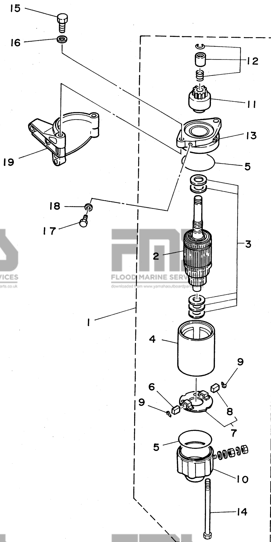
Fig. 22 STARTING MOTOR (F8AEM/F9.9AEM/F9.9AE MODEL)
