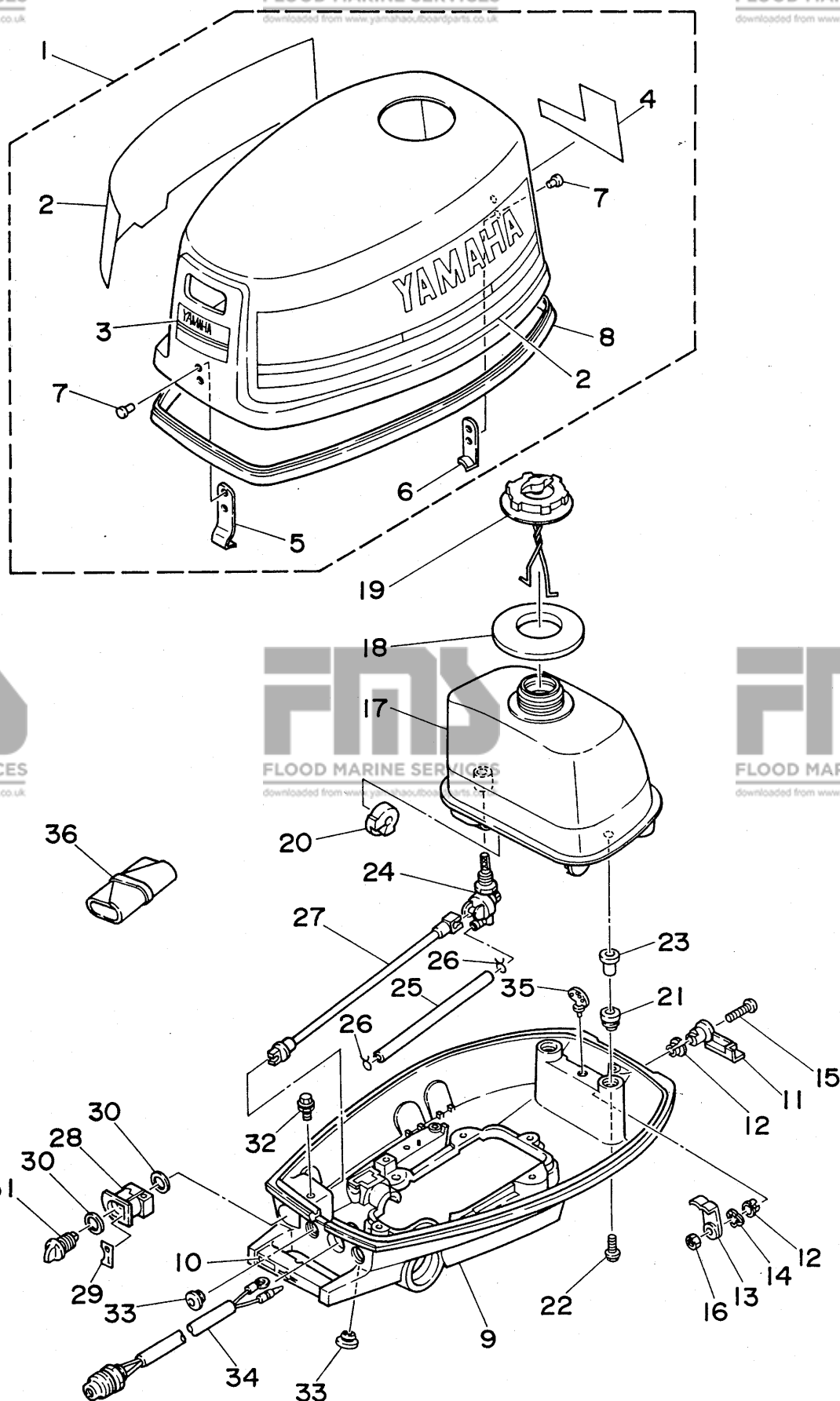
Fig. 4 COWLING & FUEL
