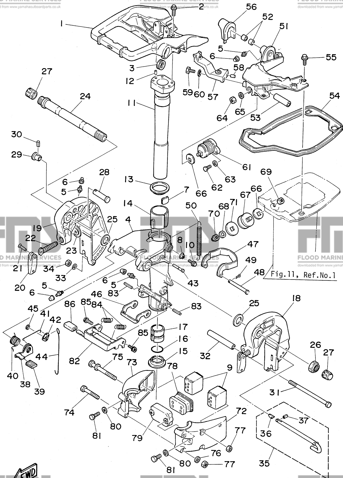
Fig. 8 BRACKET
