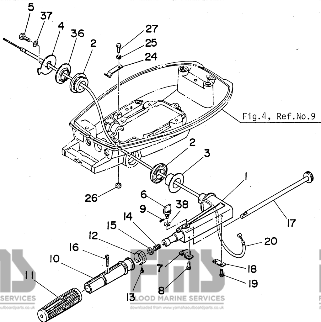
Fig. 6 CONTROL
