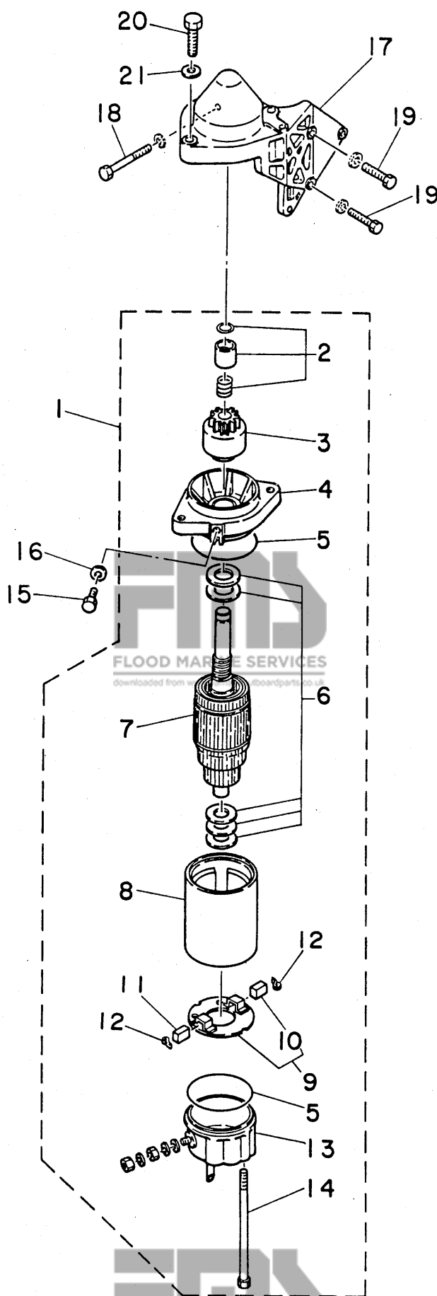
Fig. 16 ELECTRIC MOTOR (25DE MODEL)
