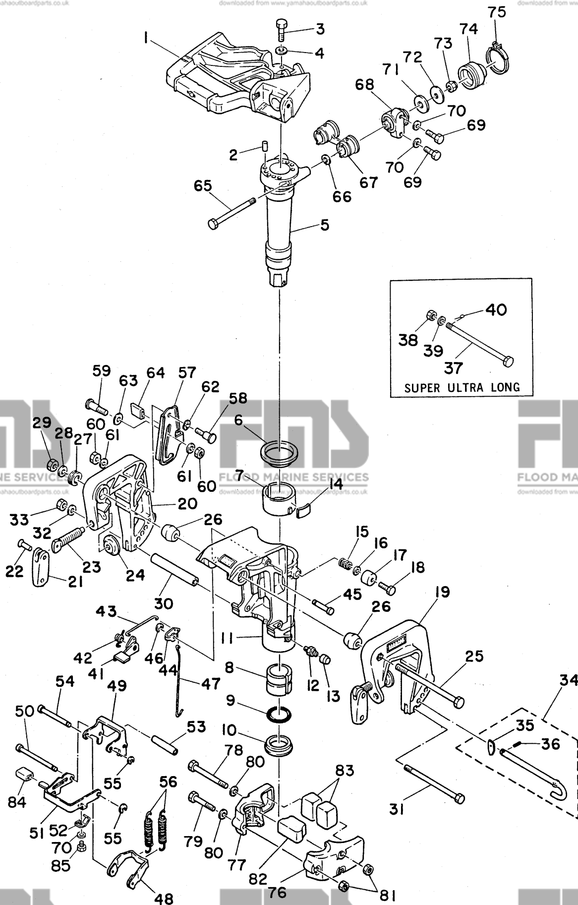
Fig. 8 BRACKET
