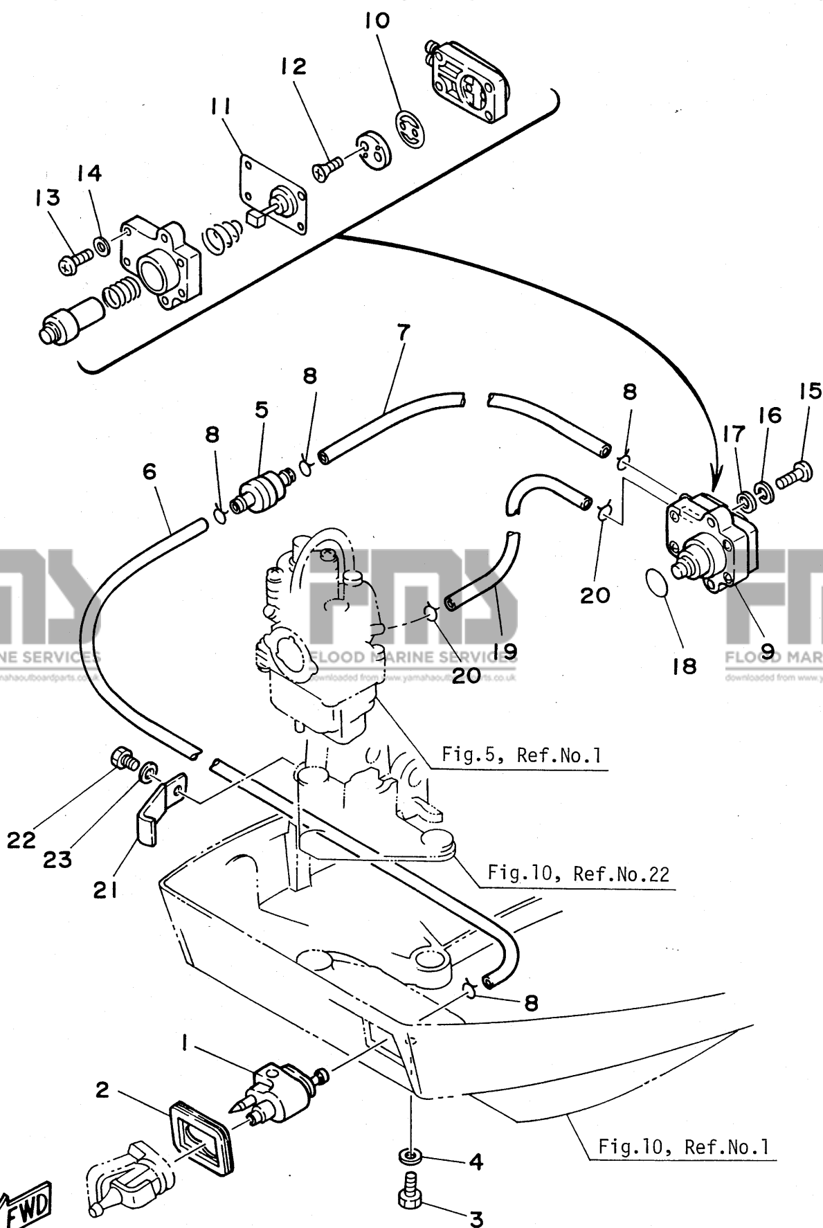
Fig. 8 FUEL
