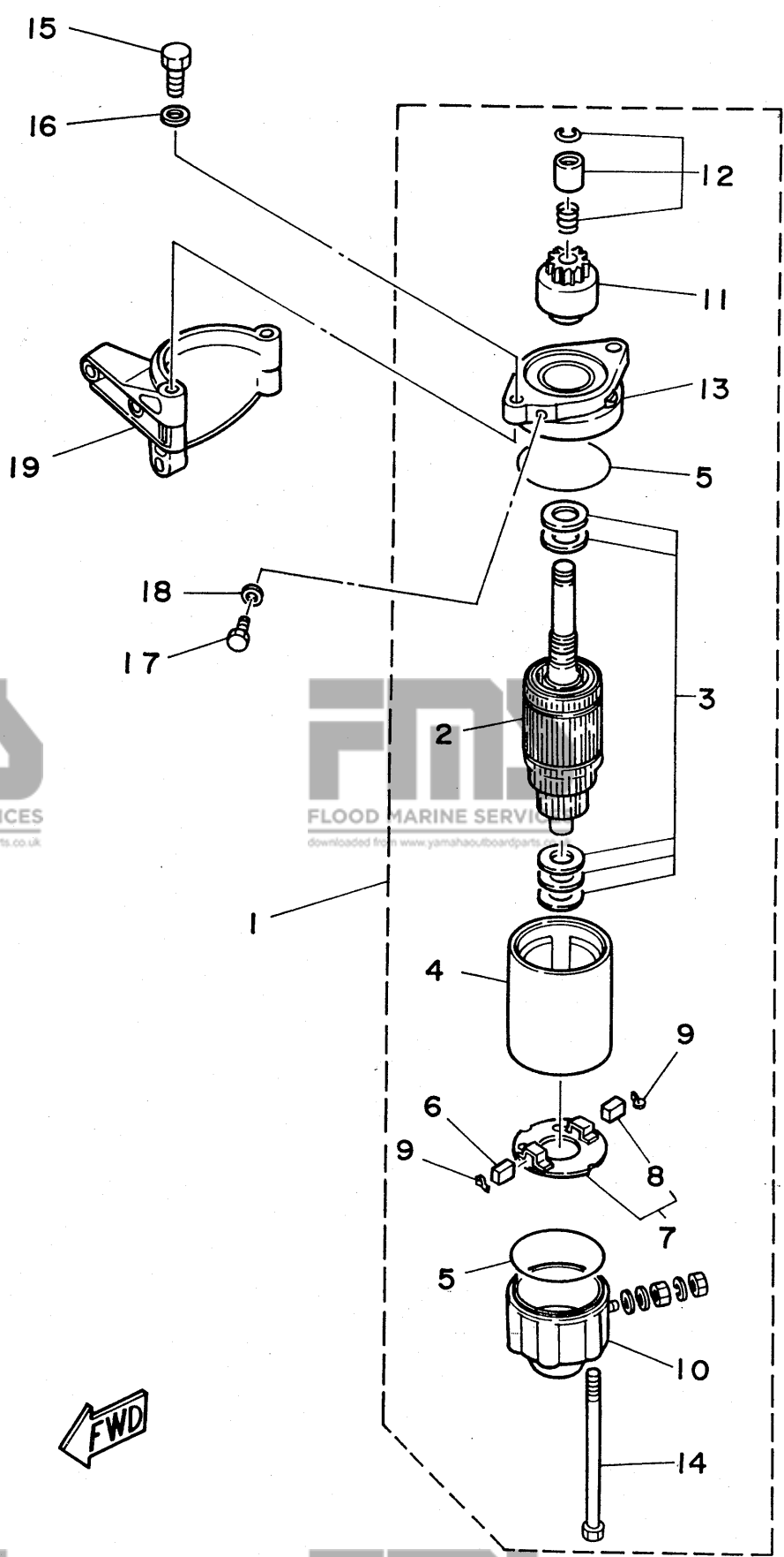
Fig. 22 STARTING MOTOR (F8BEM/F8BE/F9.9BEM/F9.9BE MODEL)
