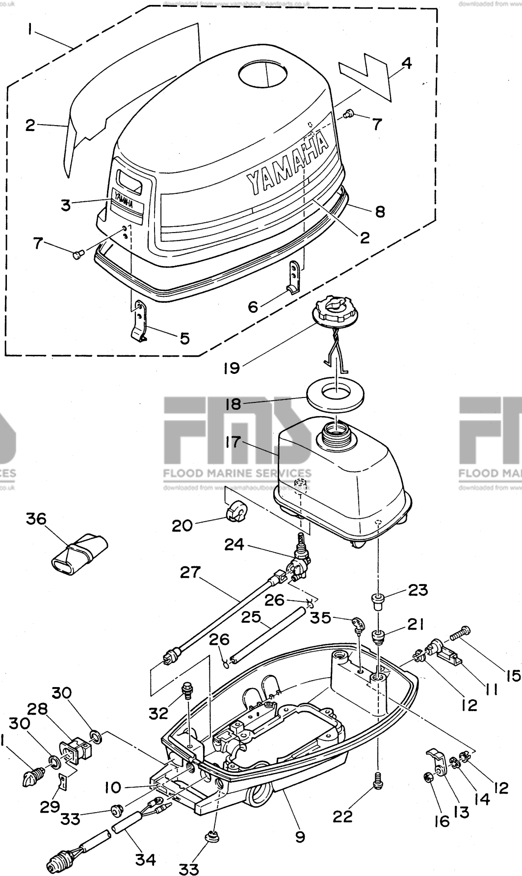
Fig. 4 COWLING & FUEL
