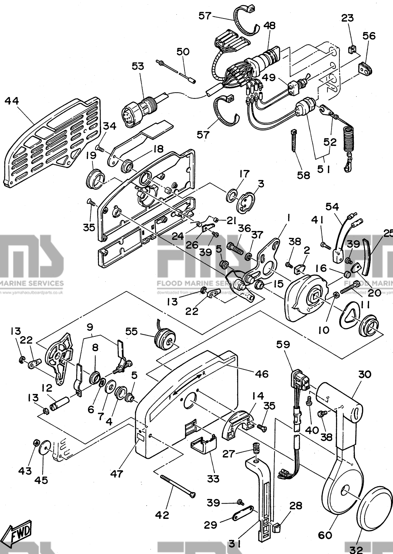
Fig. 7 REMOTE CONTROL ASS'Y 2 (PULL TO OPEN TYPE)
