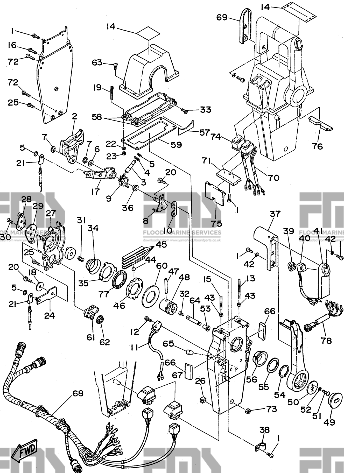
Fig. 10 REMOTE CONTROL ASS'Y 5 (PUSH TO OPEN TYPE)
