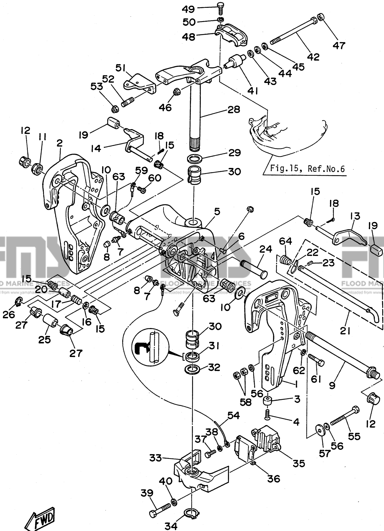
Fig. 12 BRACKET (50DETO MODEL)
