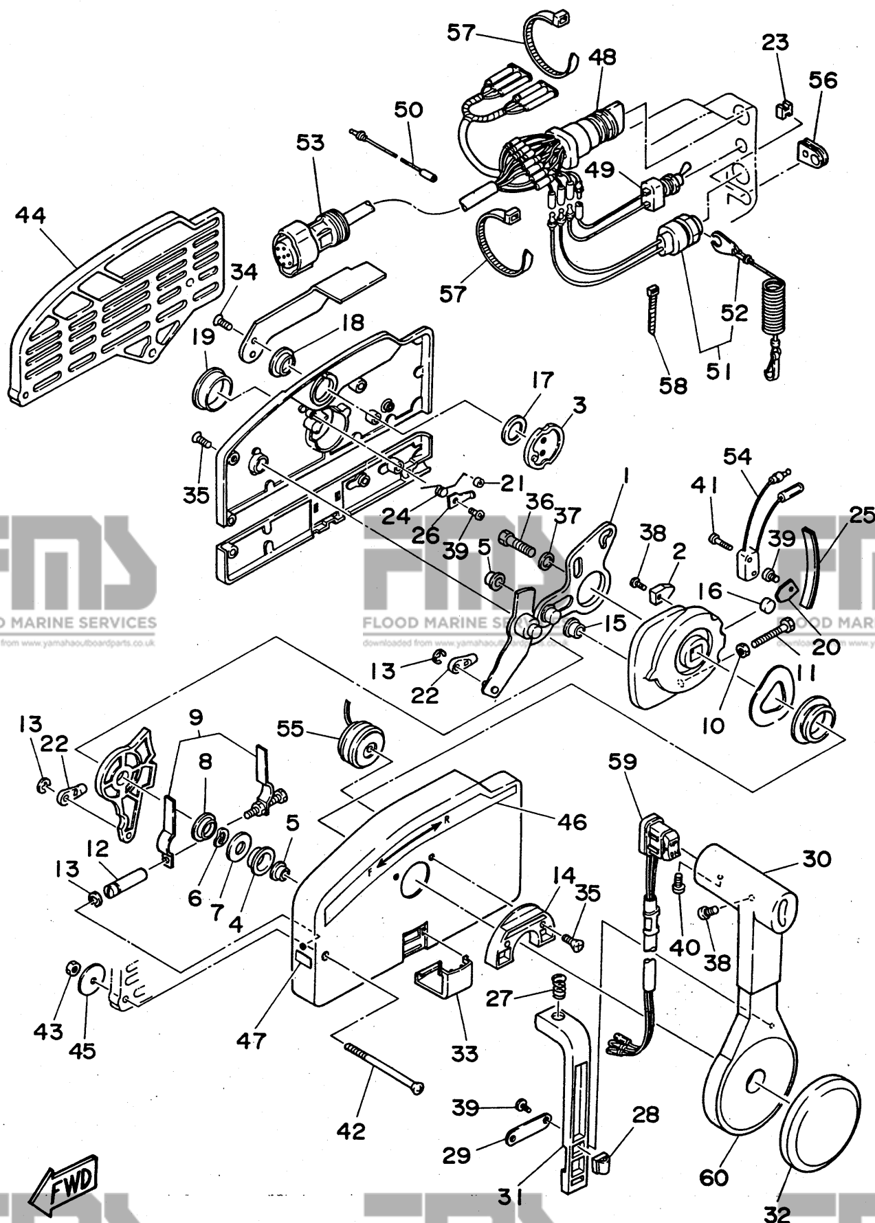
Fig. 8 REMOTE CONTROL ASS'Y 3 (PUSH TO OPEN TYPE)
