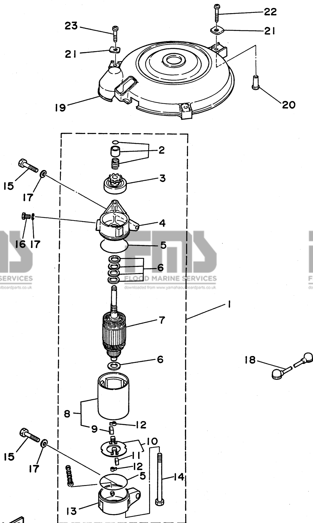
Fig. 22 ELECTRIC STARTER (40HEO/40HEPO MODEL)
