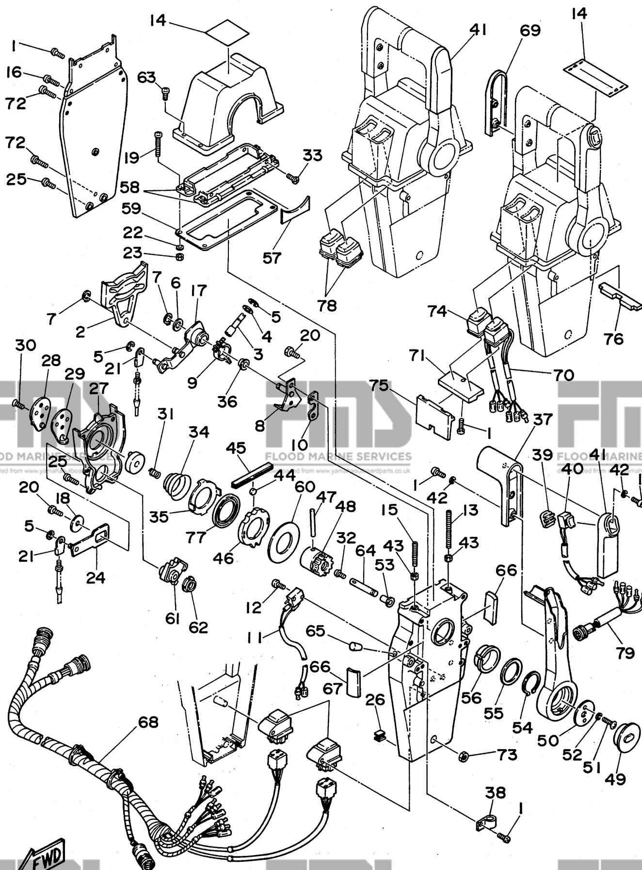
Fig. 9 REMOTE CONTROL ASS'Y 4 (PULL TO OPEN TYPE)
