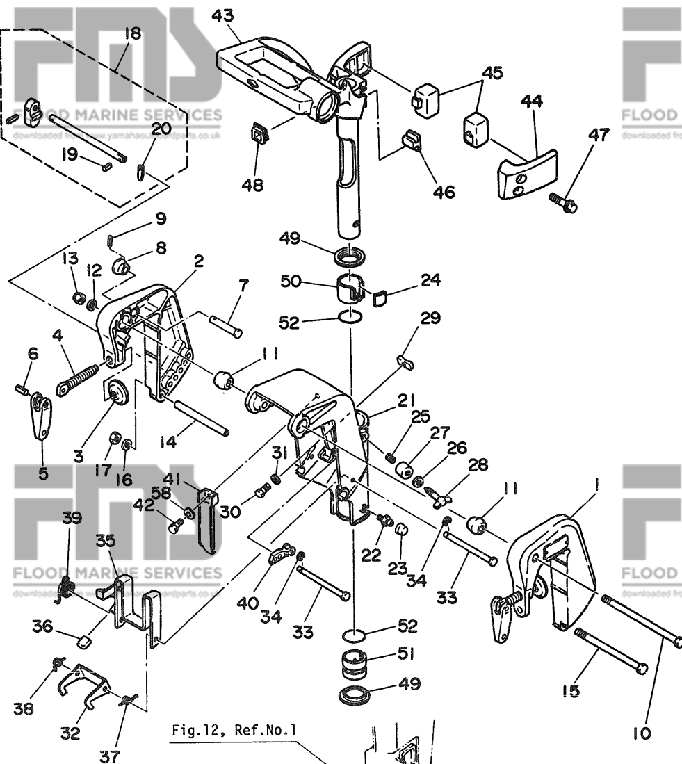
Fig. 9 BRACKET
