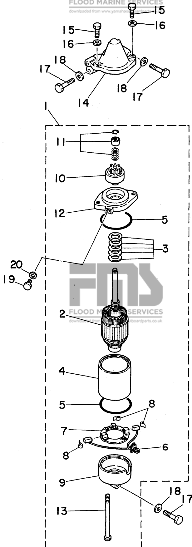
Fig. 16 ELECTRIC MOTOR
