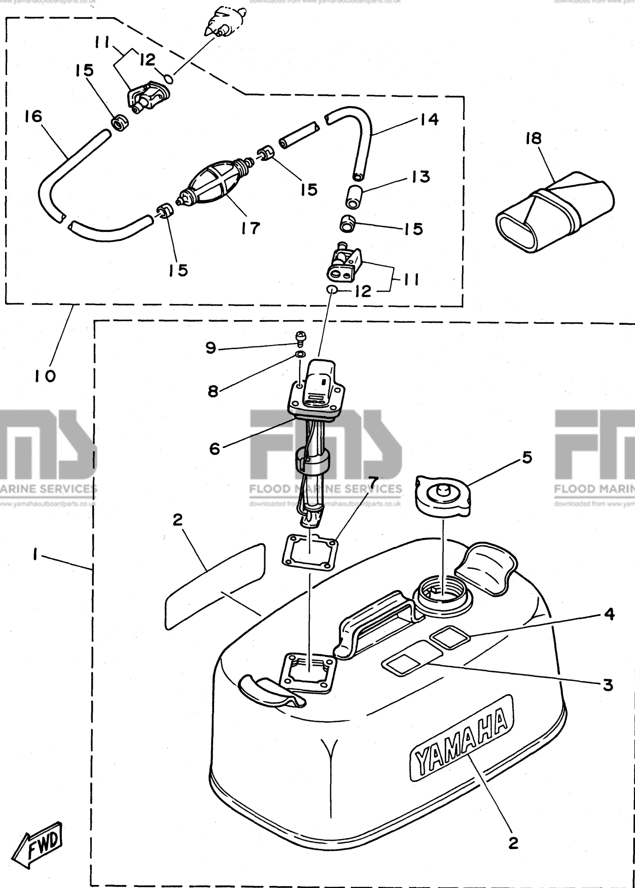
Fig. 1 FUEL TANK & FUEL PIPE (115AETO THRU 220AETO)
