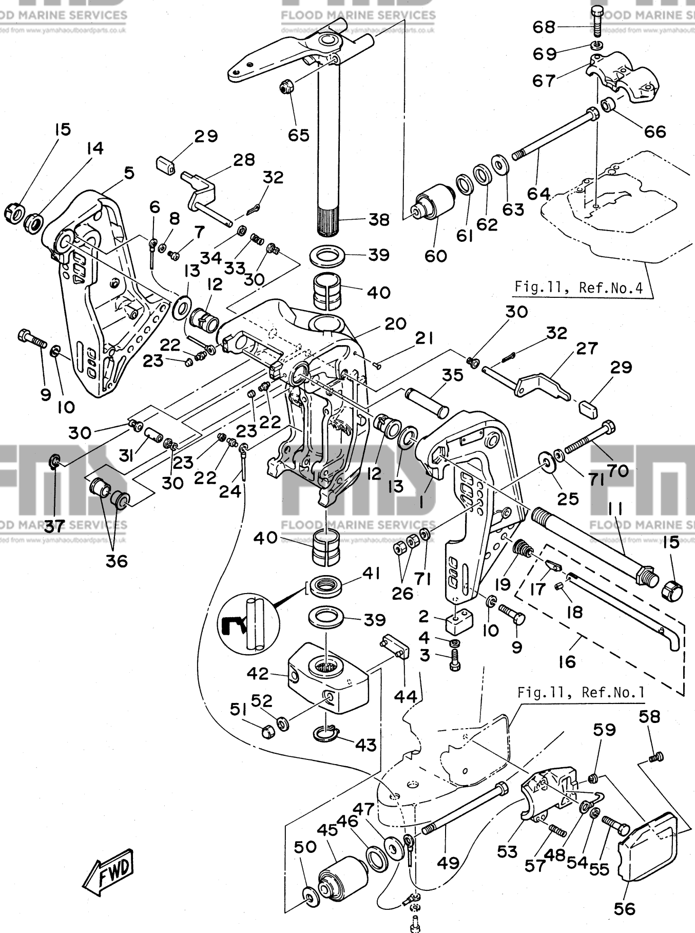
Fig. 8 BRACKET
