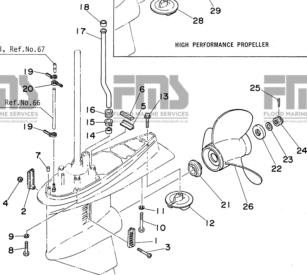
Fig.13, Ref.No.1 LOWER UNIT ASS'Y
