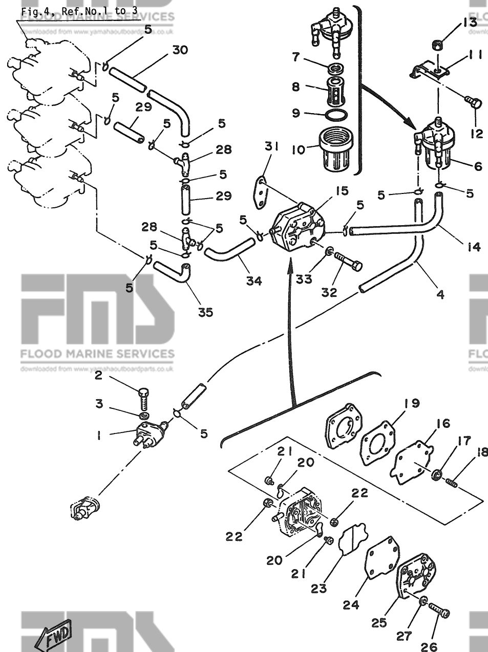
Fig.4, Ref.No.1 to 3
