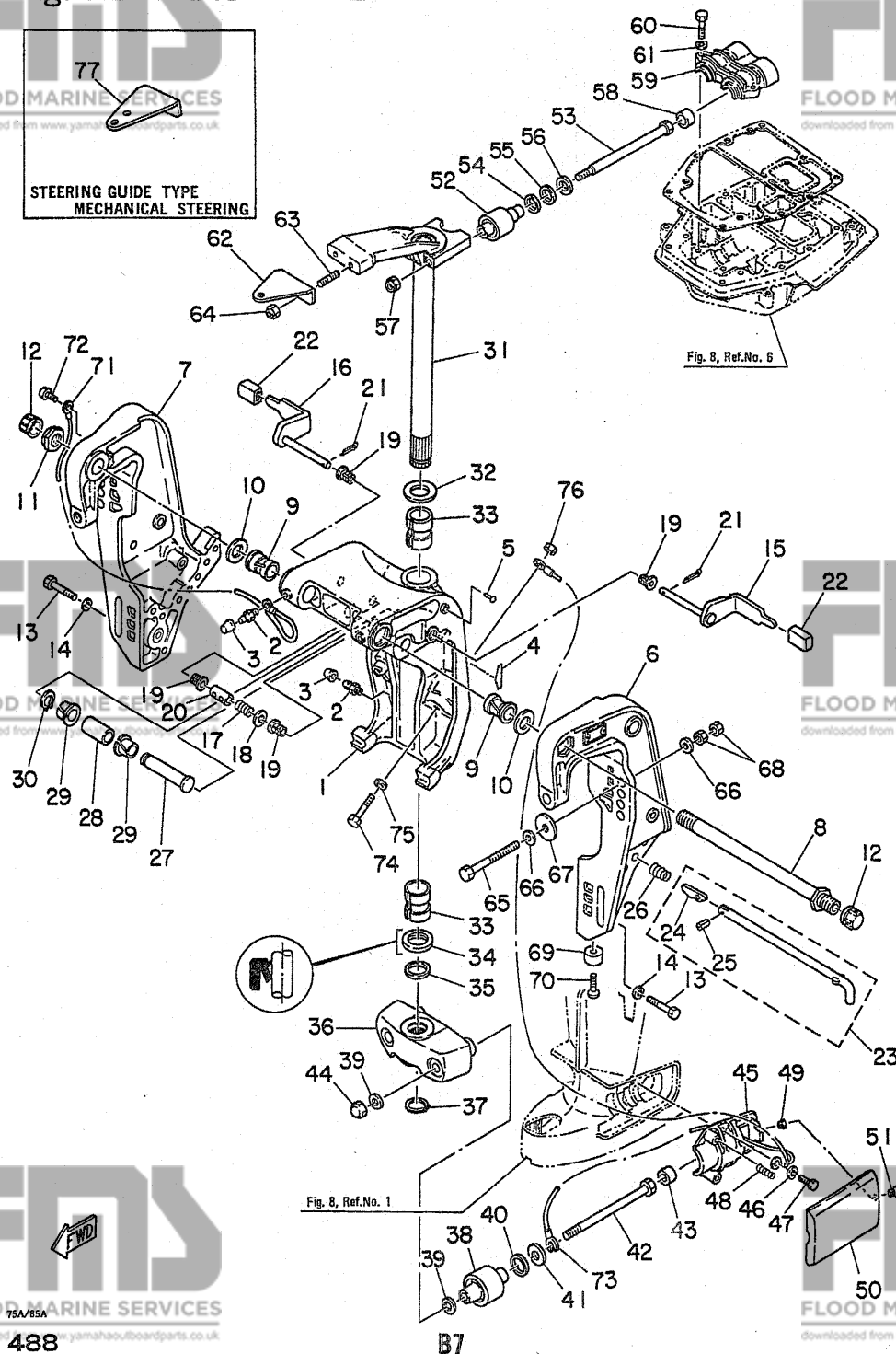
Fig. 12 BRACKET 2
