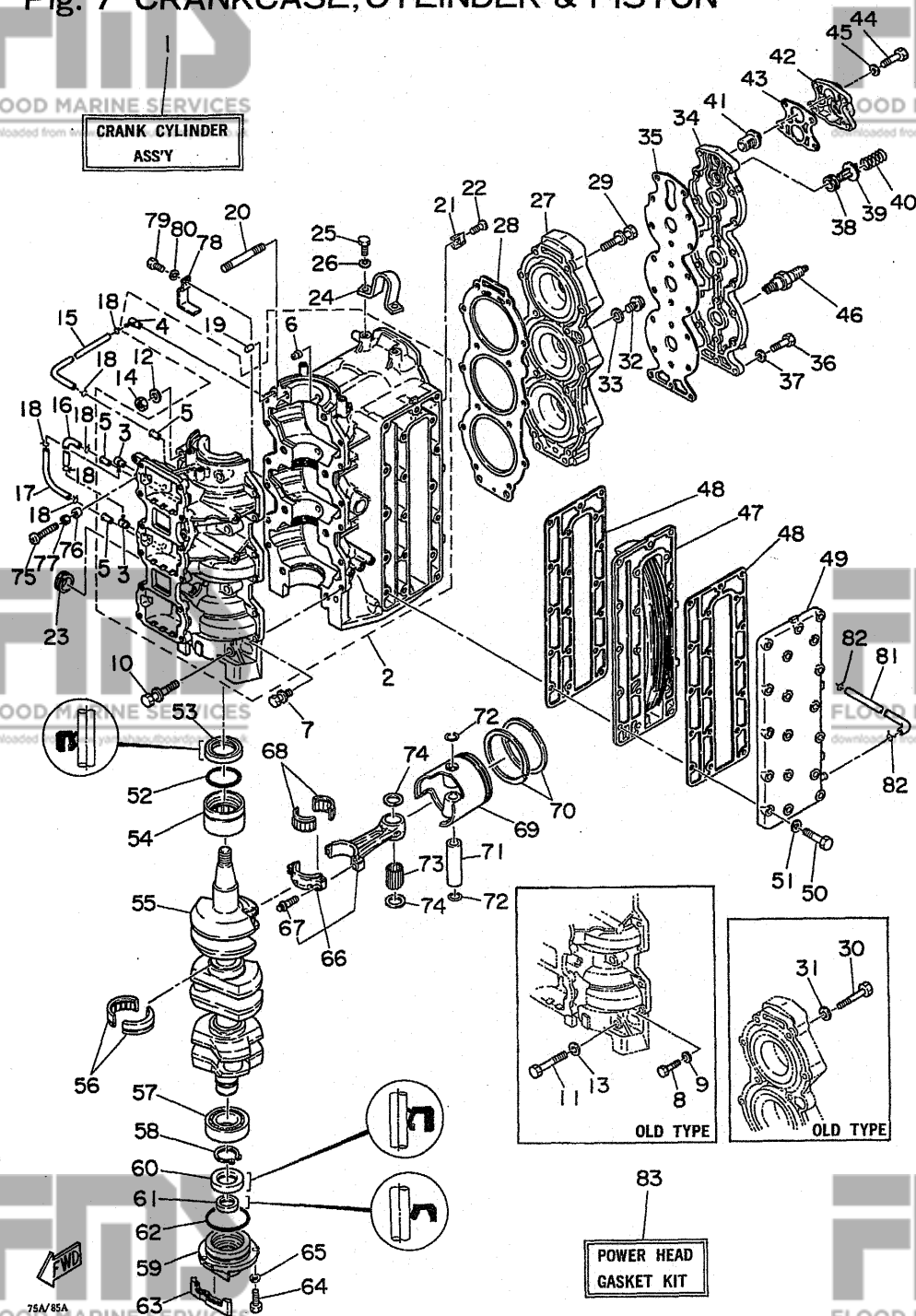
Fig. 7 CRANKCASE, CYLINDER &amp; PISTON
