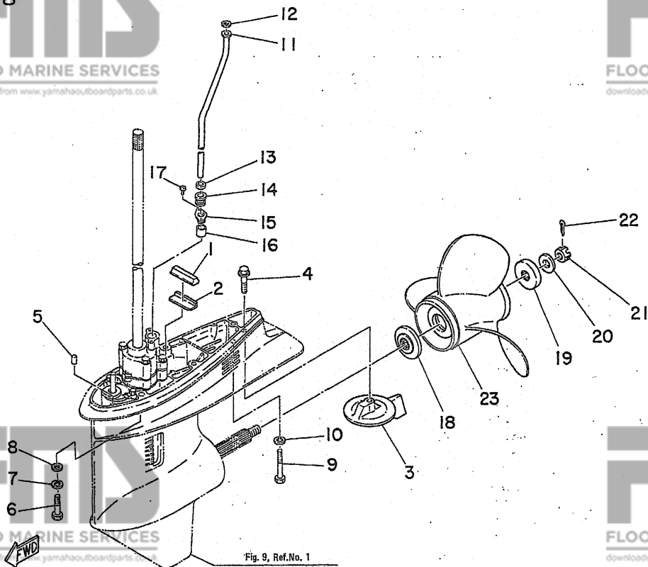
Fig. 9, Ref. No. 1 LOWER UNIT ASS'Y
