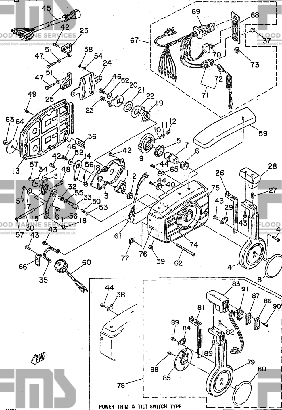
Fig. 17 REMOTE CONTROL ASS'Y I
