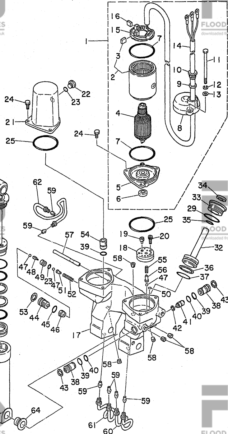
Fig. 16 POWER TRIM & TILT 2 (75AET/85AET MODEL)
