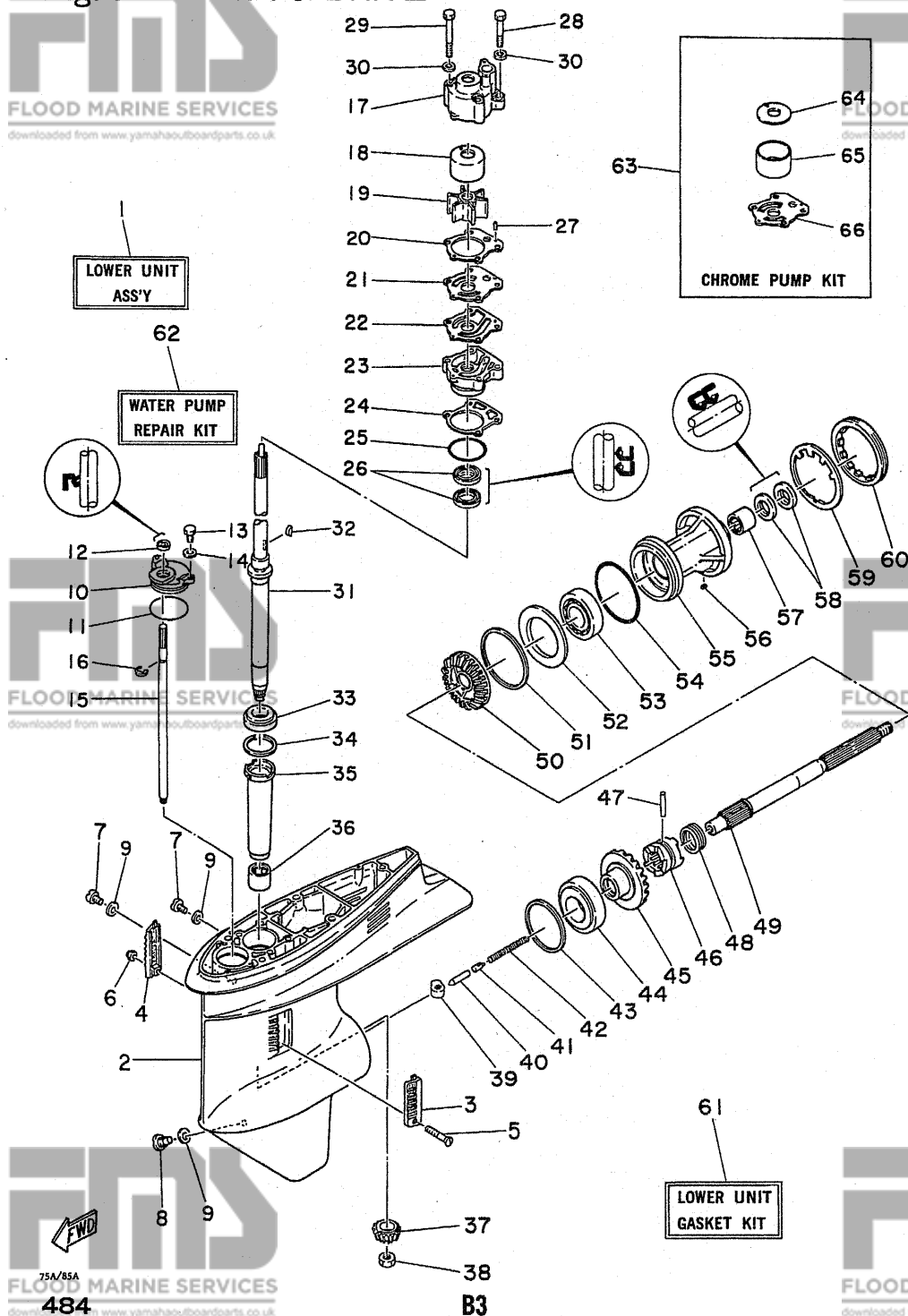
Fig. 9 LOWER &amp; DRIVE I
