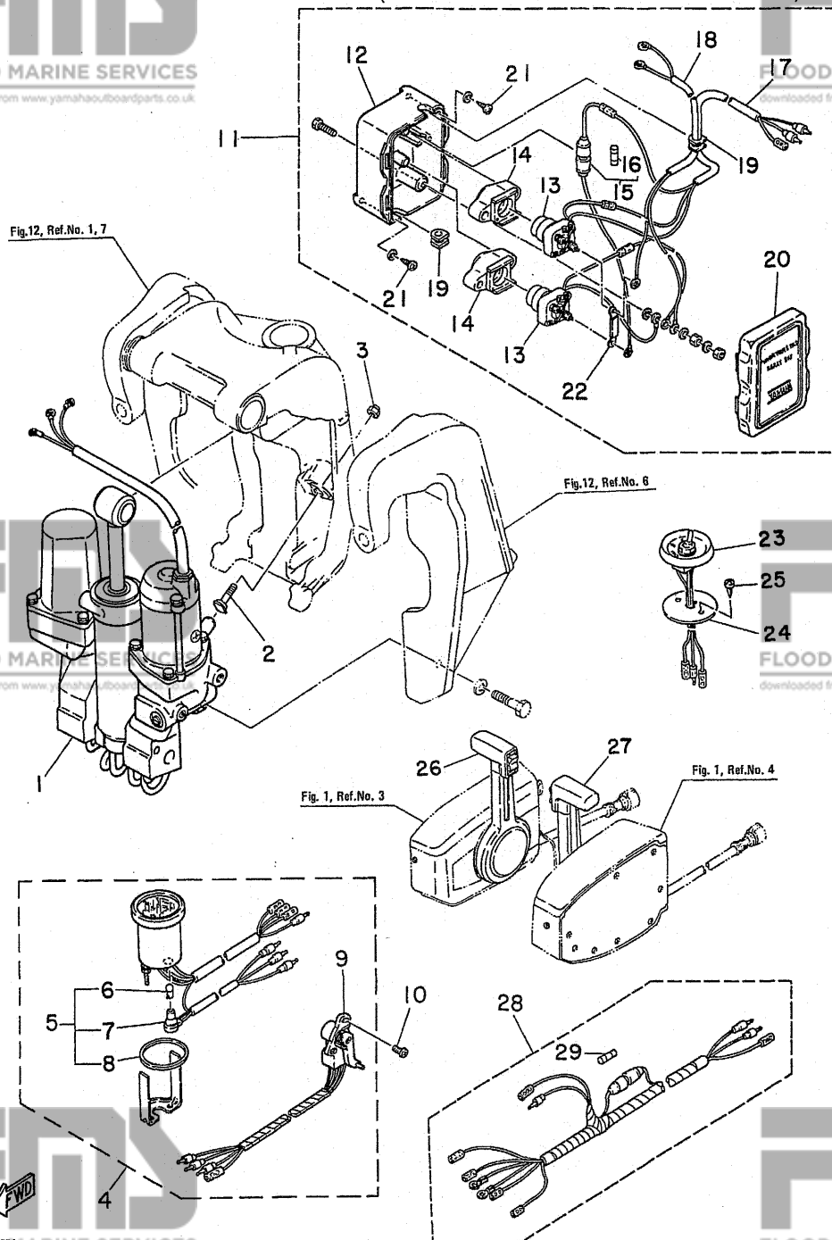
Fig. 15 POWER TRIM & TILT I (75AET/85AET MODEL)
