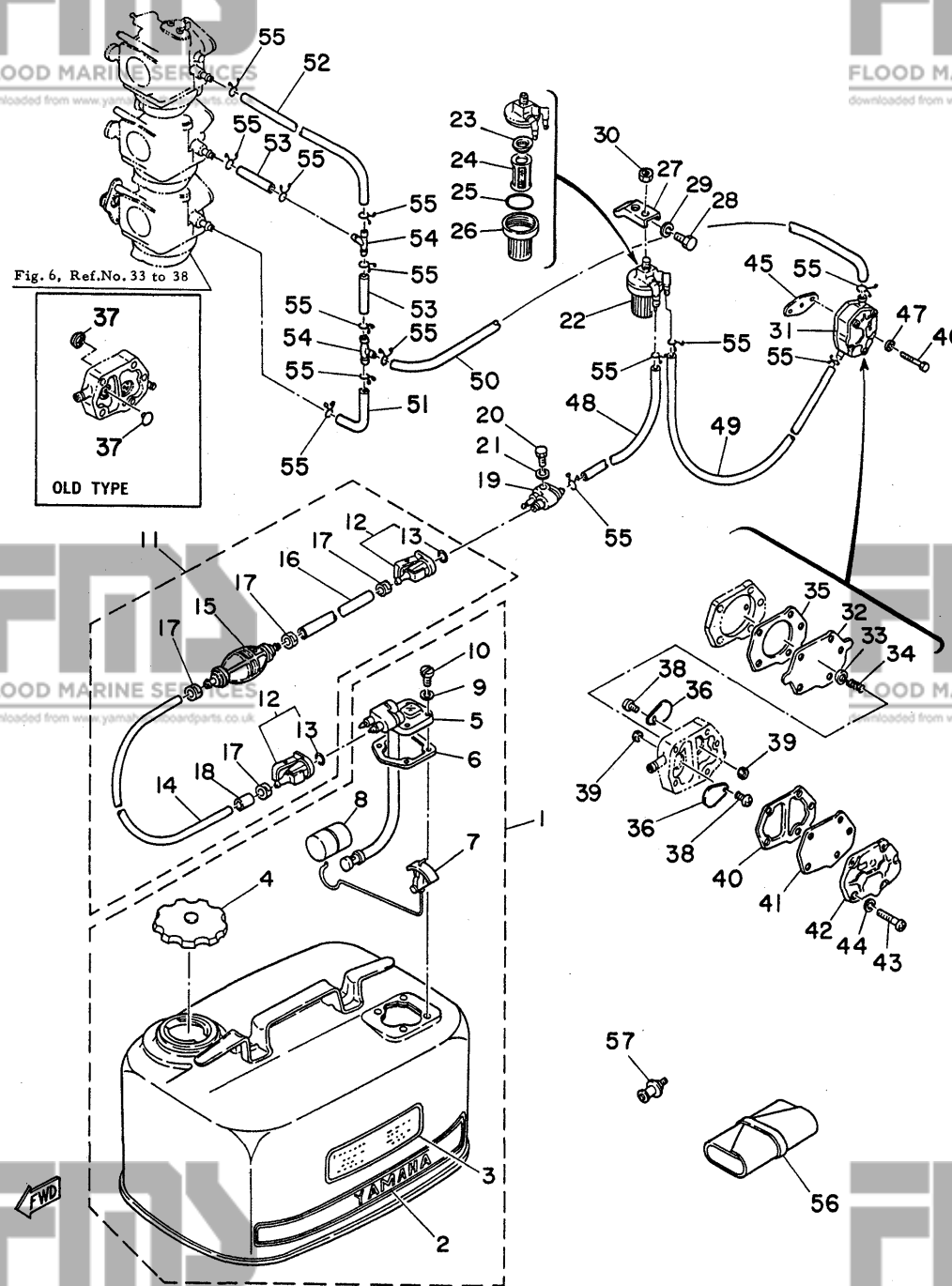
Fig. 14 FUEL SECTION -'80/'81
