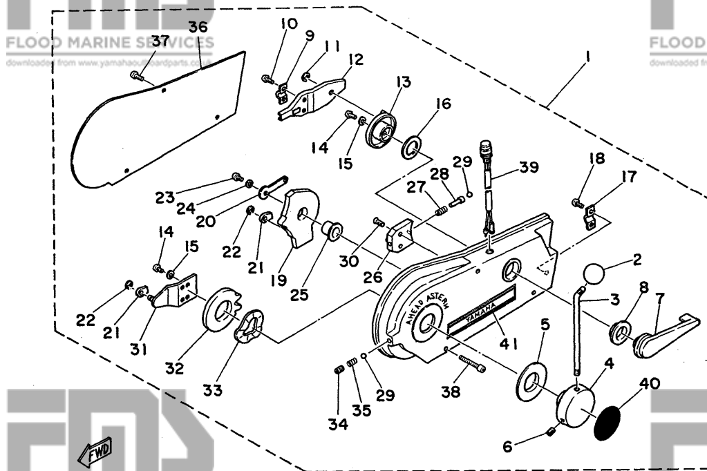
Fig.25 ACCESSORY PARTS 6-'80/'81
