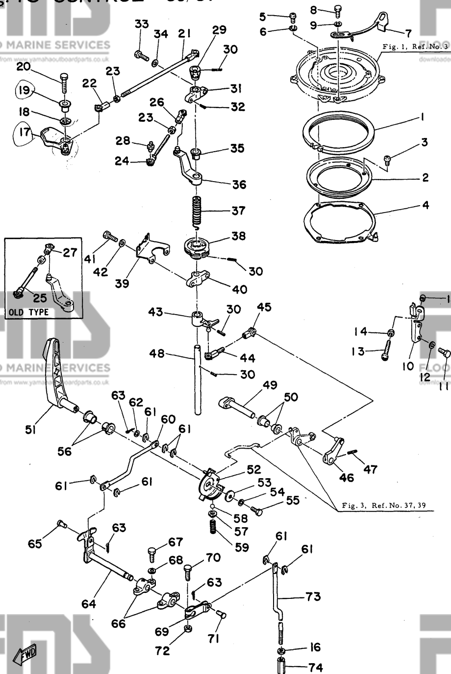
Fig. 13 CONTROL -'80/'81
