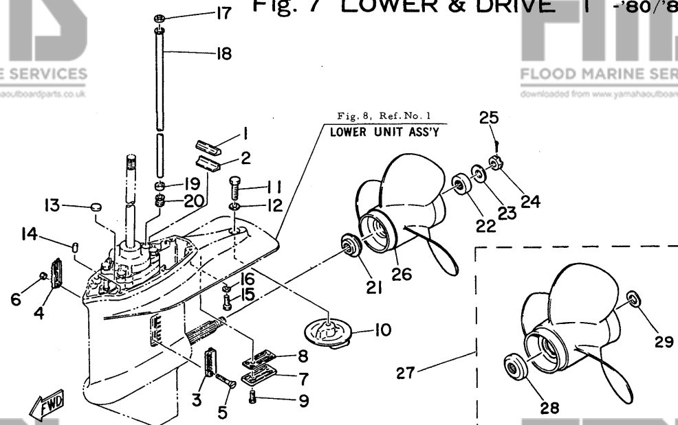
Fig. 7 LOWER &amp; DRIVE I '80/'81
