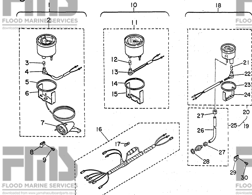
Fig. 19 ACCESSORY PARTS 1 '80/'81
