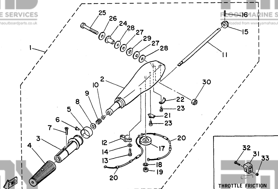
Fig. 12 STEERING -'80/'81
