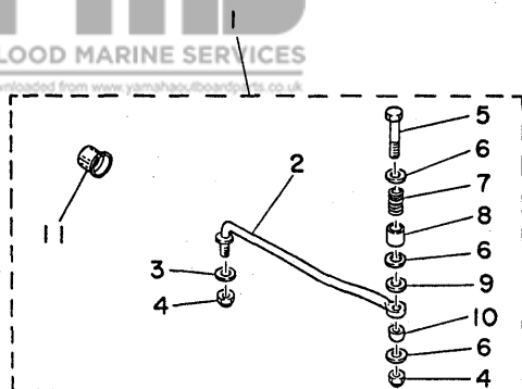
Fig. 23 ACCESSORY PARTS 5 '80/'81
