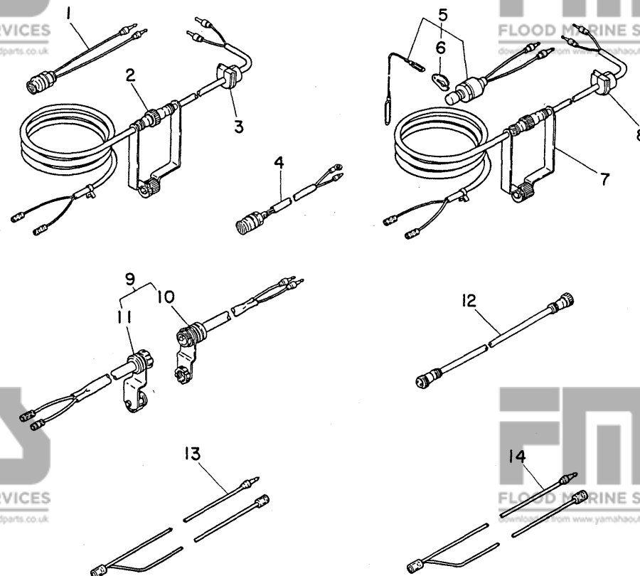
Fig. 22 ACCESSORY PARTS 4 -'80/'81
