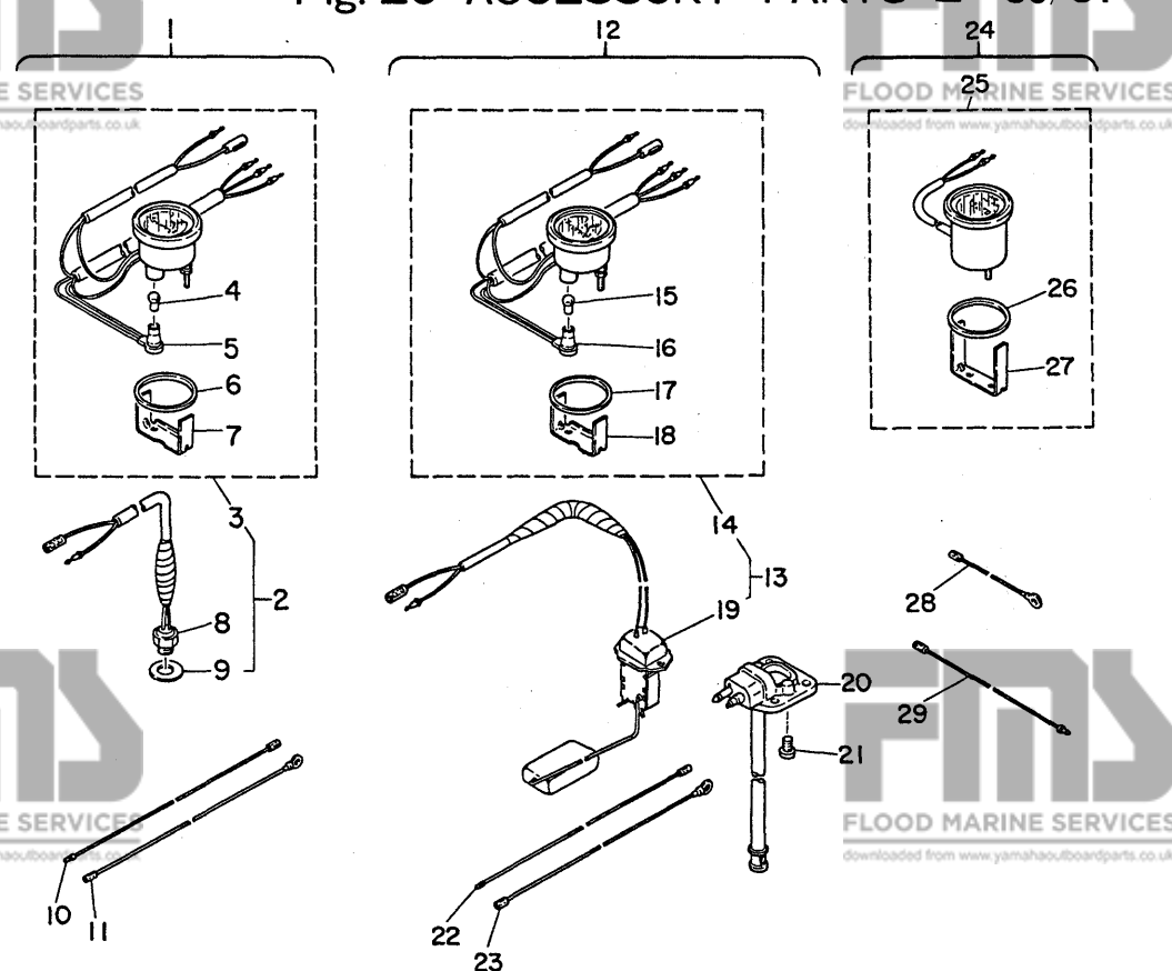
Fig. 20 ACCESSORY PARTS 2 '80/'81
