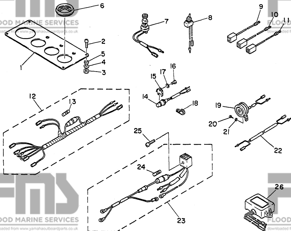
Fig. 21 ACCESSORY PARTS 3 -'80/'81
