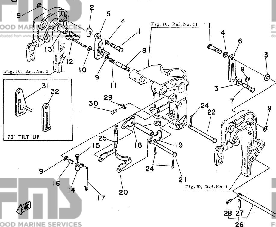
Fig. 11 BRACKET 2 -'80/'81
