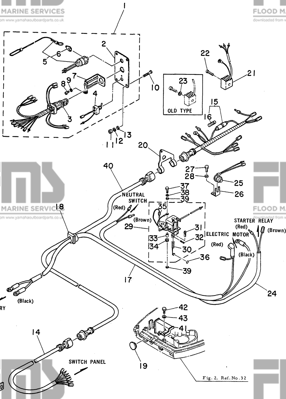
Fig. 15 ELECTRIC STARTER I (40DE MODEL) -'80/'81
