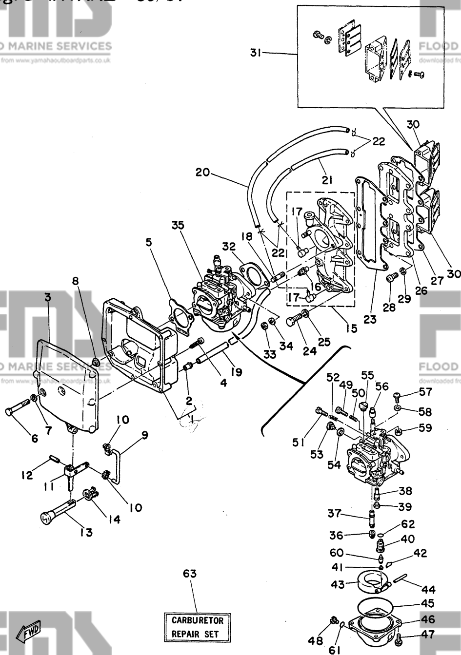
Fig. 5 INTAKE '80/'81
