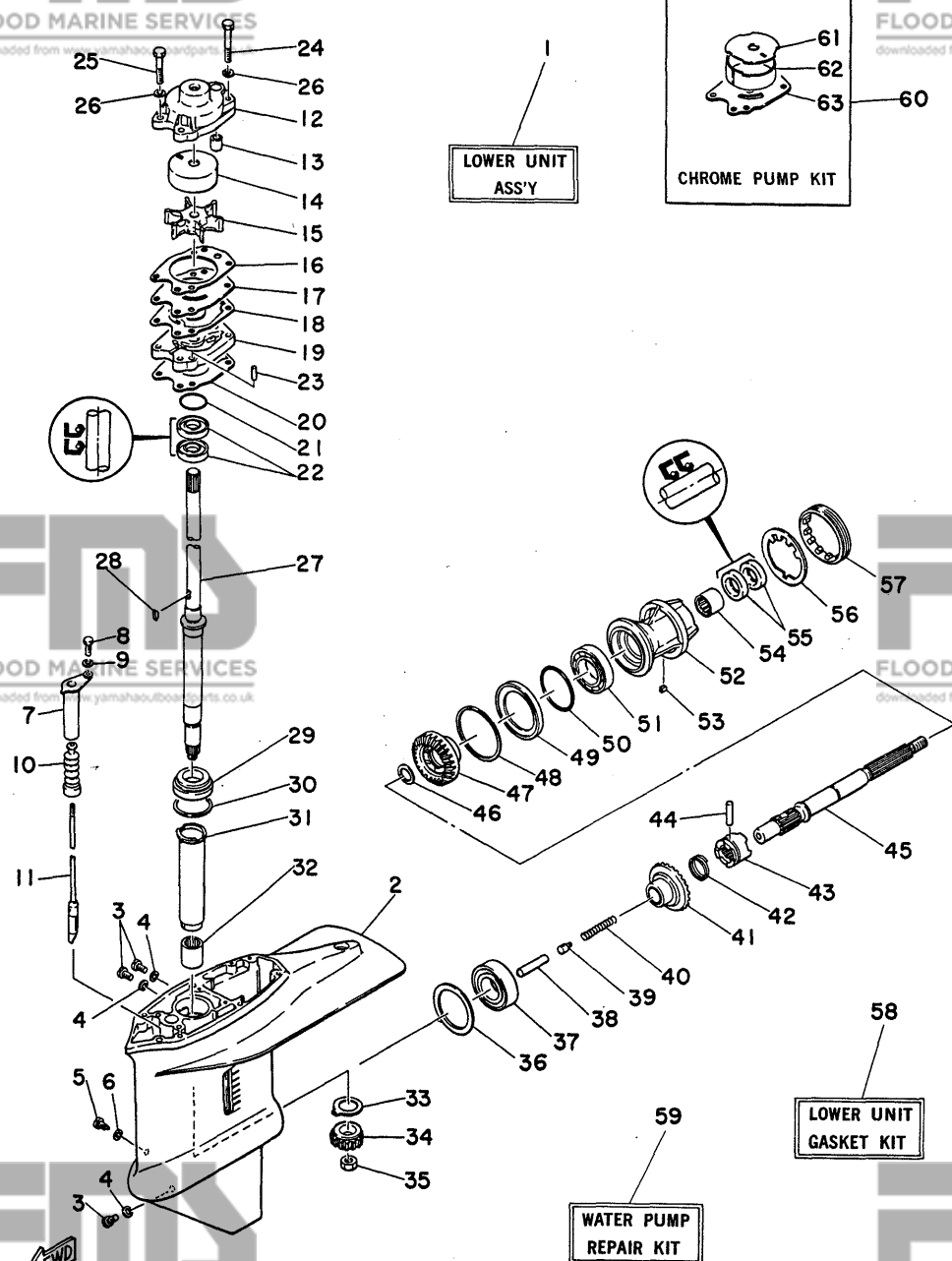
Fig. 8 LOWER &amp; DRIVE 2 -'80/'81
