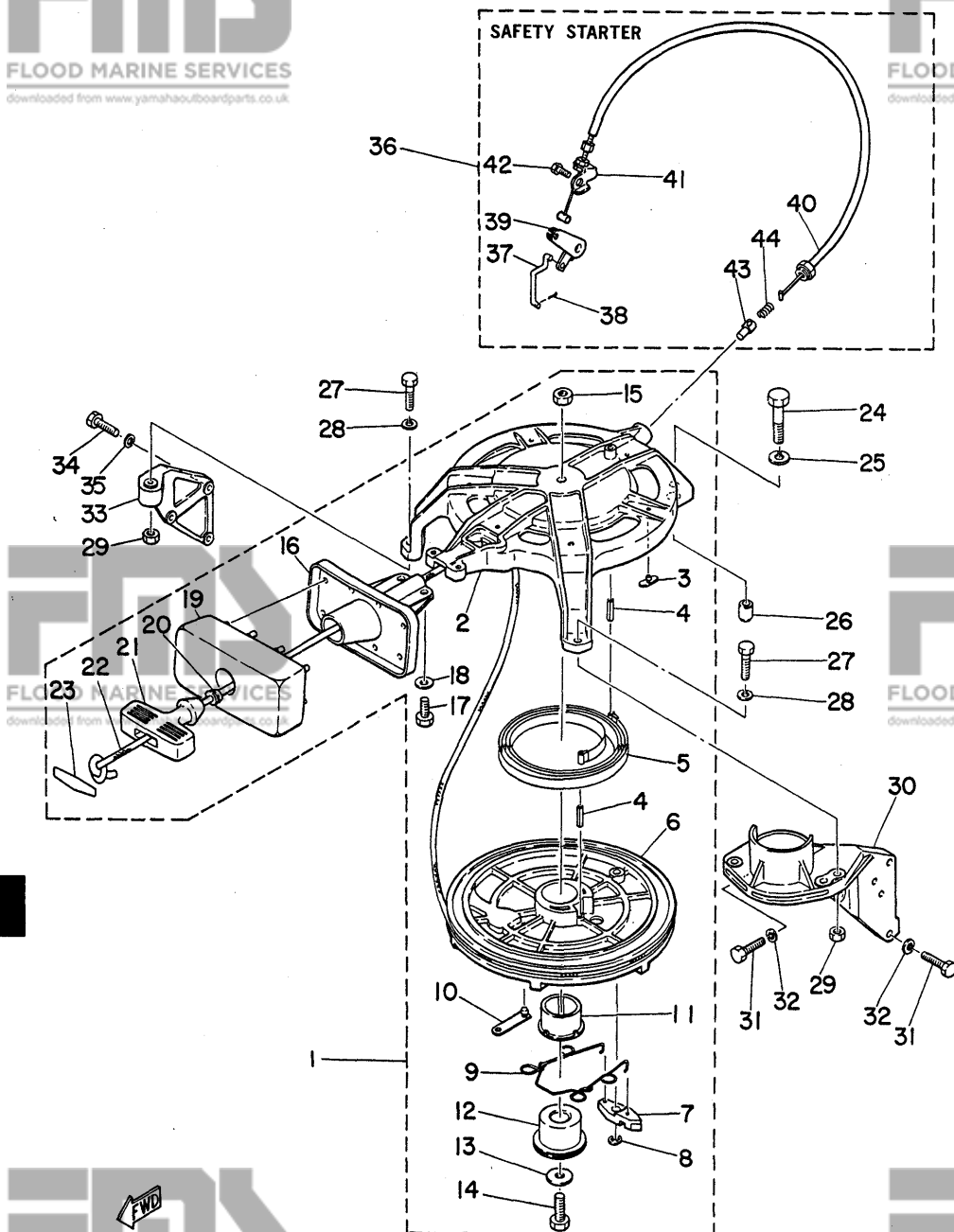
Fig. 3 STARTER '80/'81
