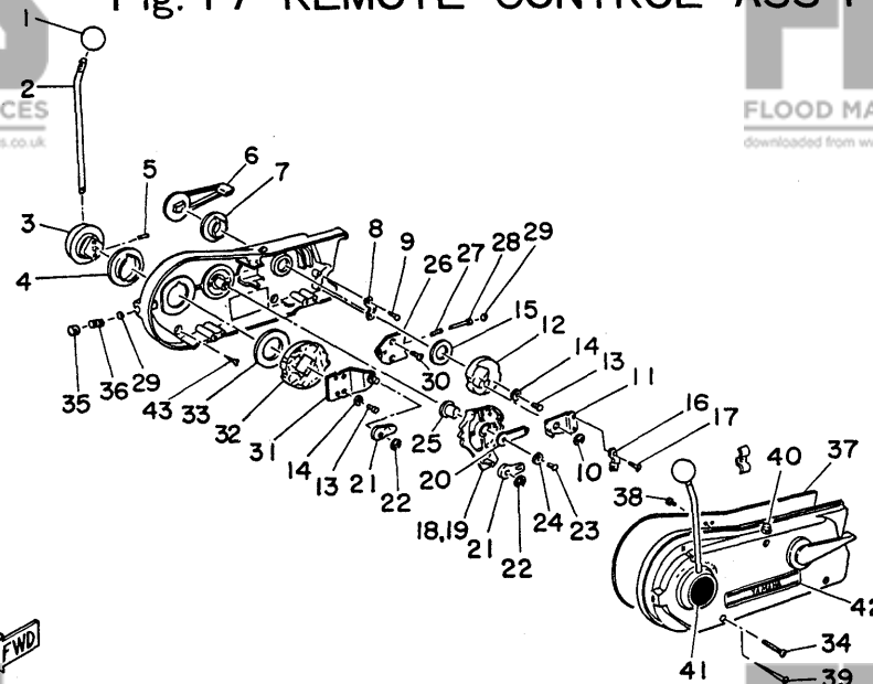
Fig. 17 REMOTE CONTROL ASS'Y '80/'81
