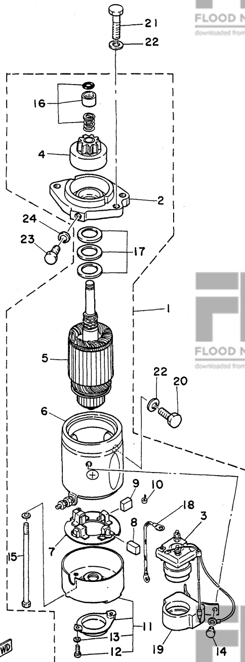
Fig. 16 ELECTRIC STARTER 2 (40DE MODEL) '80/'81
