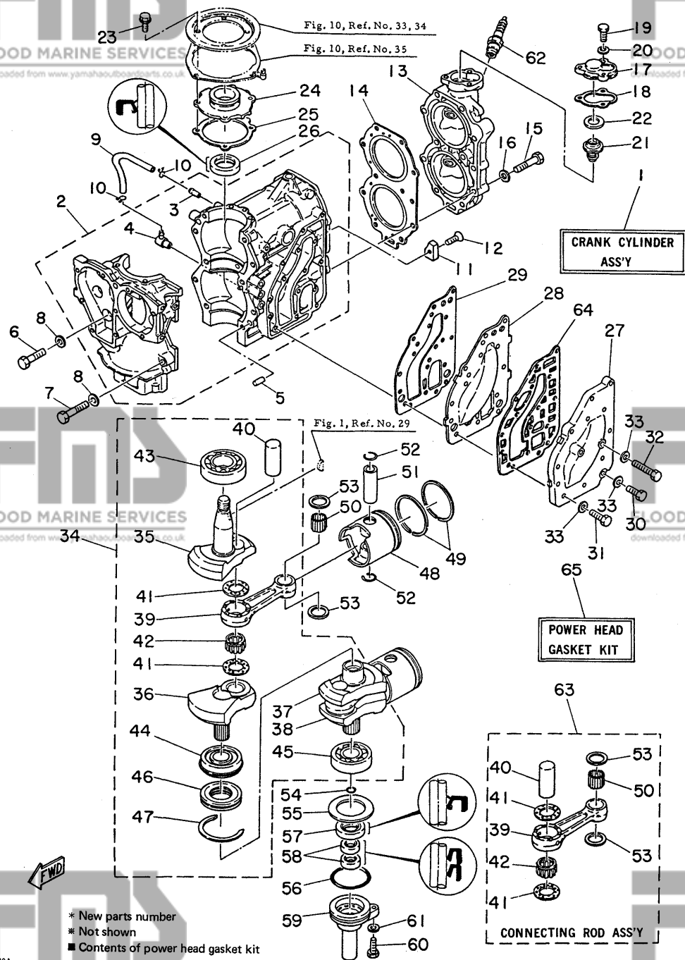
Fig. 4 CRANKCASE, CYLINDER &amp; PISTON '80/'81
