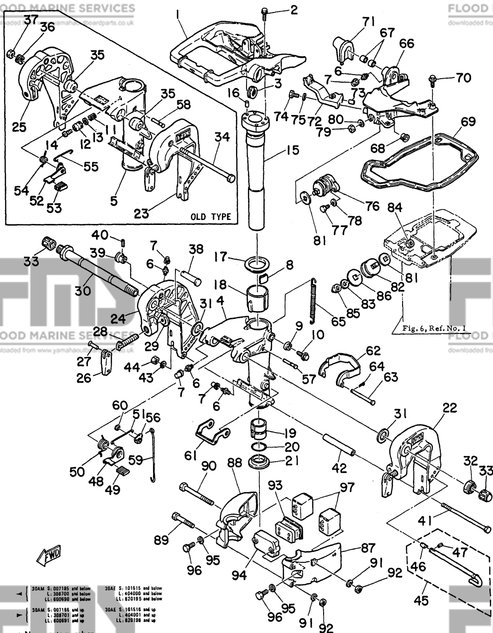
Fig. 9 BRACKET '80/'81
