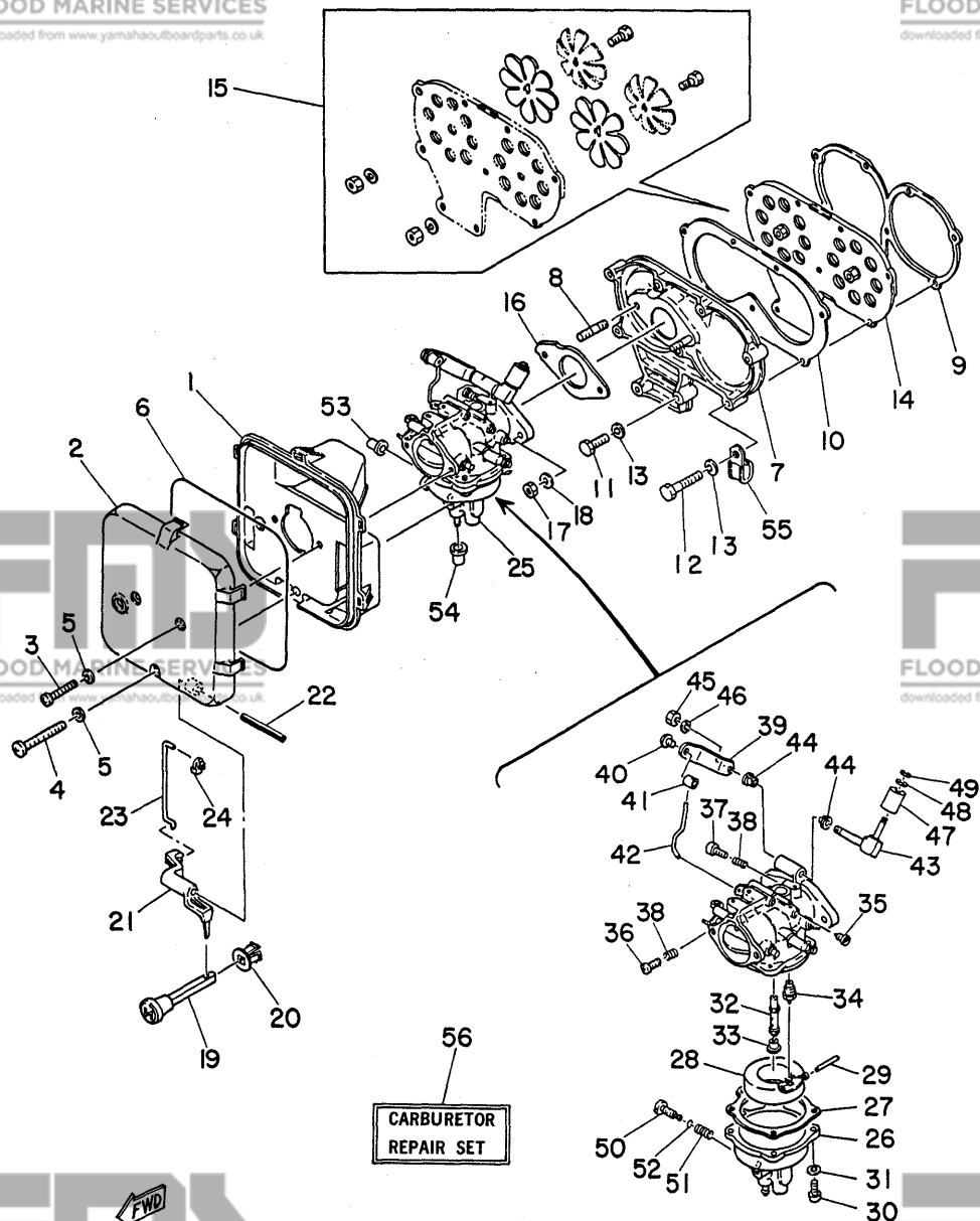
Fig. 5 INTAKE '80/'81
