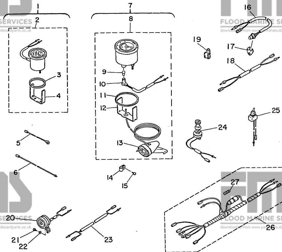
Fig. 22 ACCESSORY PARTS 2 -'80/'81
