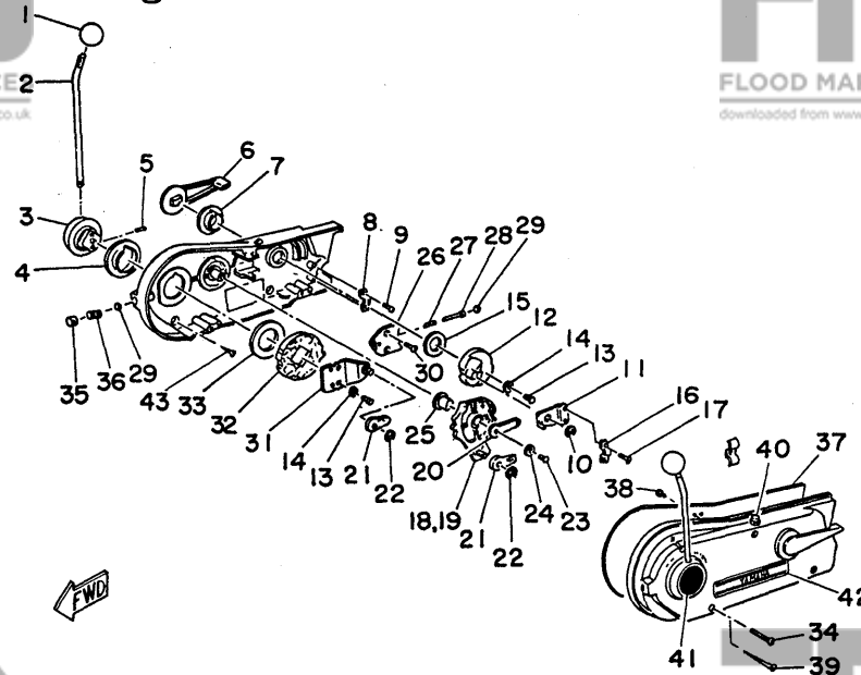
Fig. 19 REMOTE CONTROL ASS'Y -'80/'81
