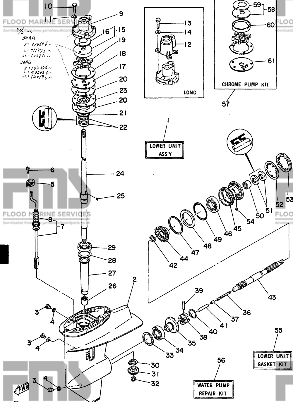
Fig. 8 LOWER &amp; DRIVE 2 '80/'81
