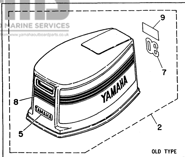
Fig. 2 COWLING -'80/'81
