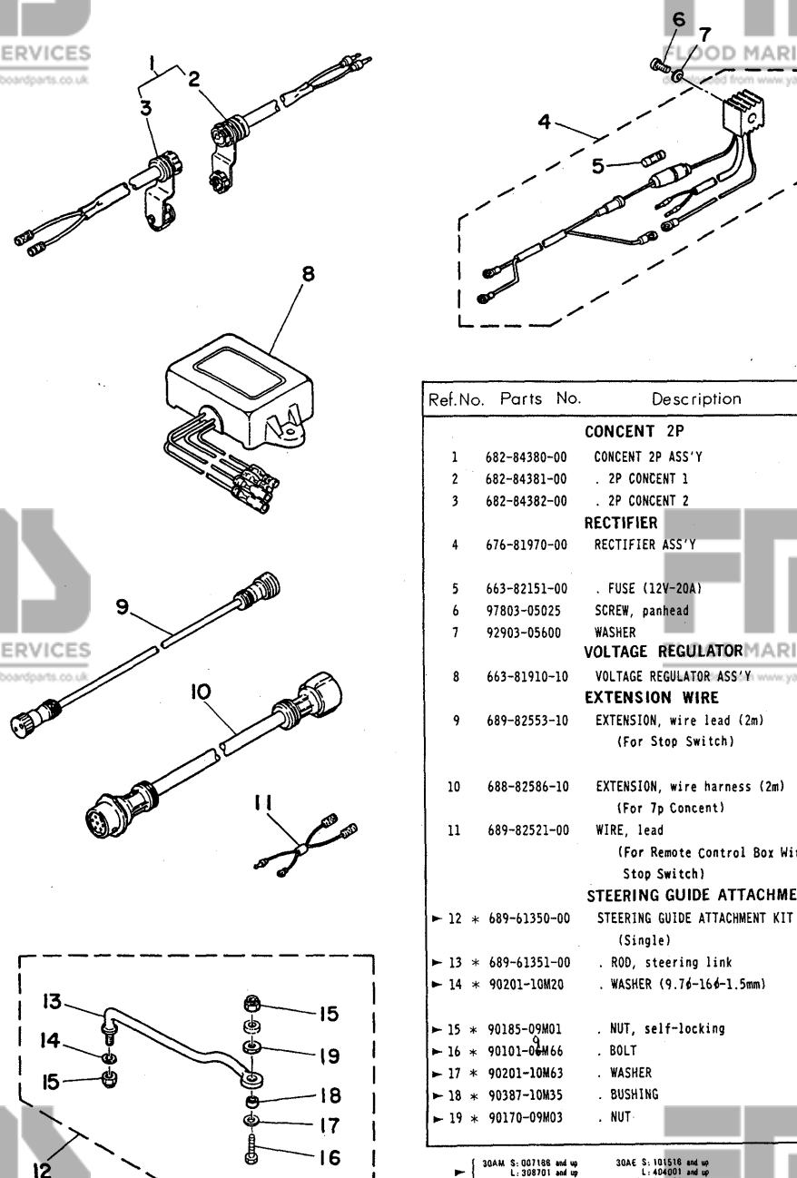
Fig. 17 OPTIONAL PARTS I -'80/'81
