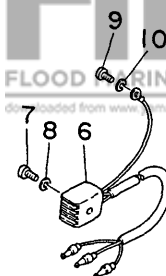
Fig. 15 ELECTRIC PARTS (30AE MODEL) '80/'81
