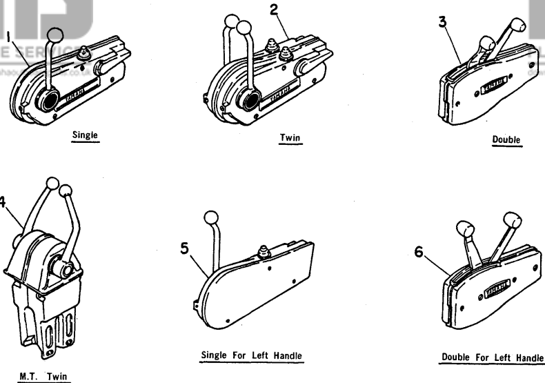
Fig. 20 REMOTE CONTROL '80/'81
