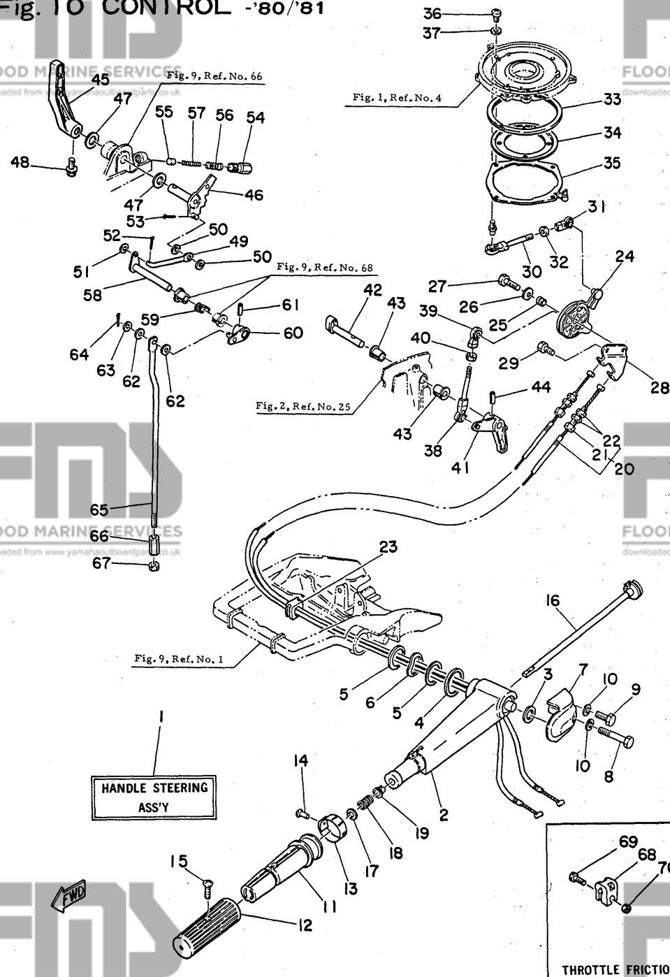
Fig. 10 CONTROL -'80/'81
