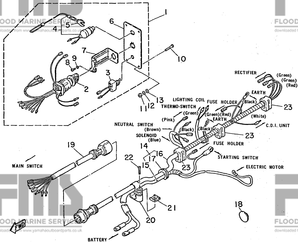
Fig. 16 SWITCH PANEL (30AE MODEL) -'80/'81
