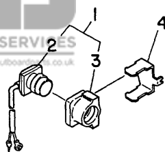
Fig. 15 ELECTRIC PARTS (30AE MODEL) '80/'81
