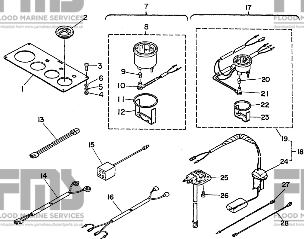
Fig. 21 ACCESSORY PARTS 1 -'80/'81
