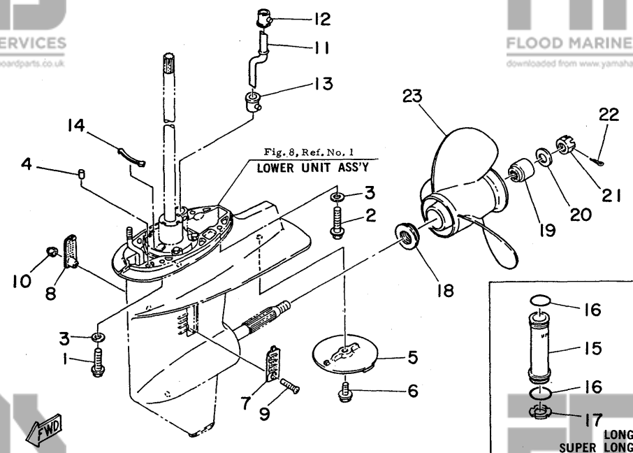
Fig. 7 LOWER &amp; DRIVE 1 -'80/'81
