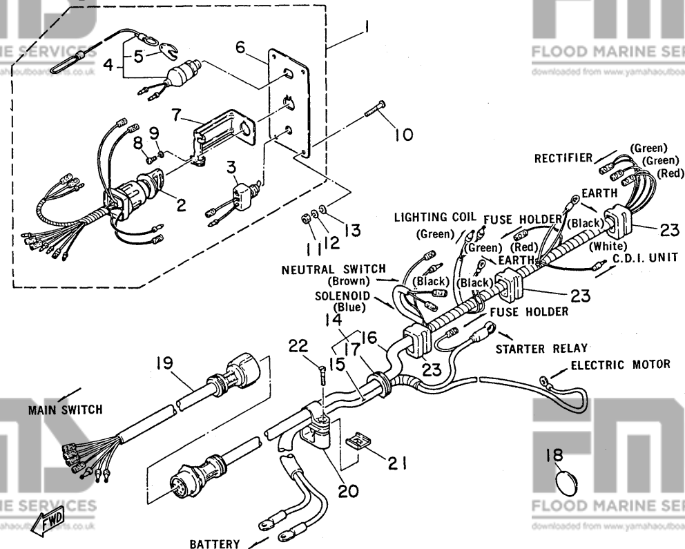
Fig. 18 SWITCH PANEL (25DE MODEL) -'80/'81
