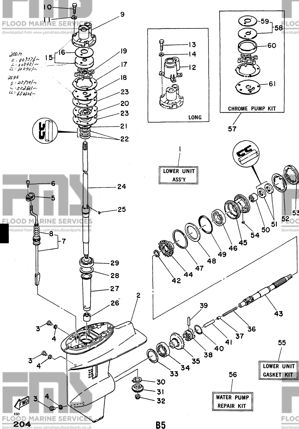
Fig. 11 LOWER &amp; DRIVE 2 -'80/'81
