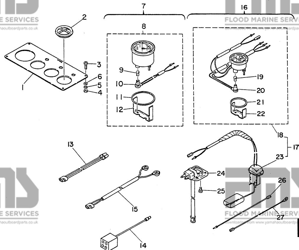
Fig. 23 ACCESSORY PARTS I -'80/'81
