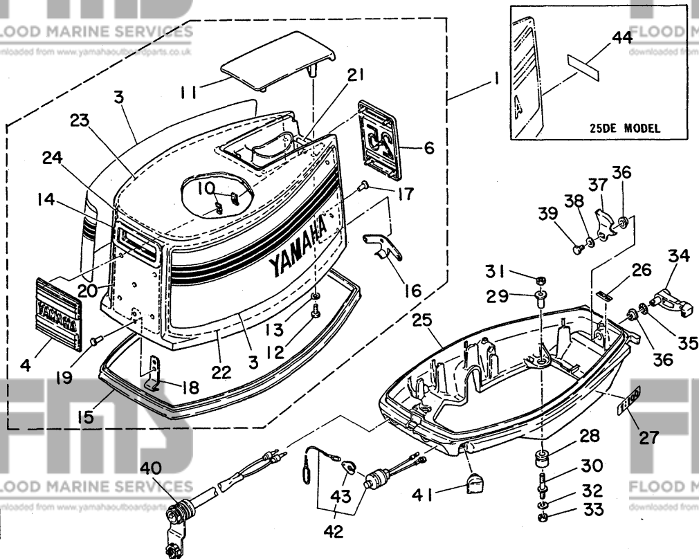
Fig. 2 COWLING '80/'81
