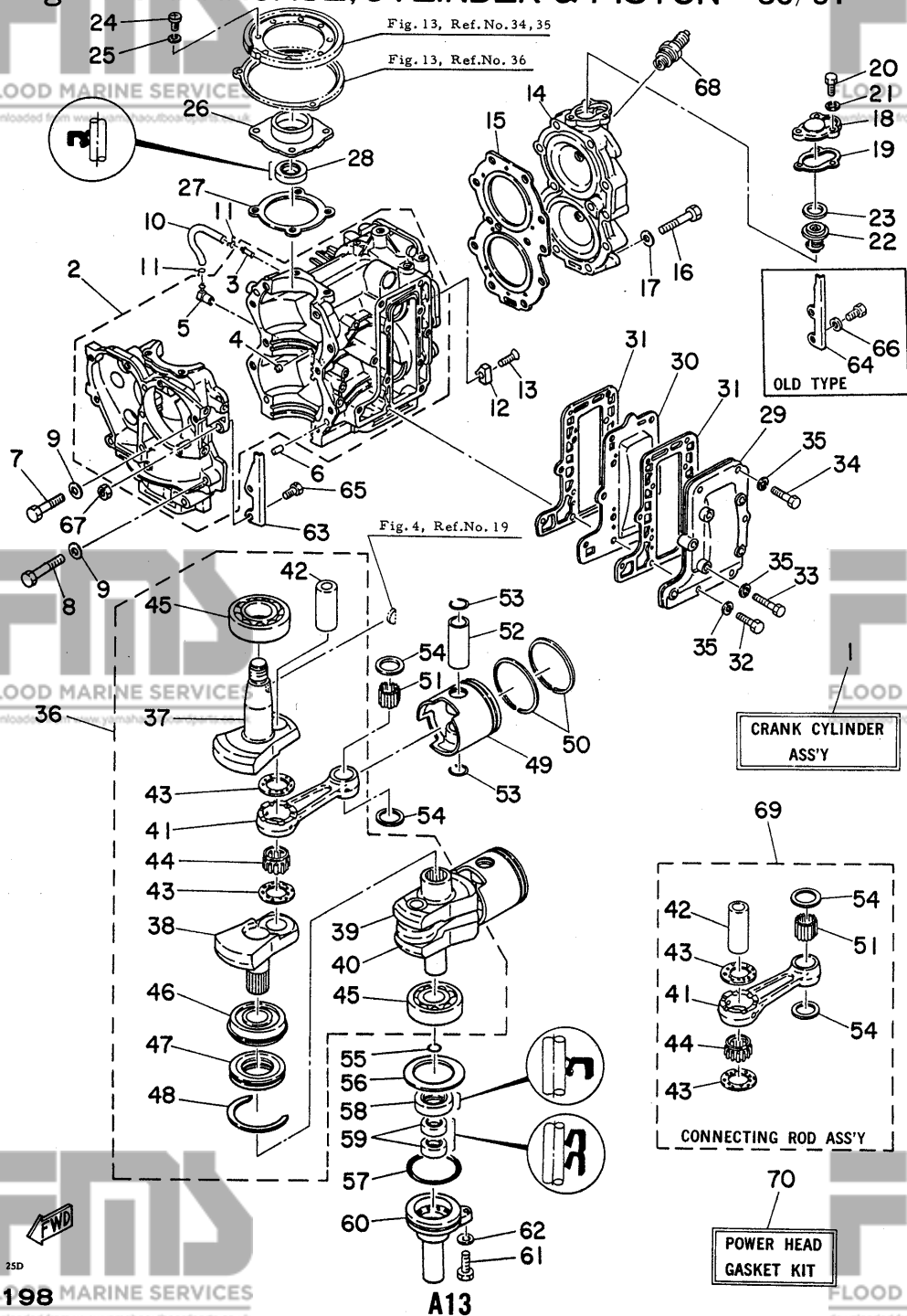
Fig. 8 CRANKCASE, CYLINDER & PISTON '80/'81
