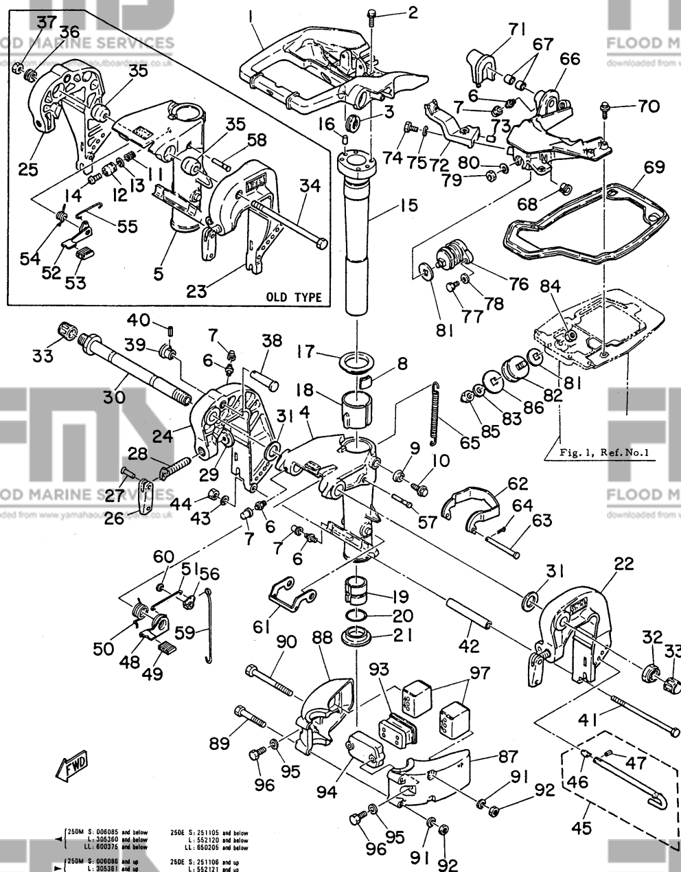
Fig. 12 BRACKET '80/'81
