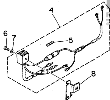
Fig. 19 OPTIONAL PARTS 1 -'80/'81
