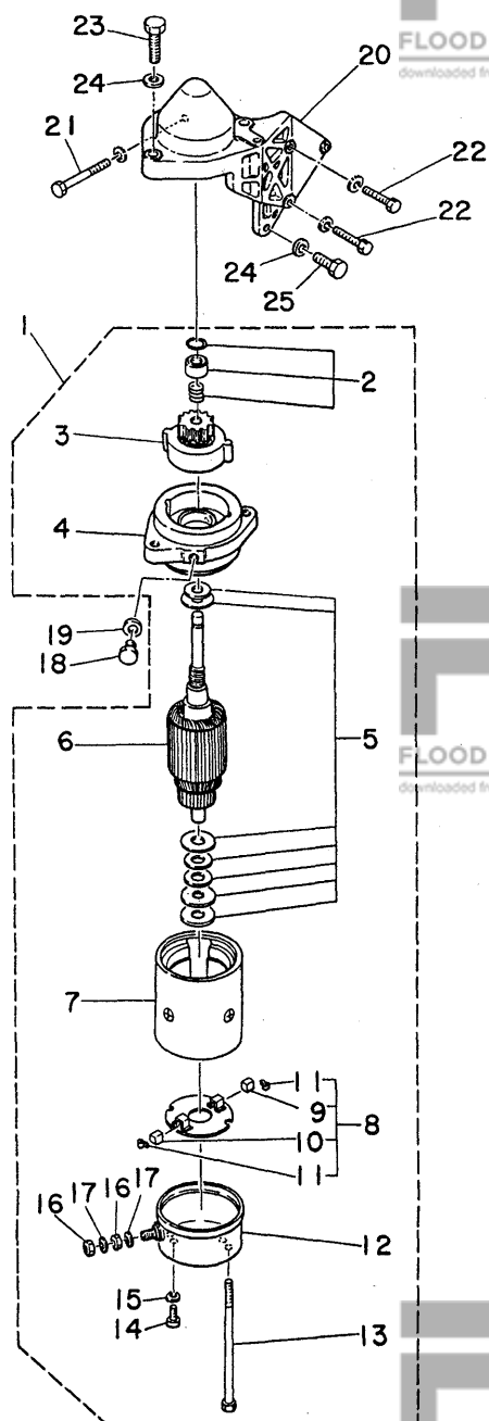
Fig. 15 ELECTRIC MOTOR (25DE MODEL) -'80/'81
