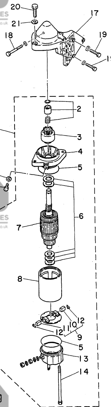
Fig. 16 ELECTRIC MOTOR (25DE MODEL) -'80/'81
