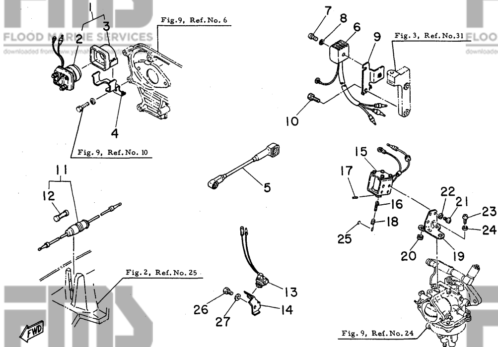
Fig. 17 ELECTRIC PARTS (25DE MODEL) -'80/'81
