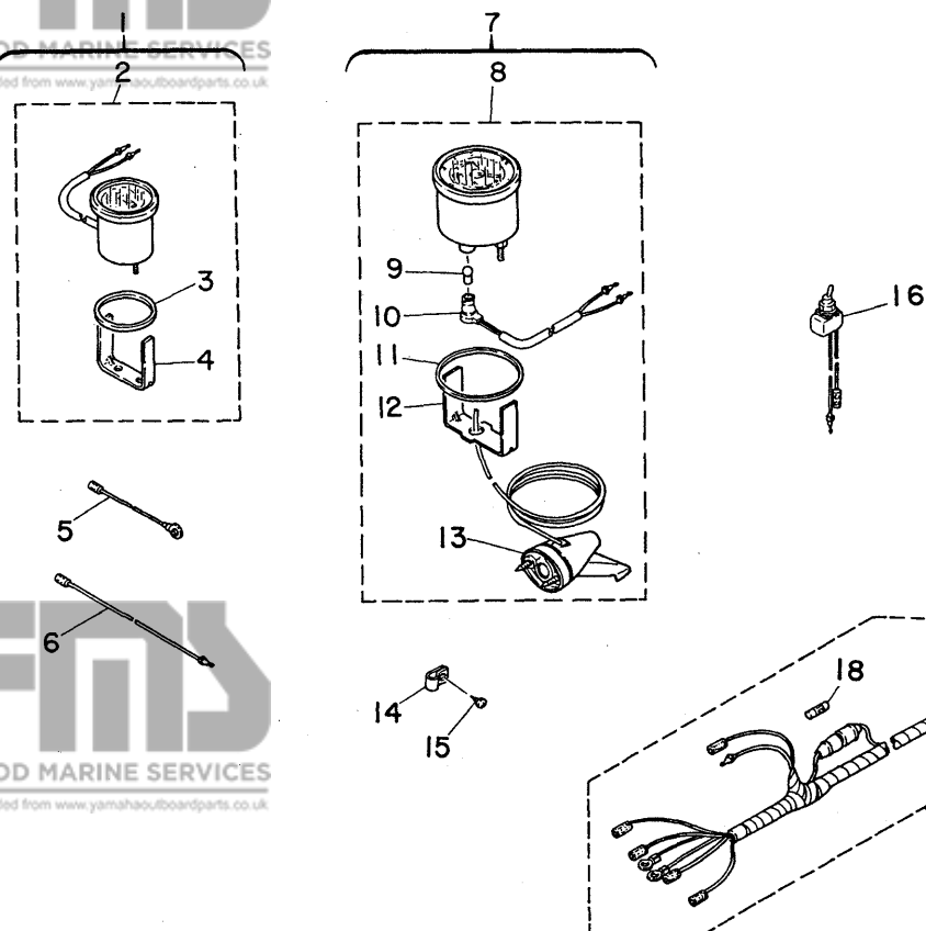
Fig. 24 ACCESSORY PARTS 2 -'80/'81
