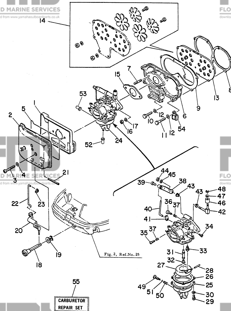
Fig. 9 INTAKE '80/'81
