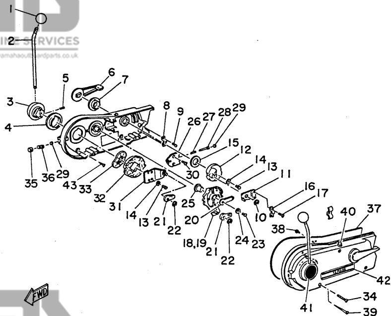
Fig. 22 REMOTE CONTROL ASS'Y -'80/'81
