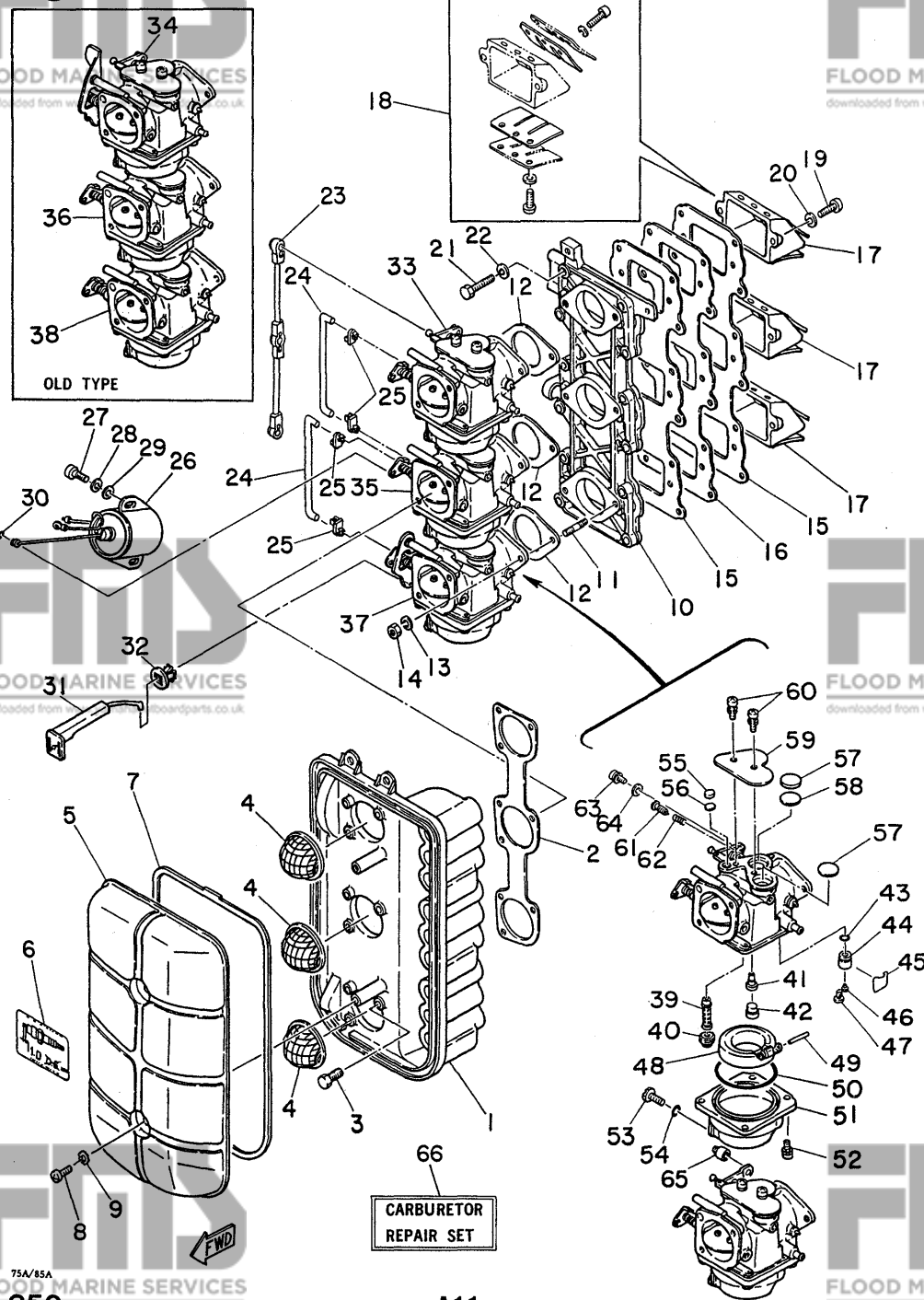
Fig. 6 INTAKE '80/'81
