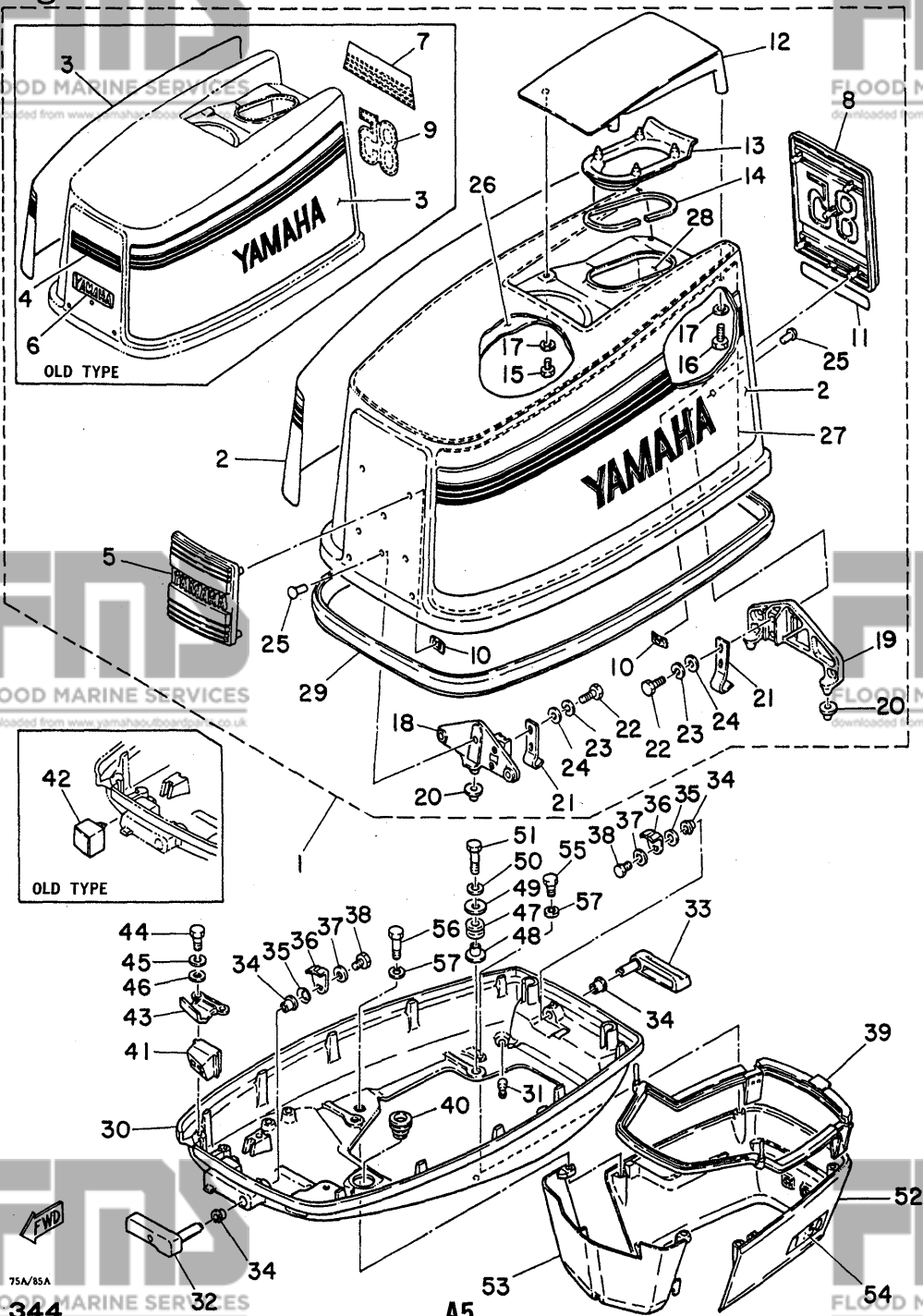
Fig. 2 COWLING-'80/'81
