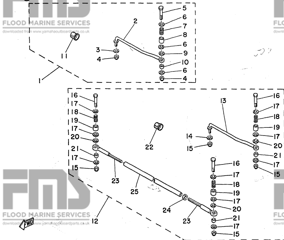
Fig. 19 STEERING GUIDE ATTACHMENT '80/'81
