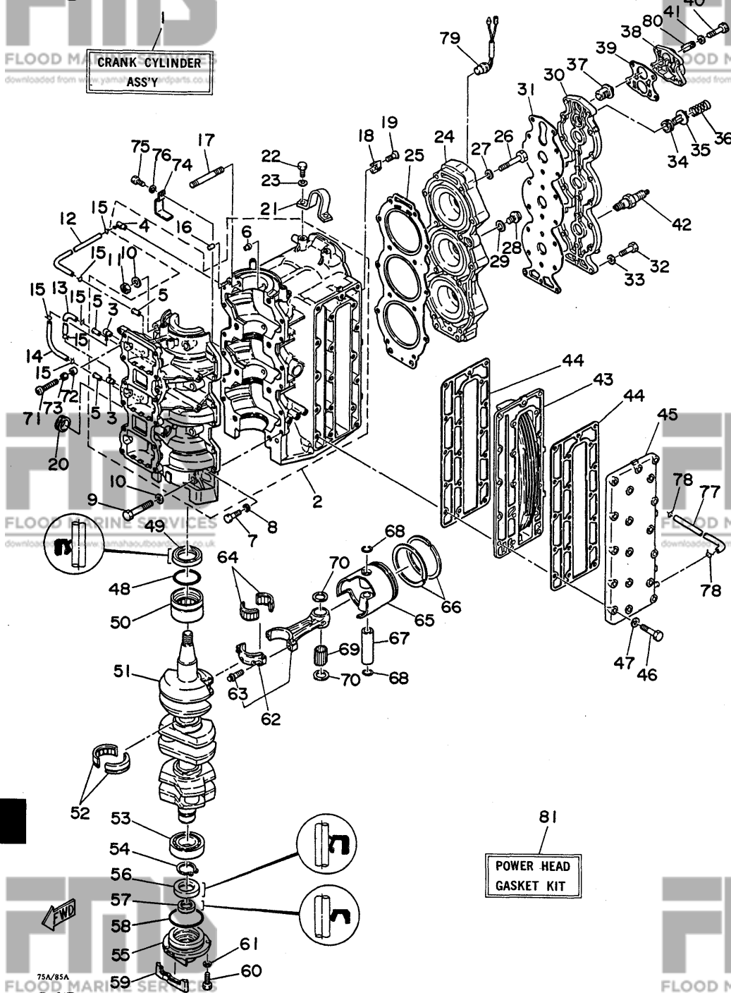
Fig. 5 CRANKCASE, CYLINDER &amp; PISTON '80/'81
