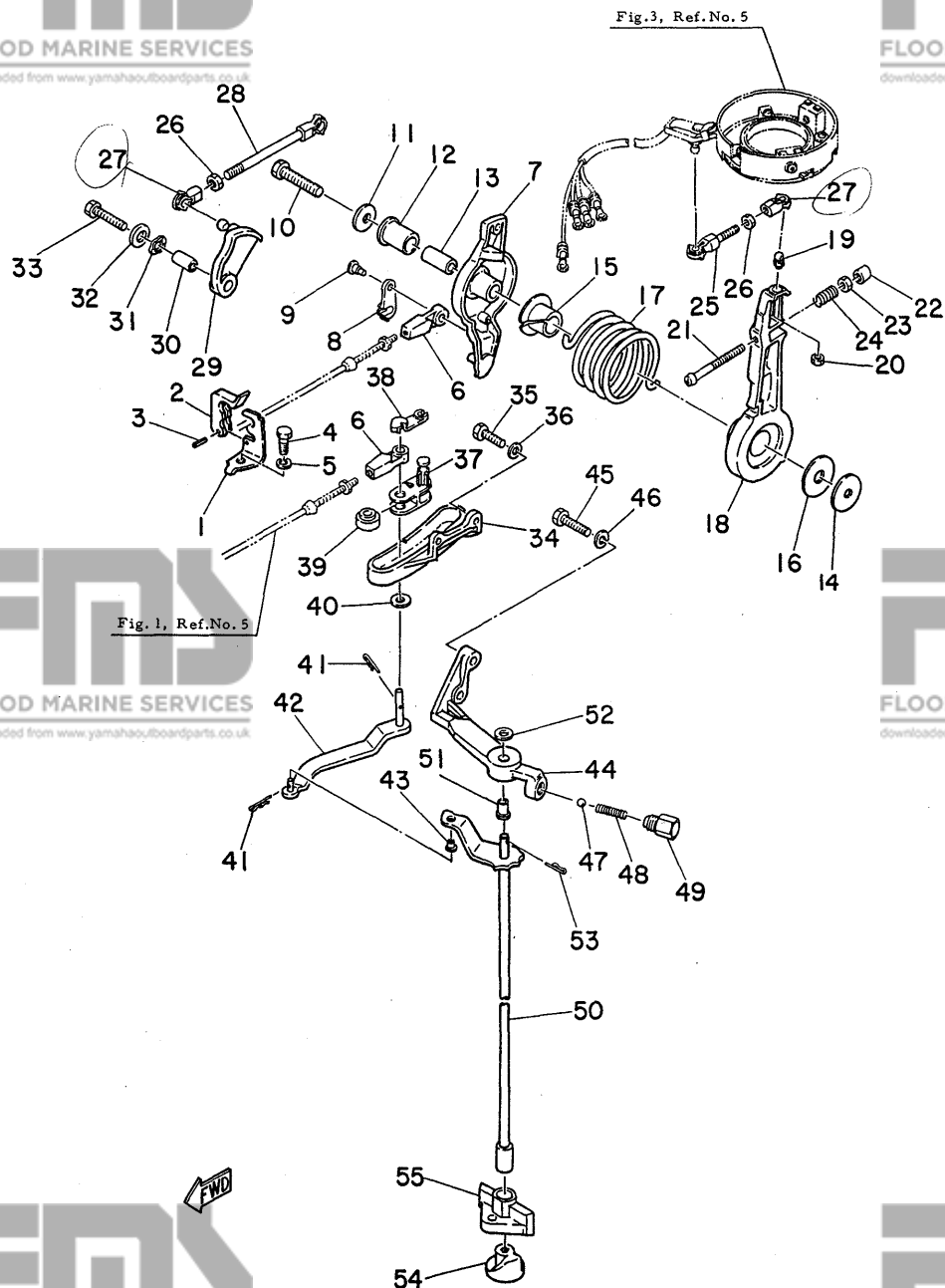
Fig. 7 CONTROL -'80/'81
