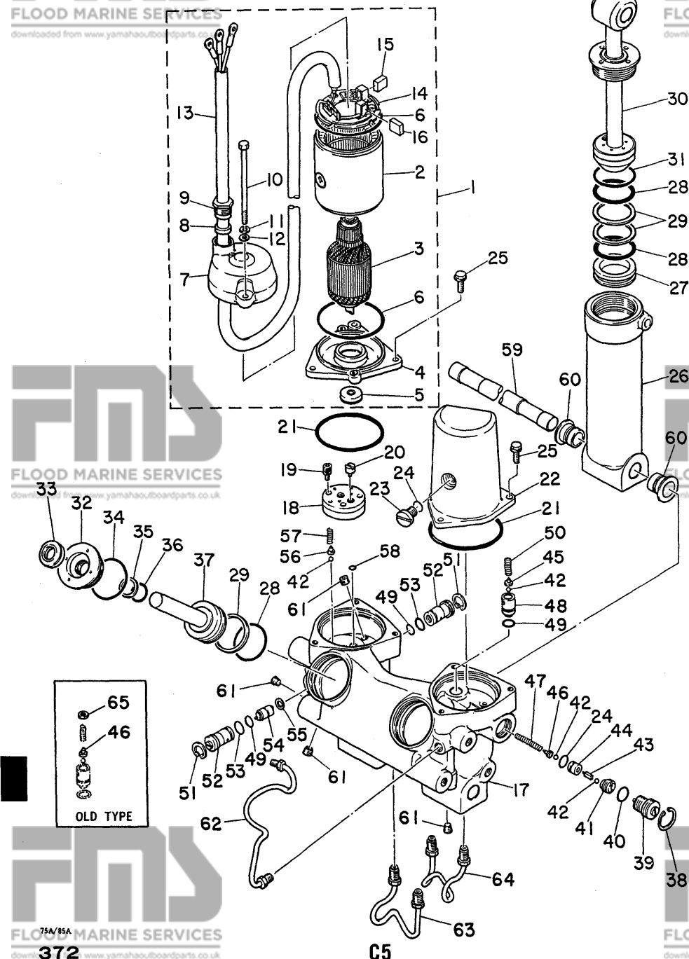
Fig. 17 POWER TRIM & TILT 2 (85AET / 75AET MODEL) - '80 / '81
