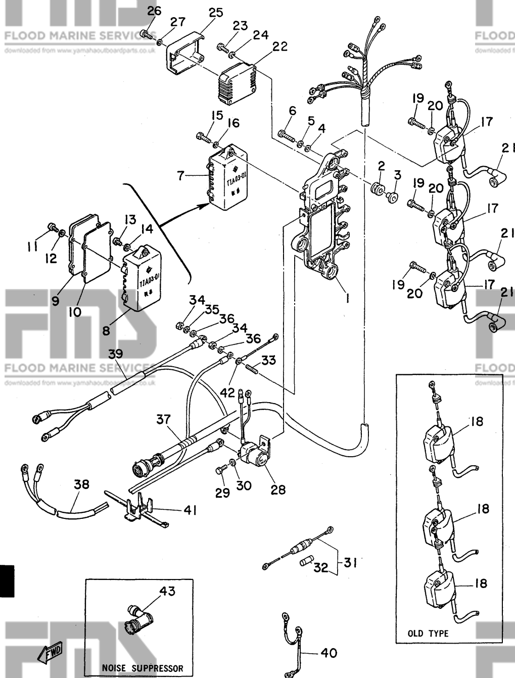
Fig. 10 ELECTRIC PARTS -'80/'81
