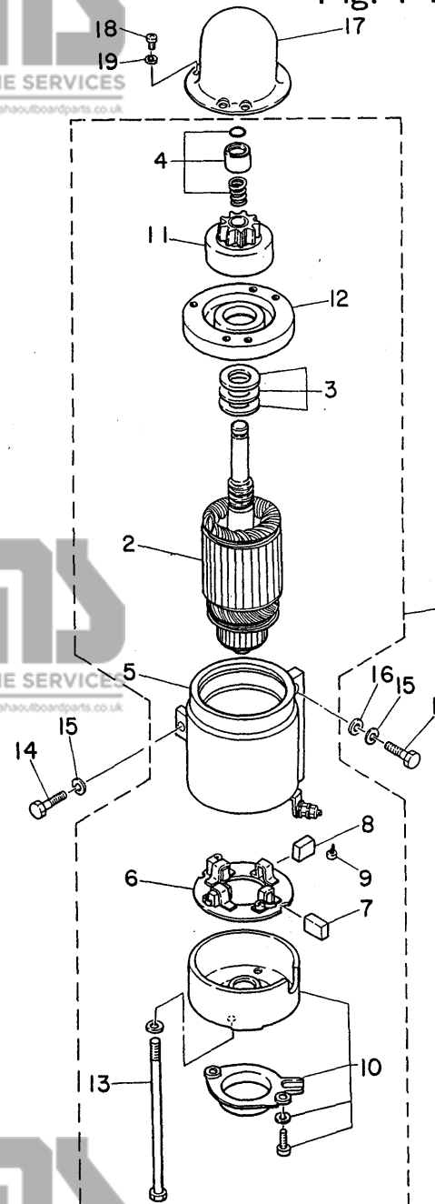
Fig. 4 ELECTRIC STARTER '80/'81
