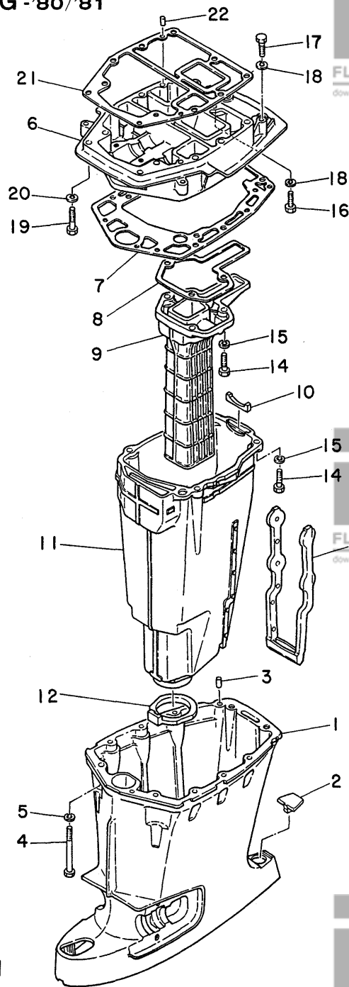
Fig. 11 UPPER CASING -'80/'81
