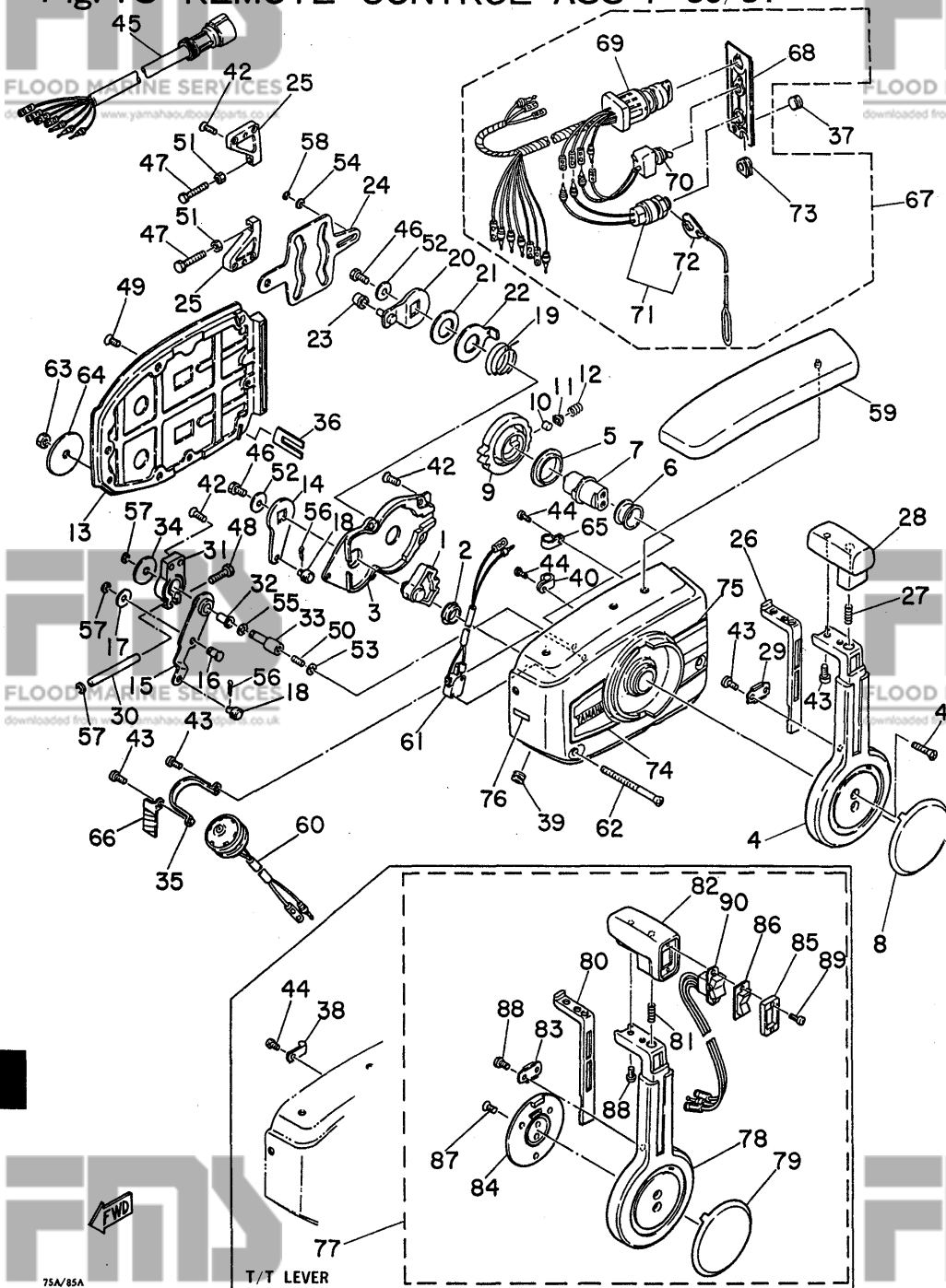
Fig. 15 REMOTE CONTROL ASS'Y -'80/'81
