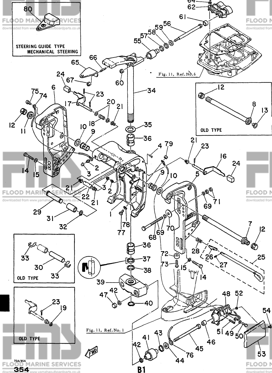
Fig. 8 BRACKET I -'80/'81
