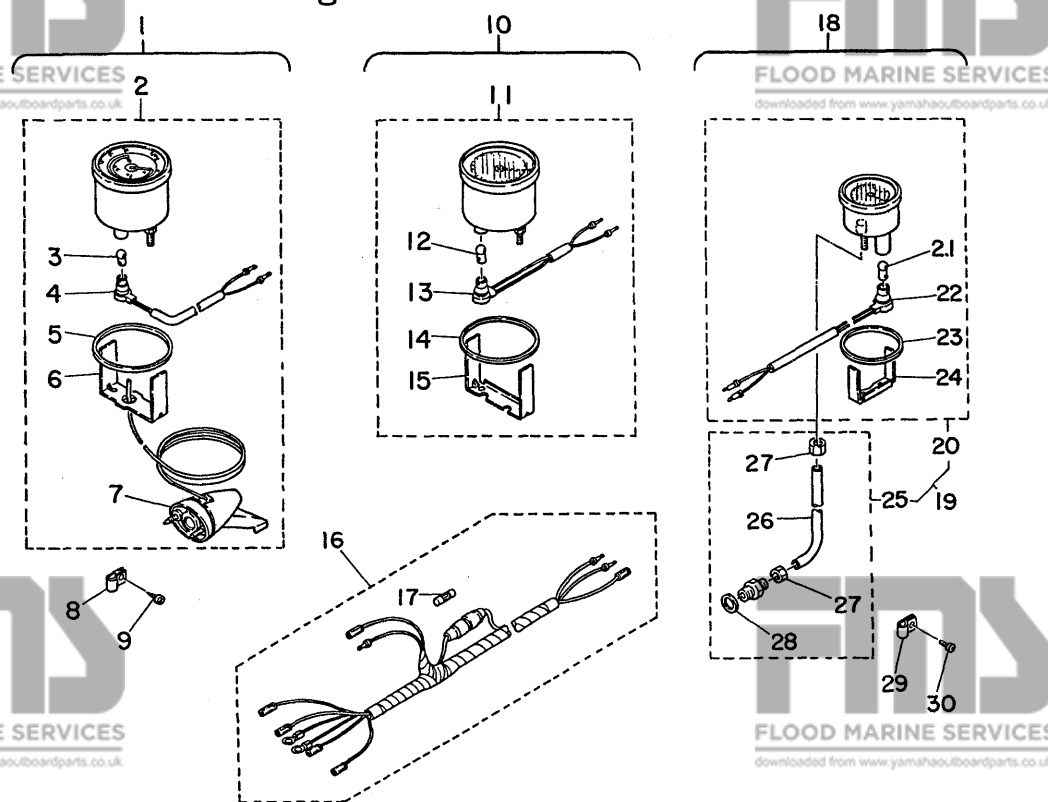
Fig. 20 ACCESSORY PARTS 1-'80/'81
