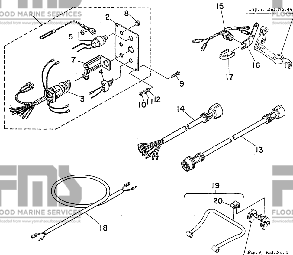
Fig. 23 ACCESSORY PARTS 4-'80/'81
