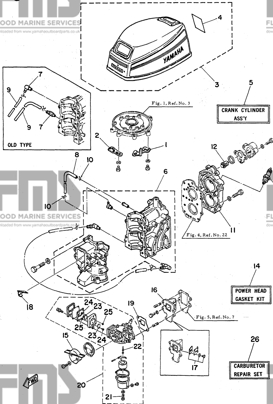
Fig. 15 OPTIONAL PARTS 2 (6B MODEL) '80/'81
