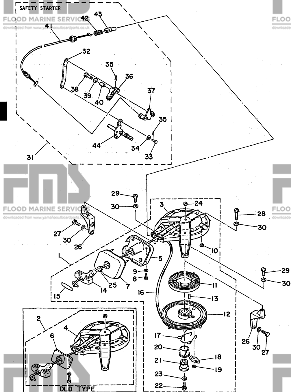
Fig. 3 STARTER '80/'81
