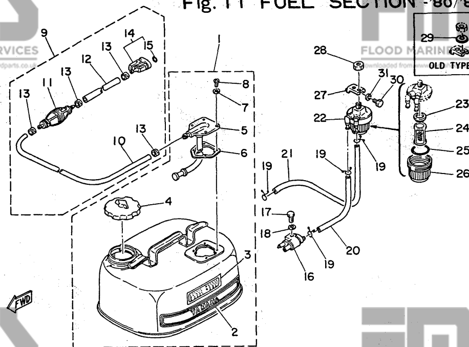
Fig. 11 FUEL SECTION -'80/'81
