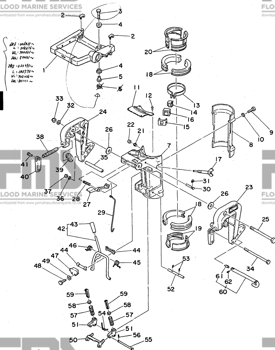
Fig. 6 BRACKET '80/'81
