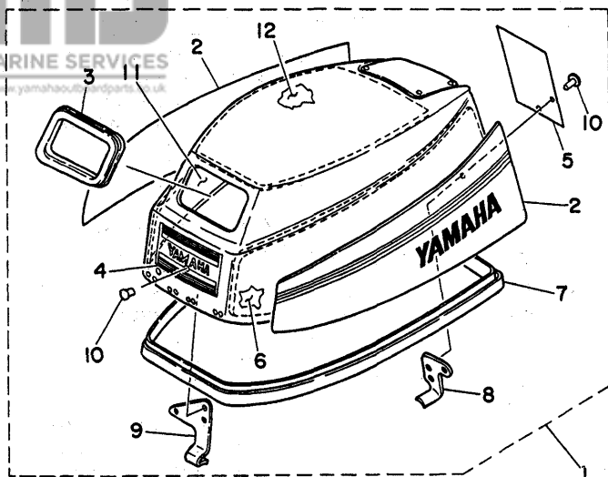
Fig. 2 COWLING '80/'81
