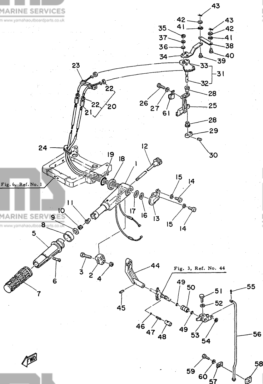
Fig. 7 CONTROL -'80/'81
