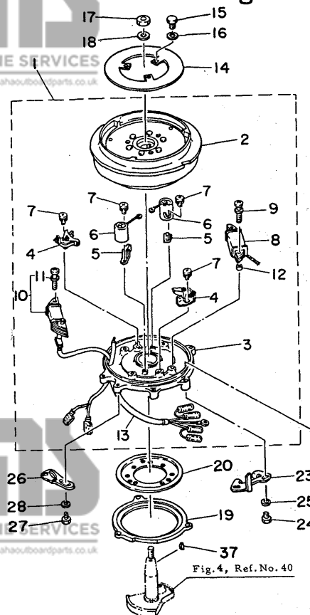
Fig. 1 FLYWHEEL MAGNETO '80/'81
