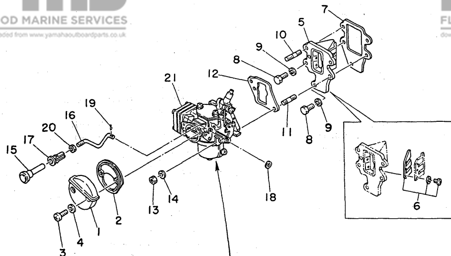
Fig. 5 INTAKE '80/'81
