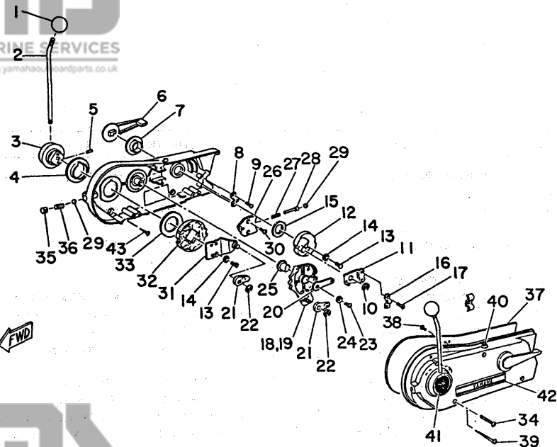
Fig. 13 REMOTE CONTROL ASS'Y '80/'81
