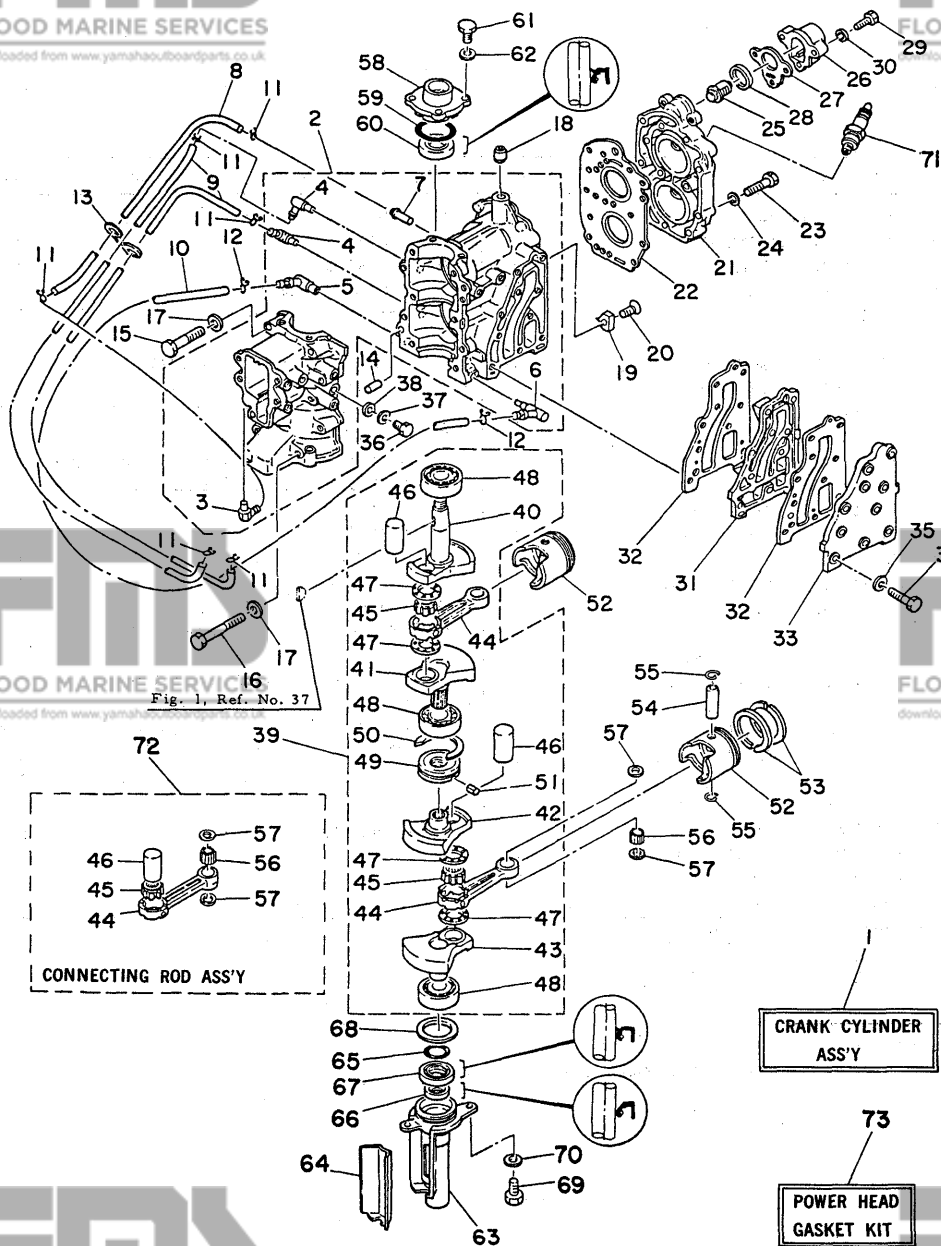
Fig. 4 CRANKCASE, CYLINDER & PISTON '80/'81
