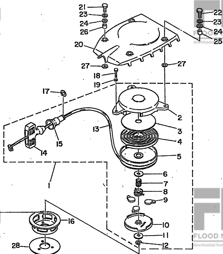
Fig. 1 STARTER-1979
