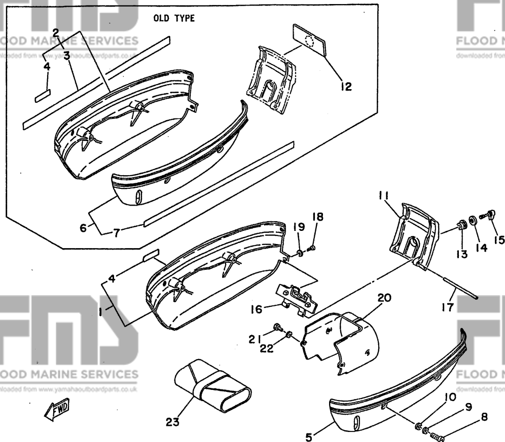
Fig. 3 COWLING-1979
