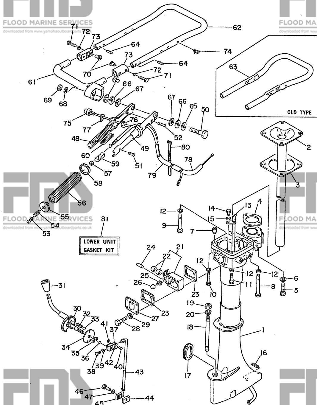
Fig. 7 UPPER CASING &amp; STEERING-1979
