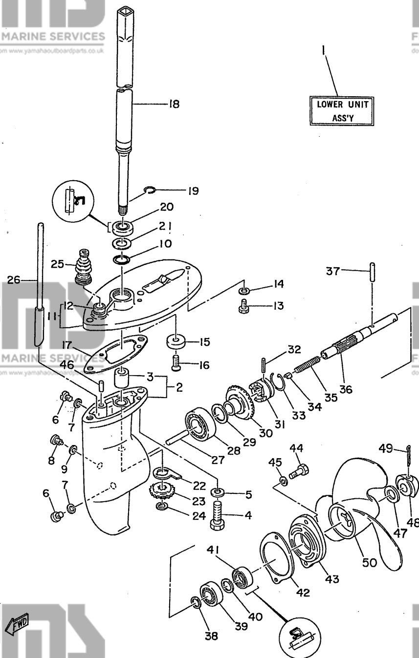
Fig. 8 LOWER &amp; DRIVE-1979
