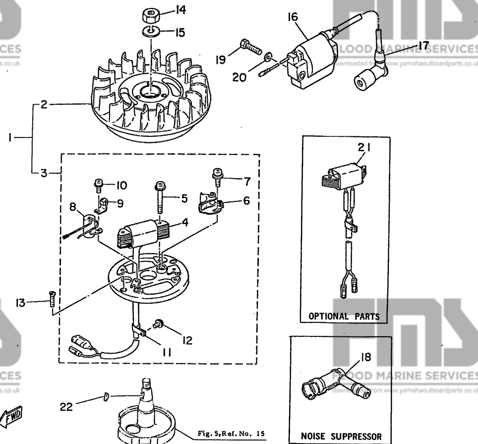
Fig. 2 FLYWHEEL MAGNETO-1979
