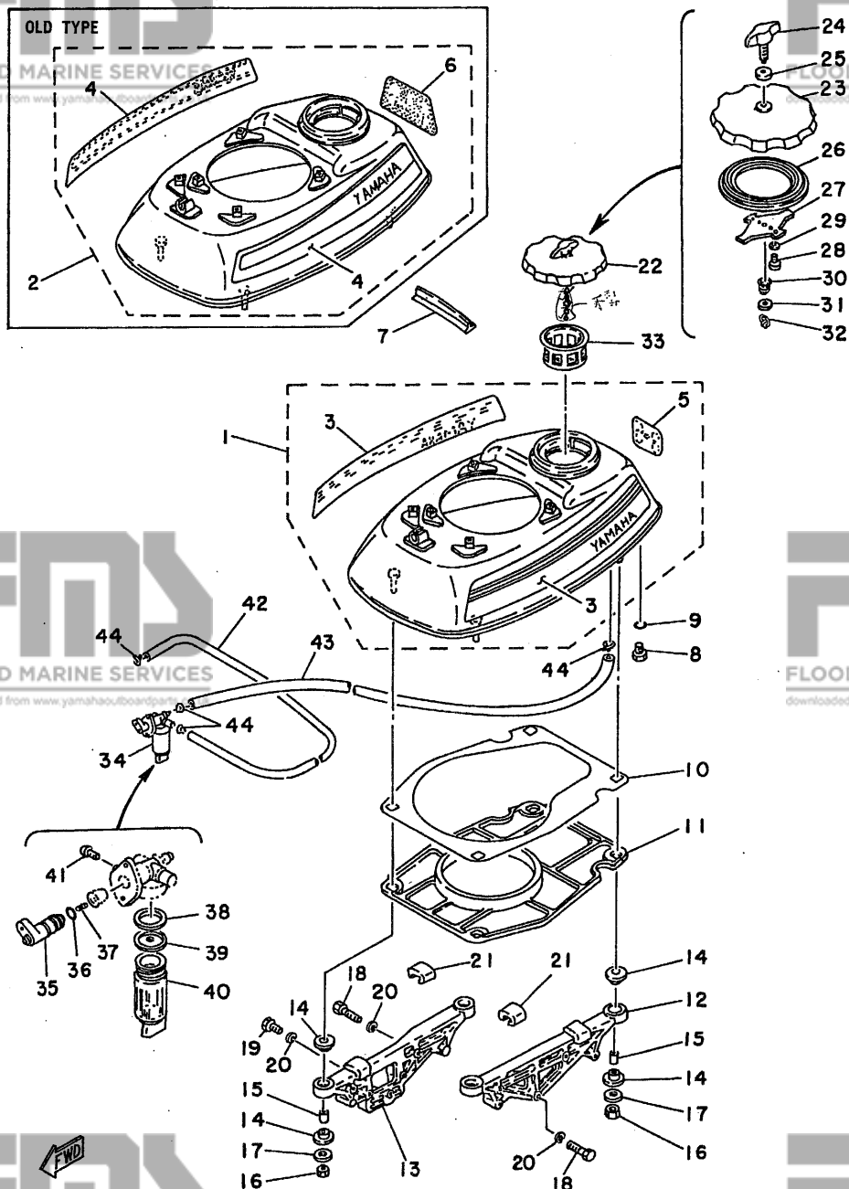
Fig. 4 FUEL SECTION -1979
