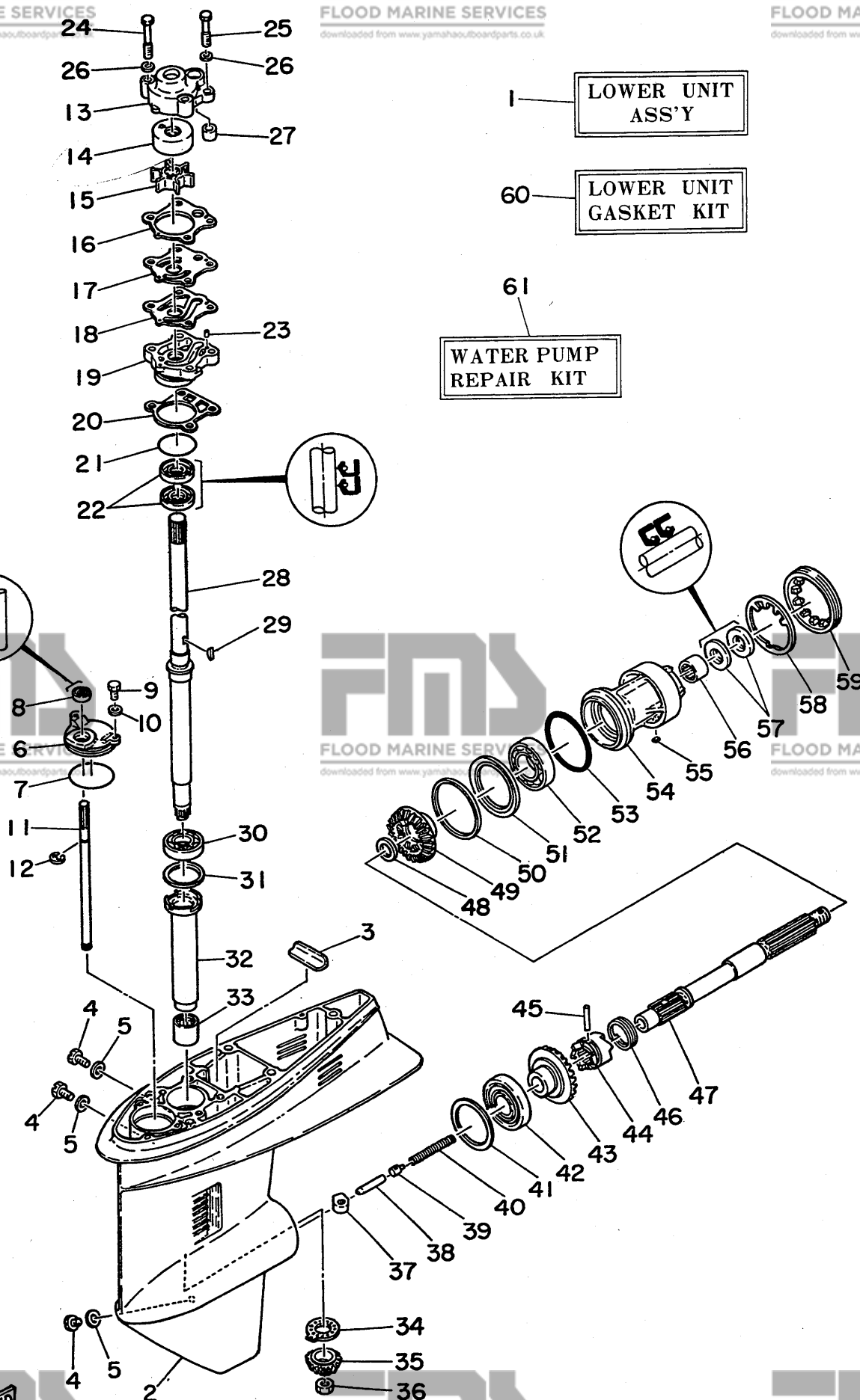
Fig. 1 LOWER & DRIVE 2-1978
