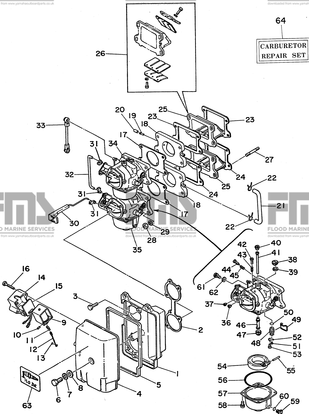
Fig. 5 INTAKE -1978
