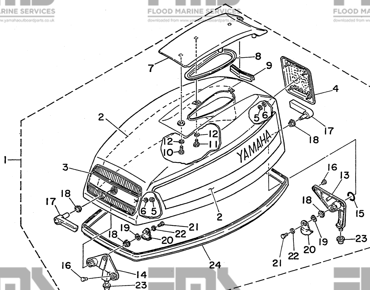
Fig. 2 COWLING - 1978
