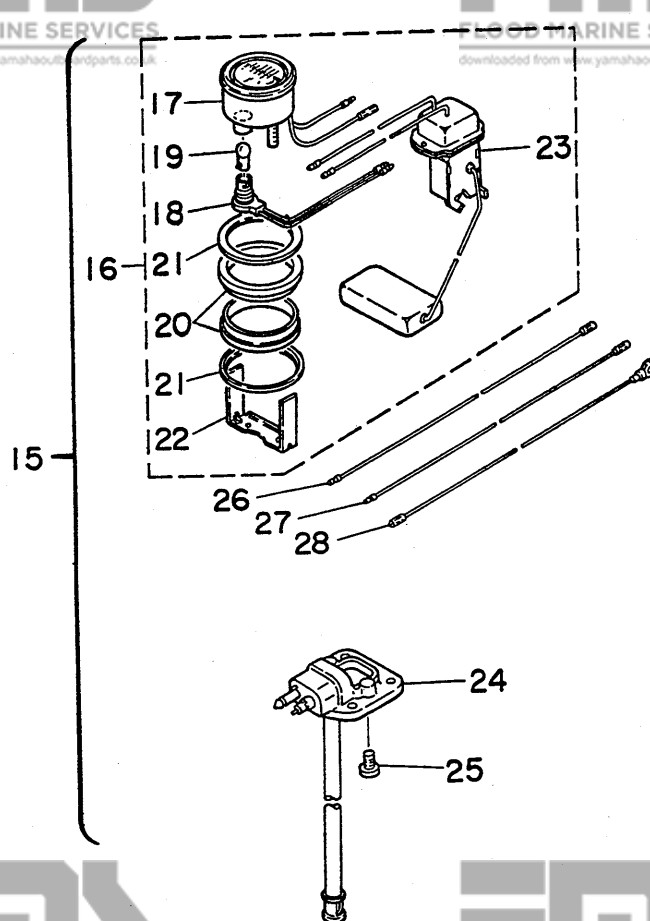
Fig. 15 ACCESSORY PARTS 2-1978
