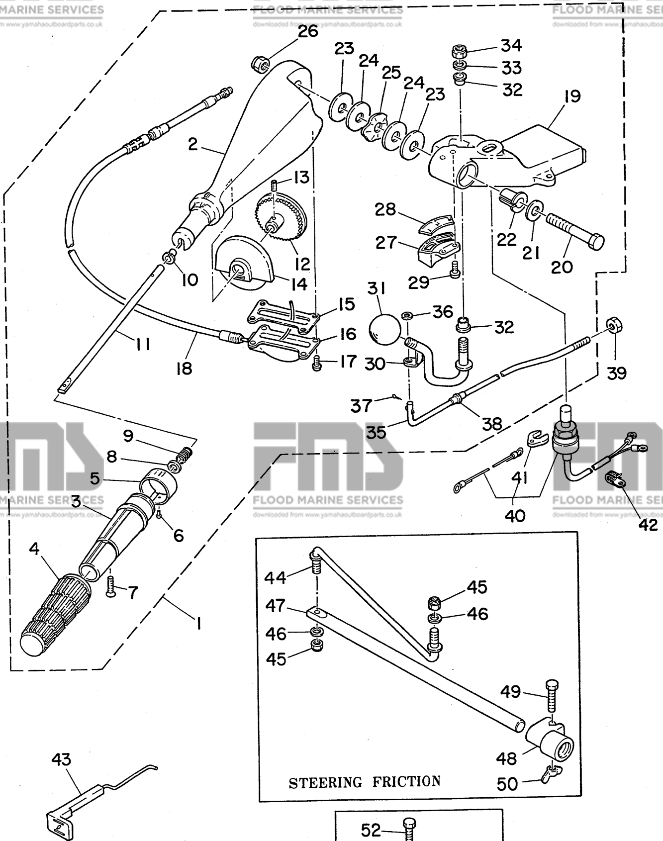
Fig. 17 MANUAL STEERING (55AM MODEL) - 1978
