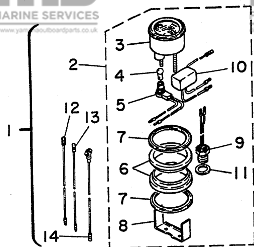
Fig. 15 ACCESSORY PARTS 2-1978
