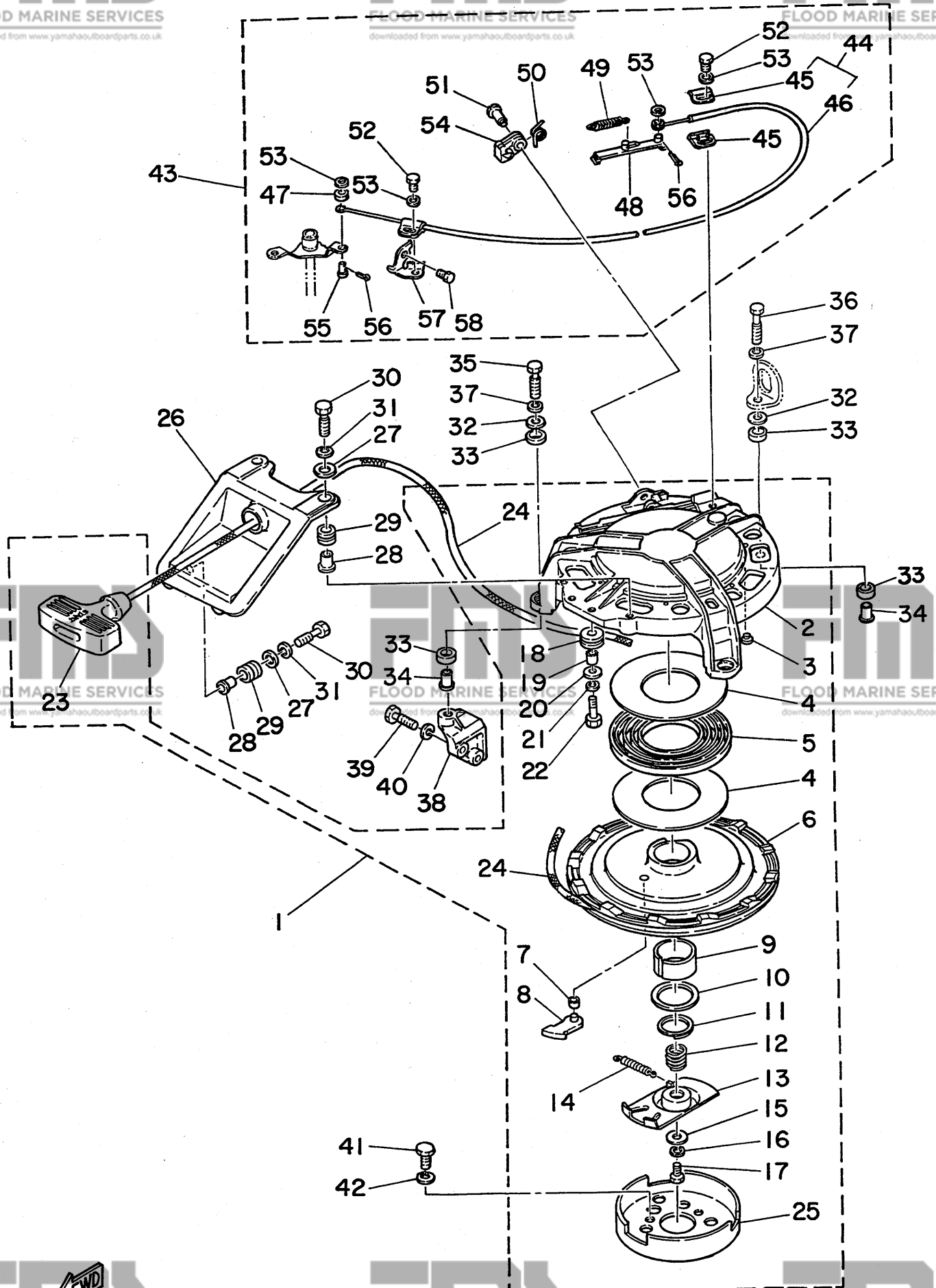
Fig. 1 8 MANUAL STARTER 1 (55AM MODEL) -1978
