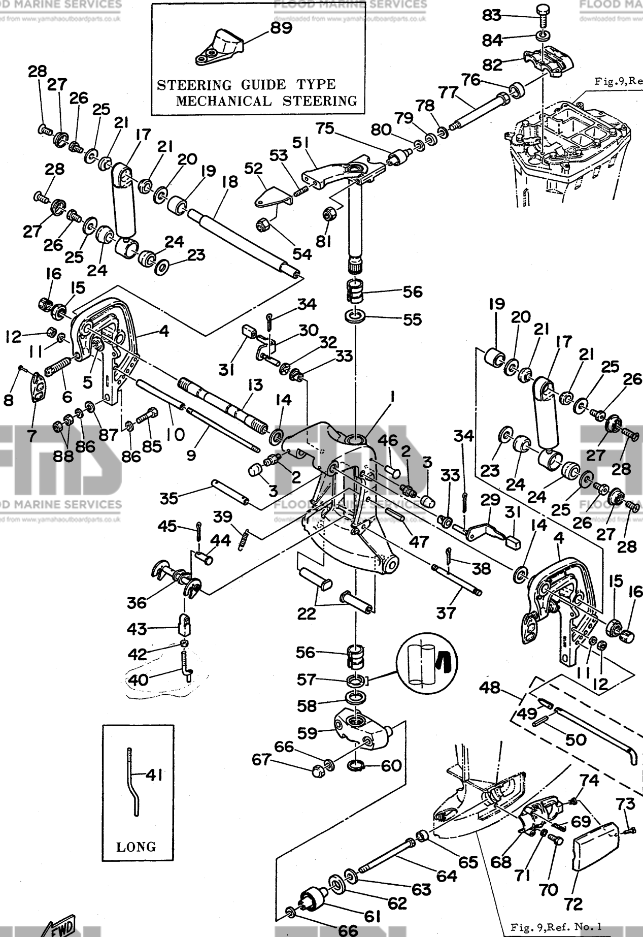
Fig. 8 BRACKET -1978
