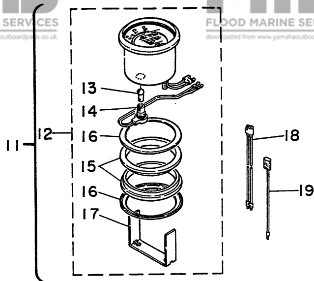
Fig. 14 ACCESSORY PARTS I-1978
