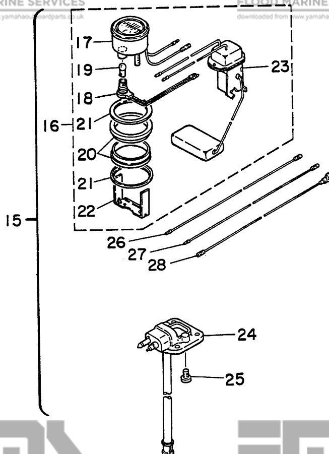
Fig. 15 ACCESSORY PARTS 2-1978
