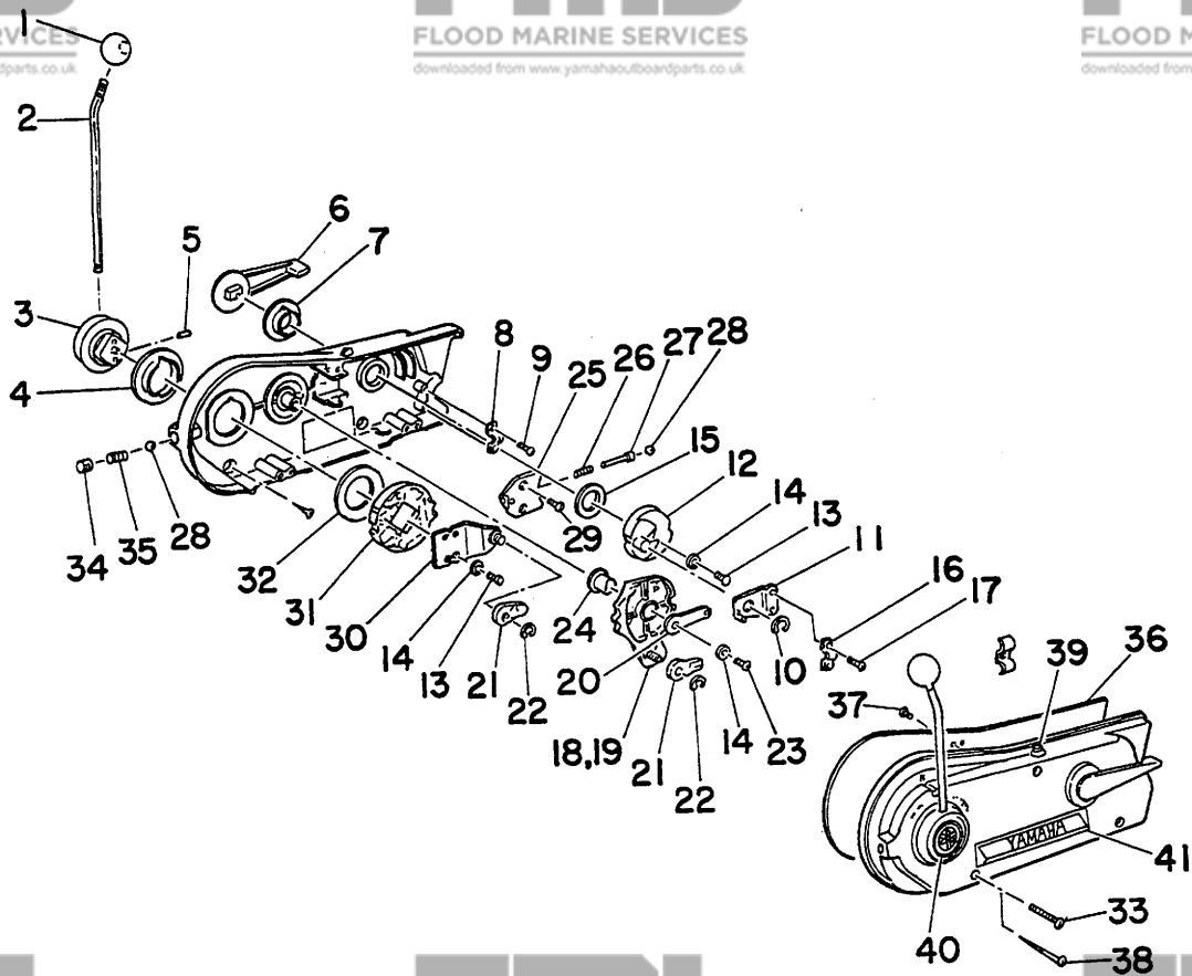
Fig. 21 REMOTE CONTROL ASS'Y - 1978
