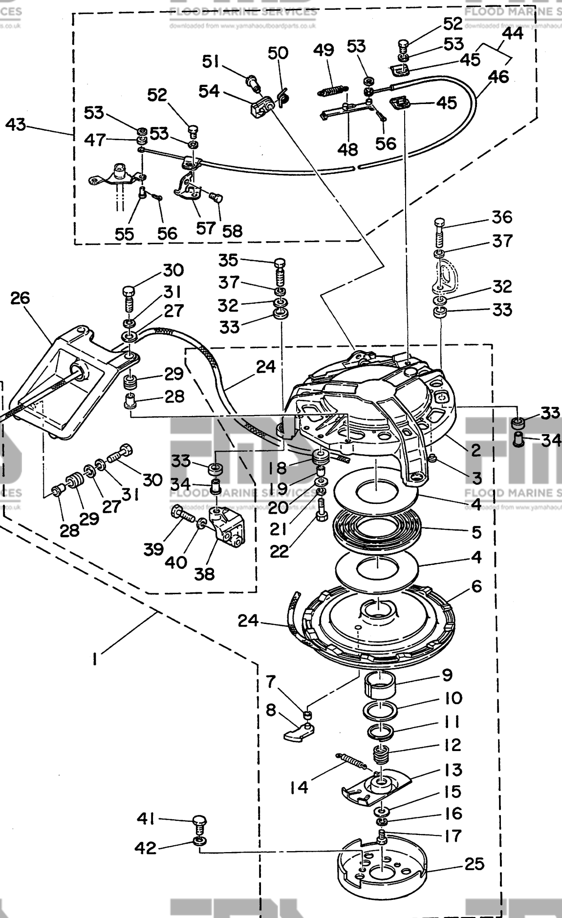
Fig. 1 8 MANUAL STARTER 1 (55AM MODEL) -1978
