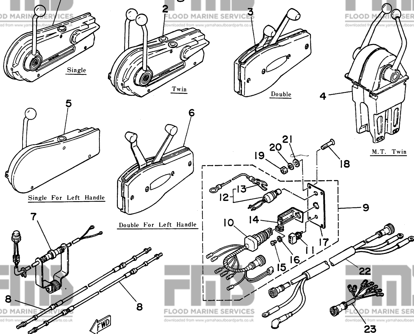
Fig. 1 REMOTE CONTROL - 1978
