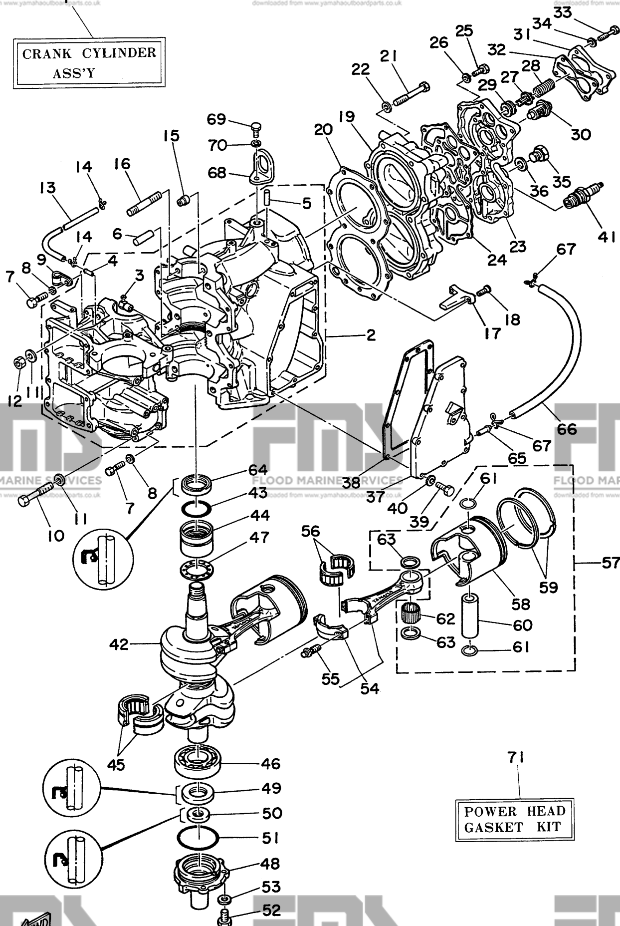
Fig. 6 CRANKCASE, CYLINDER & PISTON -1978
