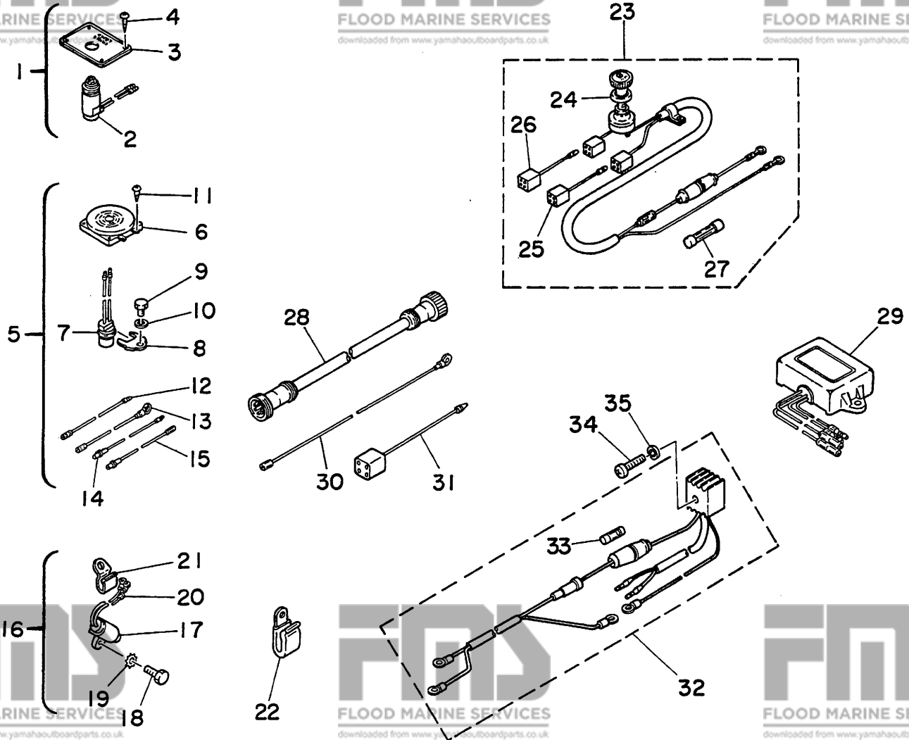
Fig. 16 ACCESSORY PARTS 3-1978
