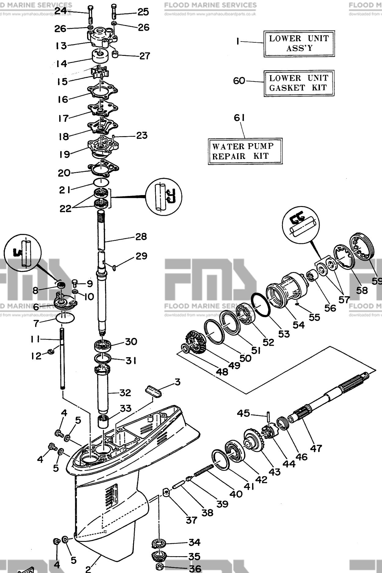
Fig. 1 I LOWER & DRIVE 2-1978
