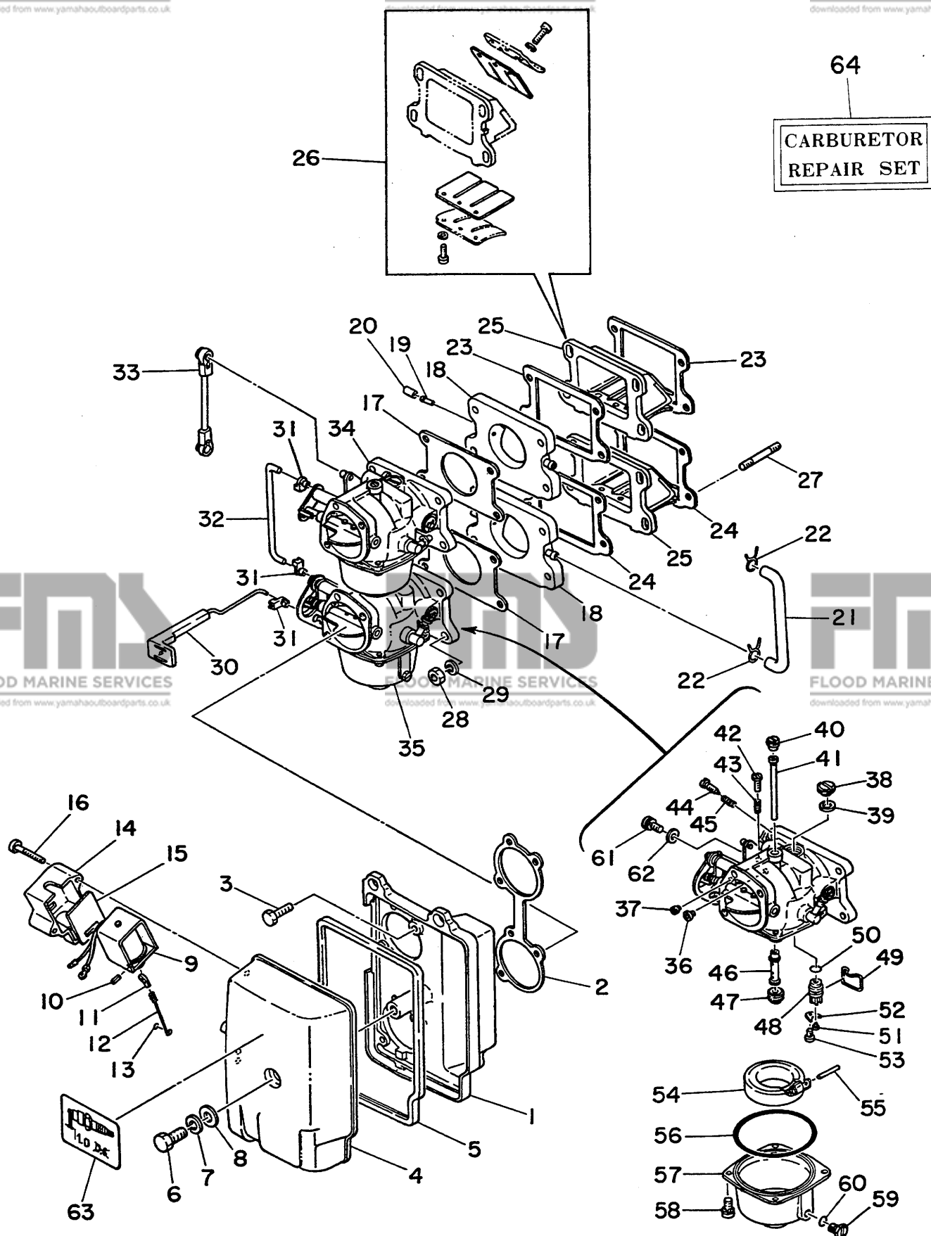
Fig. 5 INTAKE -1978
