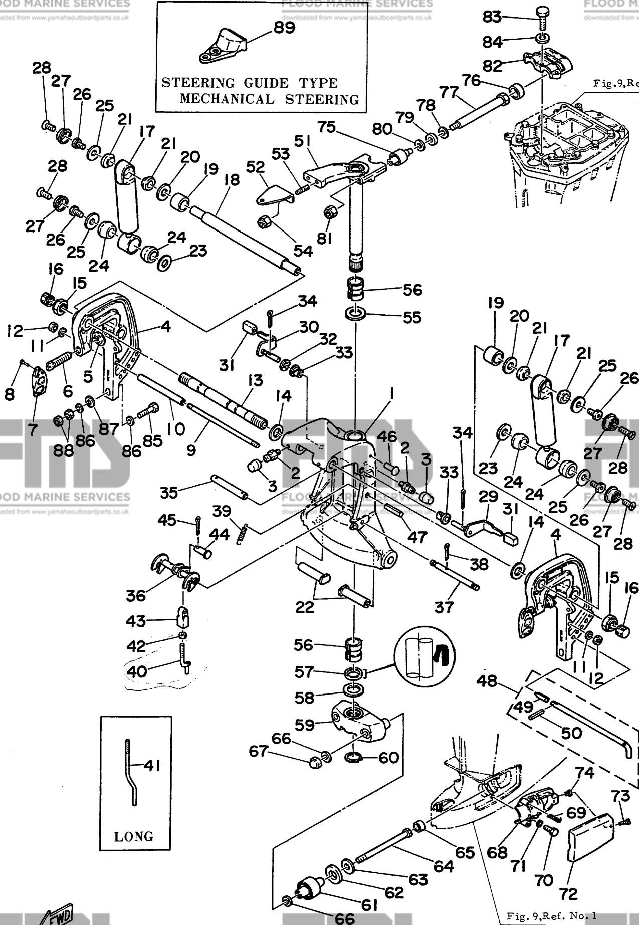
Fig. 8 BRACKET -1978
