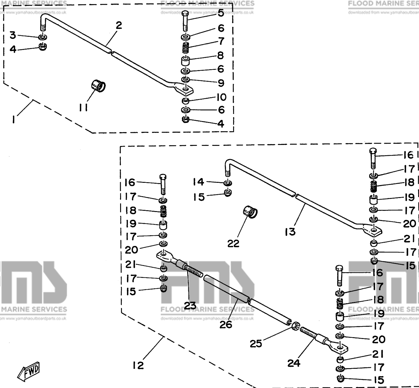
Fig. 20 STEERING GUIDE ATTACHMENT -1978
