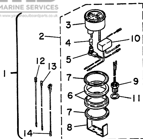
Fig. 15 ACCESSORY PARTS 2-1978
