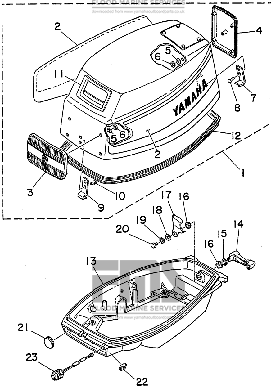
Fig. 1 COWLING-1978
