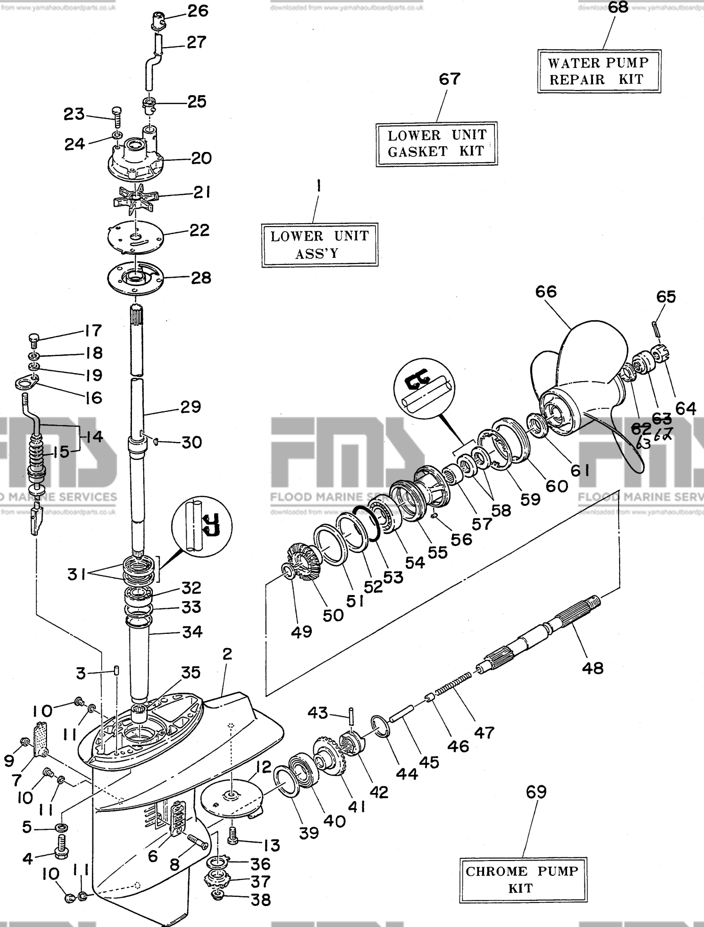
Fig. 7 LOWER & DRIVE - 1978
