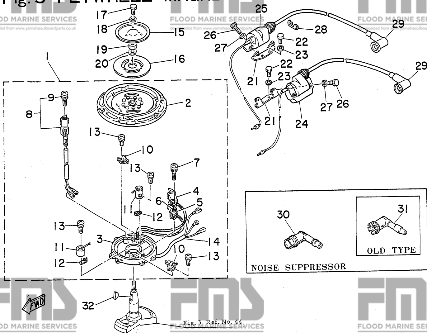
Fig. 5 FLYWHEEL MAGNETO-1978
