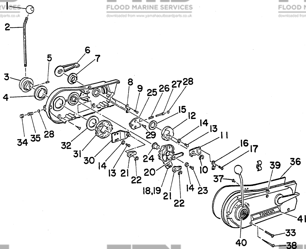
Fig. 17 REMOTE CONTROL ASS'Y - 1978
